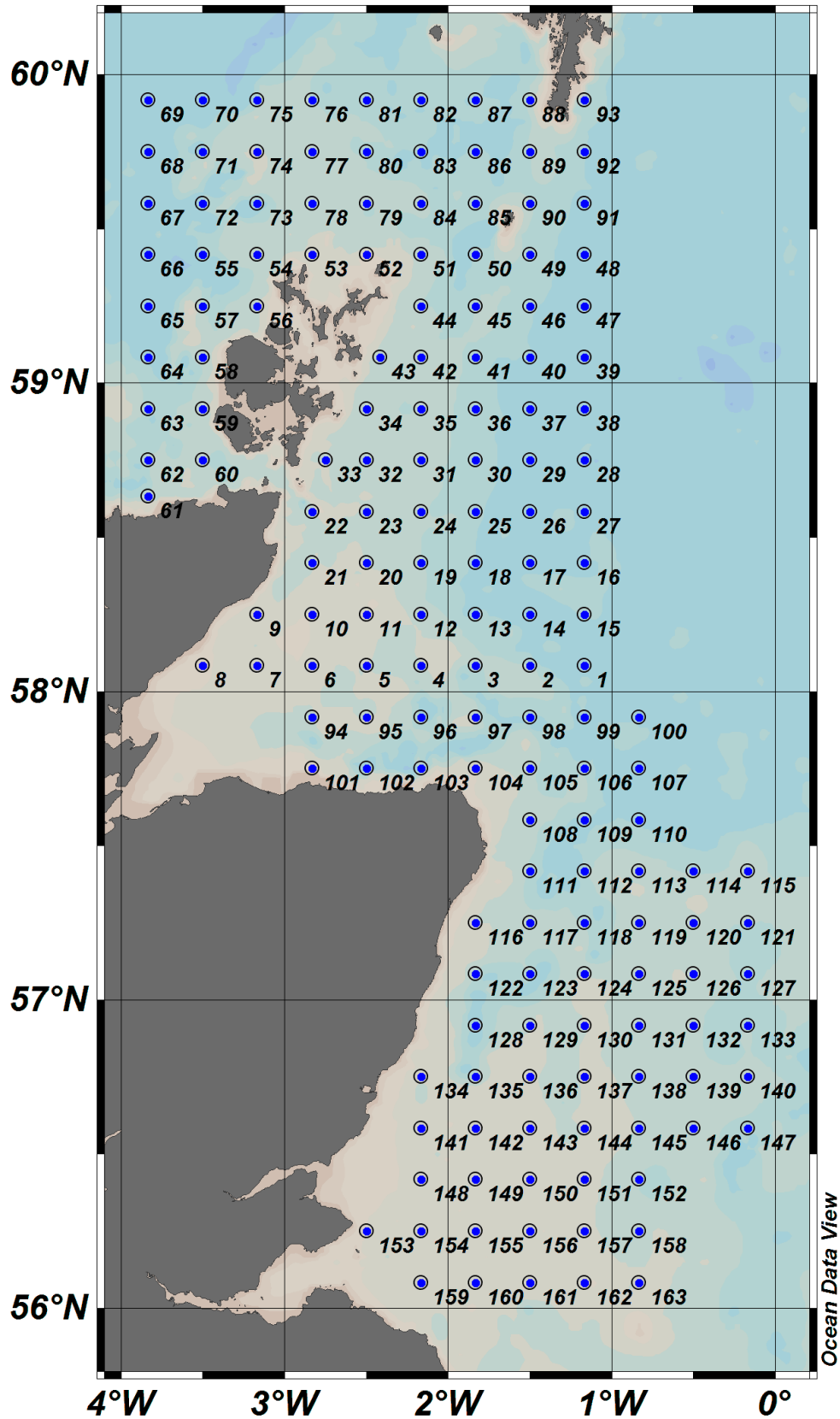
Figure 1: proposed station grid FRV „Walther Herwig III“, 09/22/15 – 10/02/15
