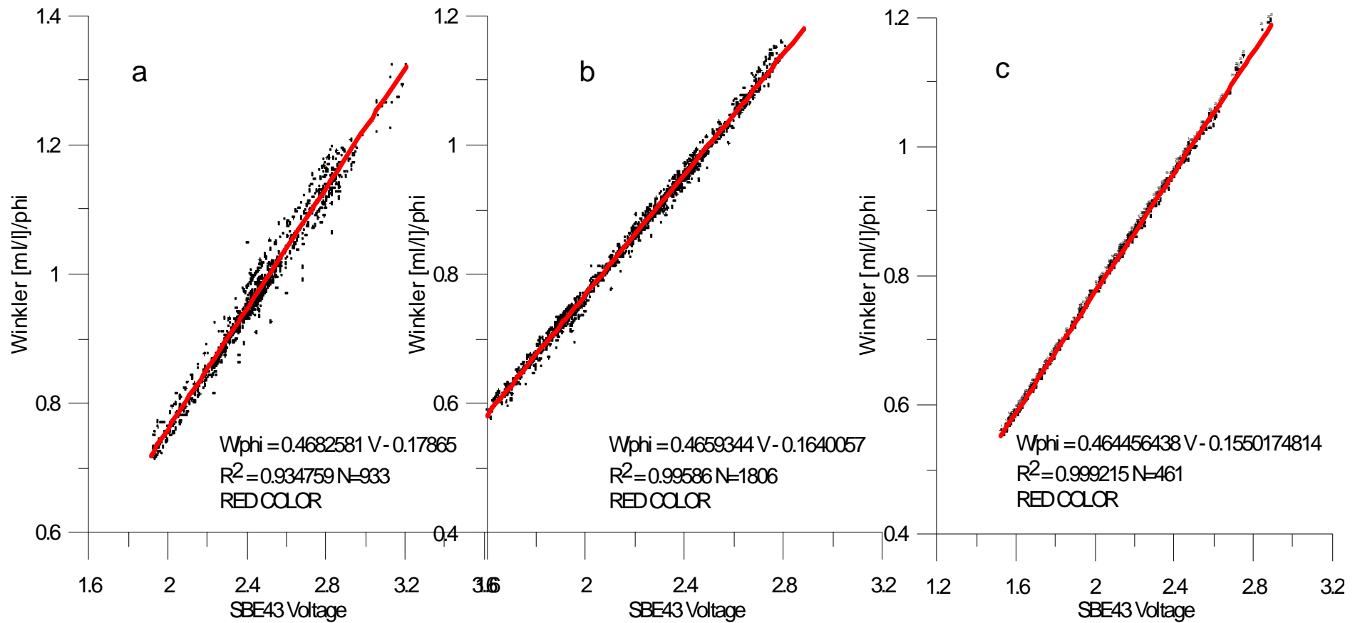
Figure 15 Regression lines for Winkler oxygen divided by \phi versus SBE 43 output voltage for (a) sill sections (b) 59.5 section and (c) the Labrador Sea. Oxygen data collected at the East Greenland shelf is regressed separately.
