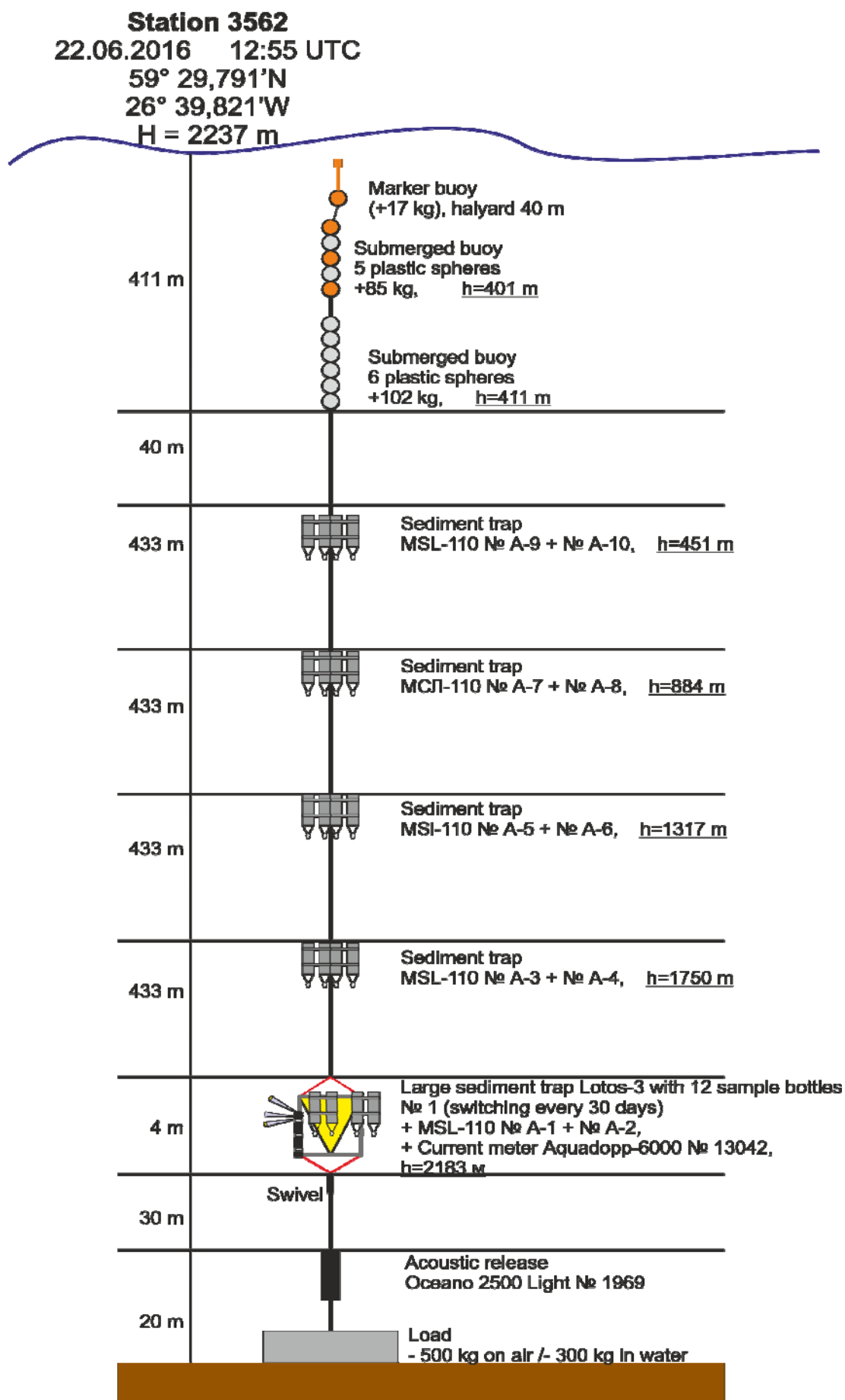
Figure 19. Mooring composition at sta. 3562.
