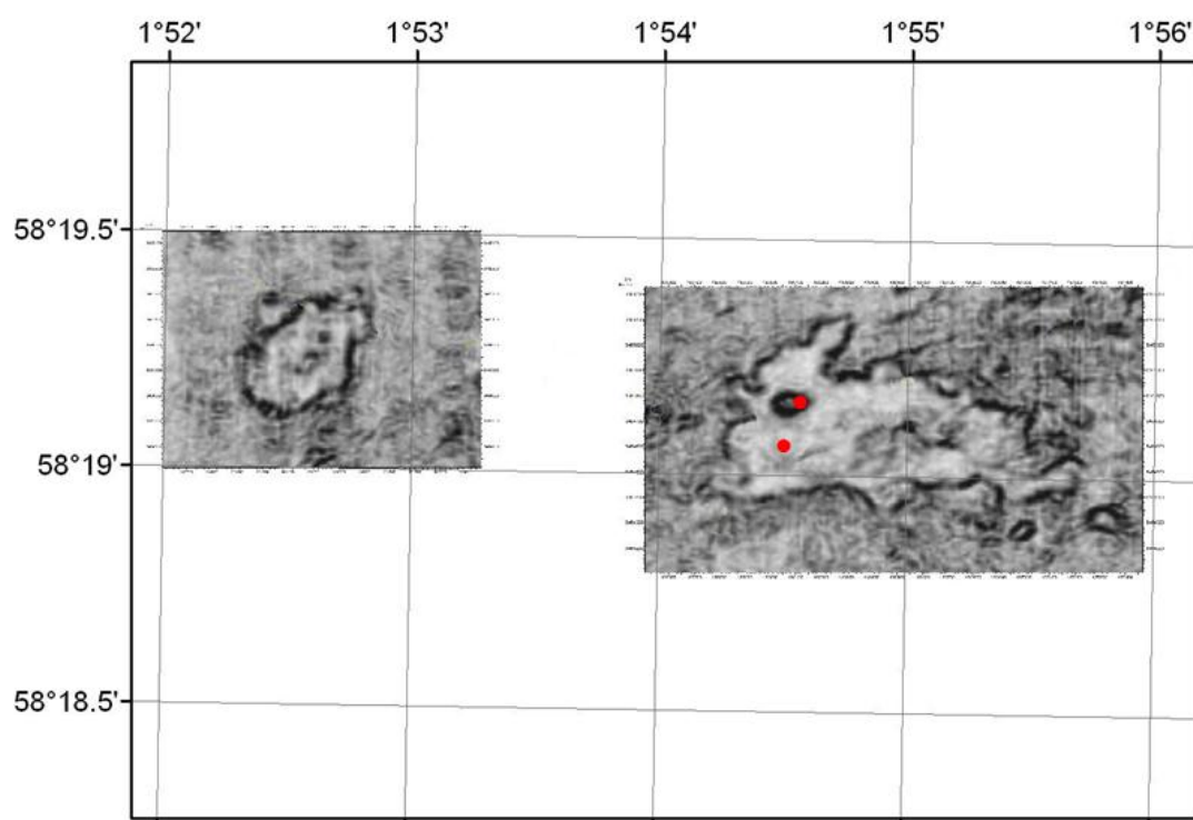
Figure 4.4.5: Vibro-Coring locations ('rabbits eye' and reference) at the seismic chimneys ~10 km south of Sleipner.
