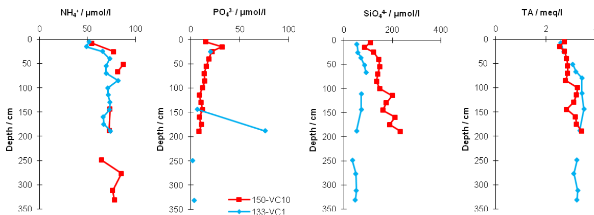
Figure 4.4.6: Reference VCs from the fracture north of Sleipner (blue) and the seismic chimneys south of Sleipner (red). Depths are given with respect to the top of the recovered core and are not corrected for any sediment loss that has occurred.
