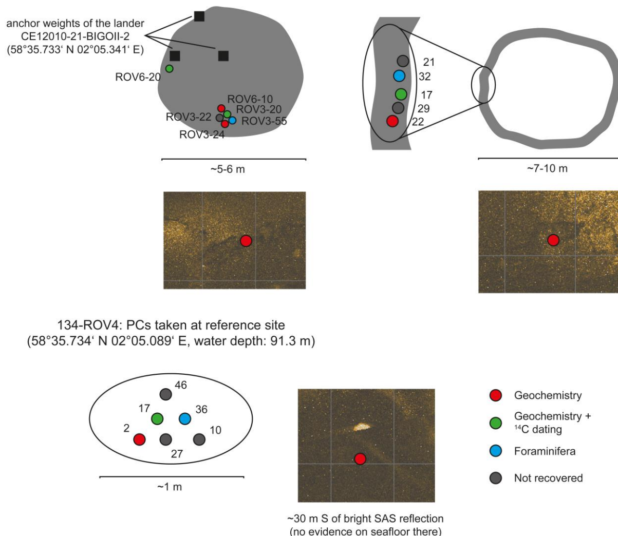
Figure 4.4.4: Details of the push coring at the fracture north of Sleipner. The PCs used for geochemical analyses including \delta D_{CH_4} and ^{14}C_{DIC} are indicated by red and green dots, respectively. Location of the BIGOII lander from CE12010 is given in ship coordinates. PC locations are ROV-coordinates.
