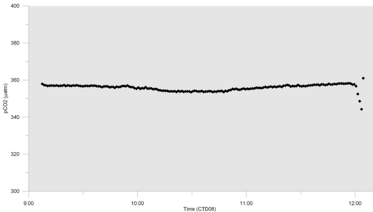
Fig. 4.1.9: p\text{CO}_2 concentrations determined by HydroC- \text{CO}_2 sensor during towed CTD08 (south-west of “fracture” area; towed at water depths of about 87 m). Note the slightly lowering of p\text{CO}_2 during uplift at the end of the track.
