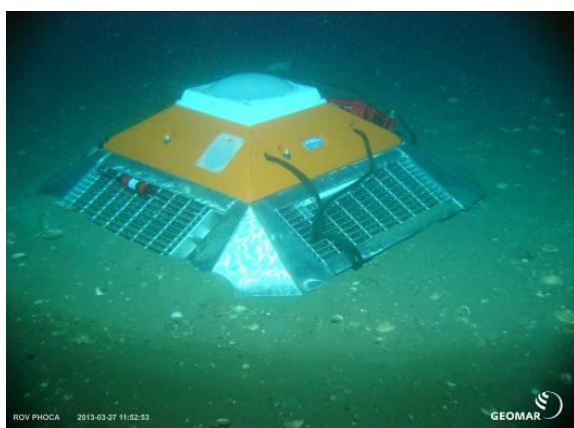
Fig. 4.2.3a: Trawl-resistant lander at the Blowout site.
