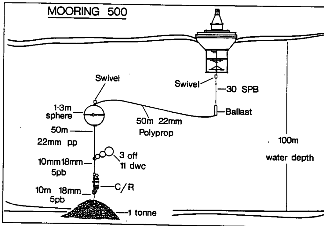
Figure 9. VAESAT mooring.
