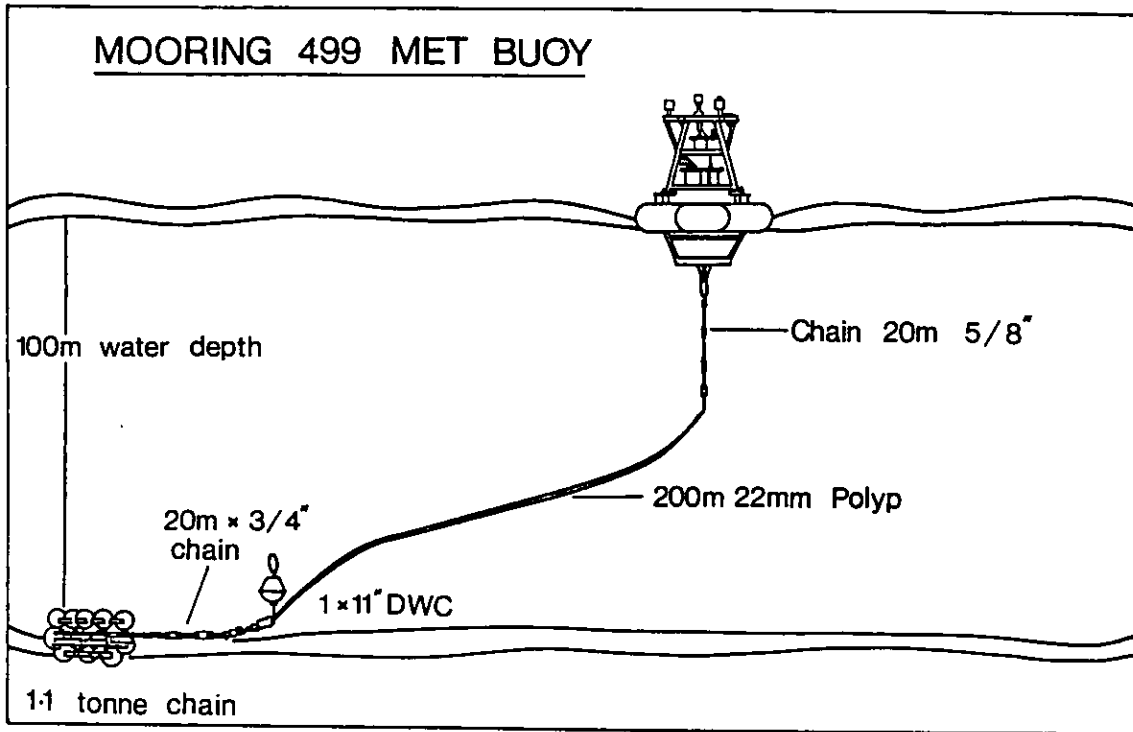
Figure 6. Meteorological mooring.
