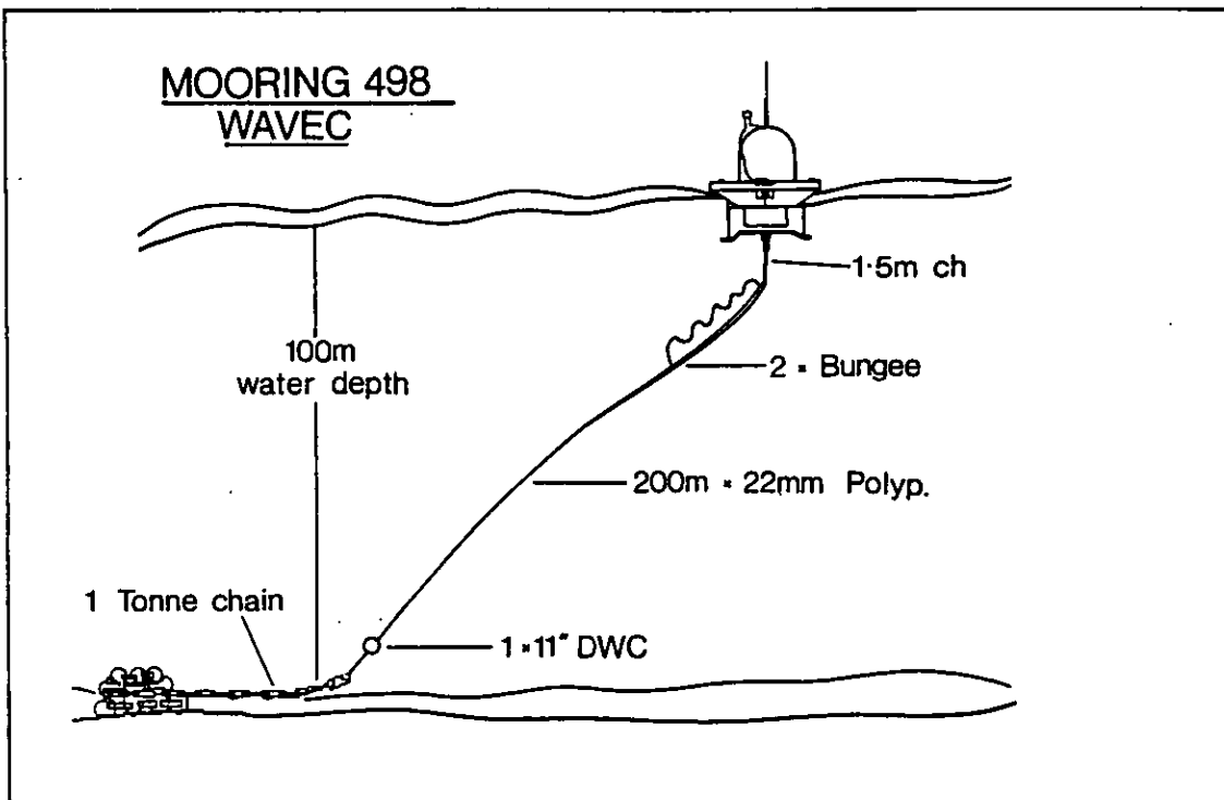
Figure 7. Wavec mooring.
