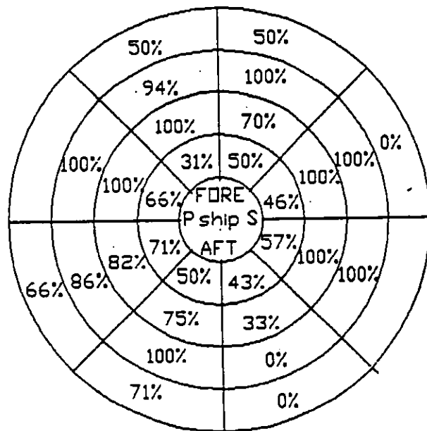
Figure 8. Range and relative bearing at which the Wavec was received.
