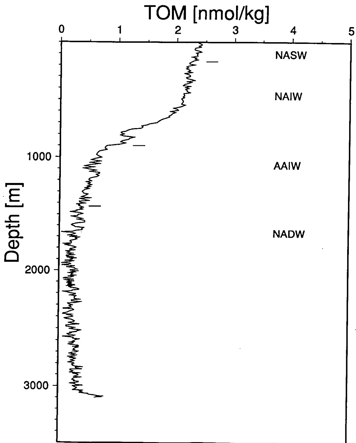
Fig 2.2 ZAPS Profile 053/16:01 - 18:25 26° 52.05' N 44° 29.38' W
