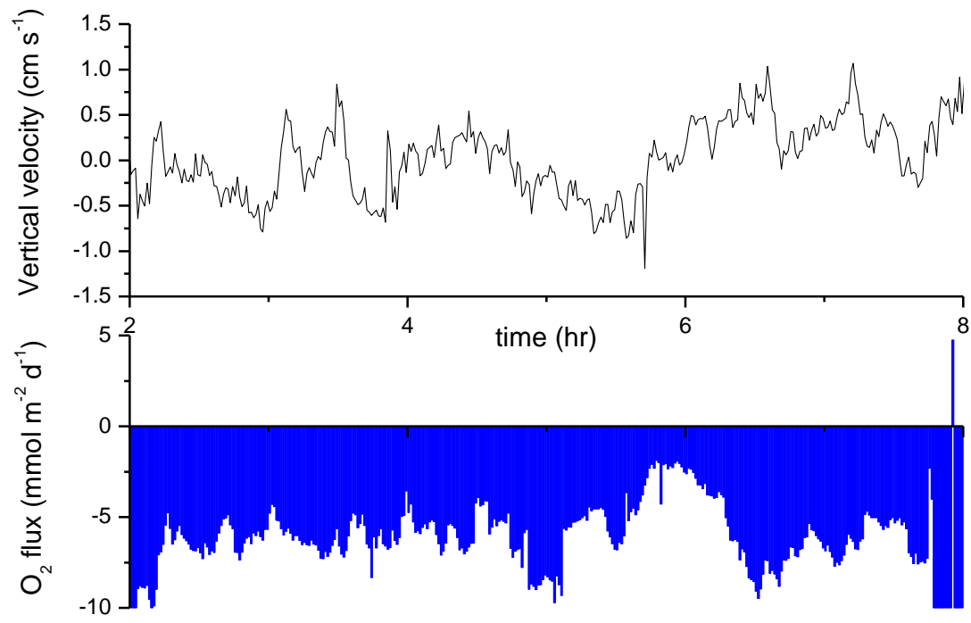
Fig. 4.5.3.1: Preliminary results showing variation in vertical velocity (top) and \text{O}_2 flux (bottom) at ~10 m away from a controlled- \text{CO}_2 -release site during the CE12010 expedition.
