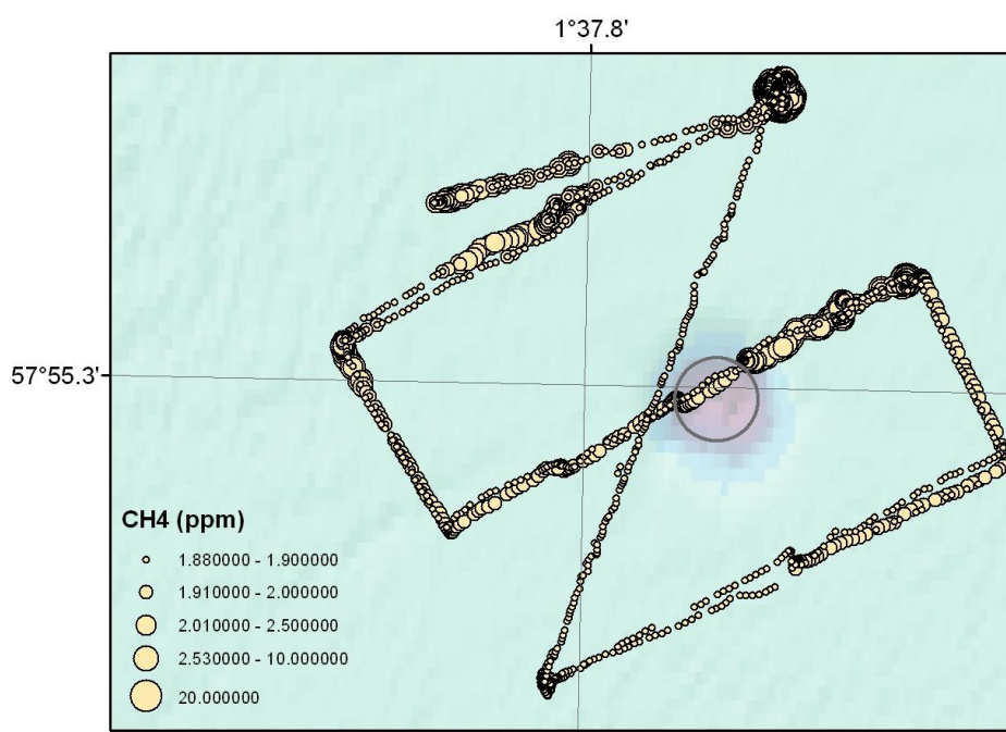
Fig. 4.1.3.7: Atmospheric methane concentration measured 2 m above sea level at the Blowout site (01.08.2012). Data is recorded in parallel to a water sampling campaign.
