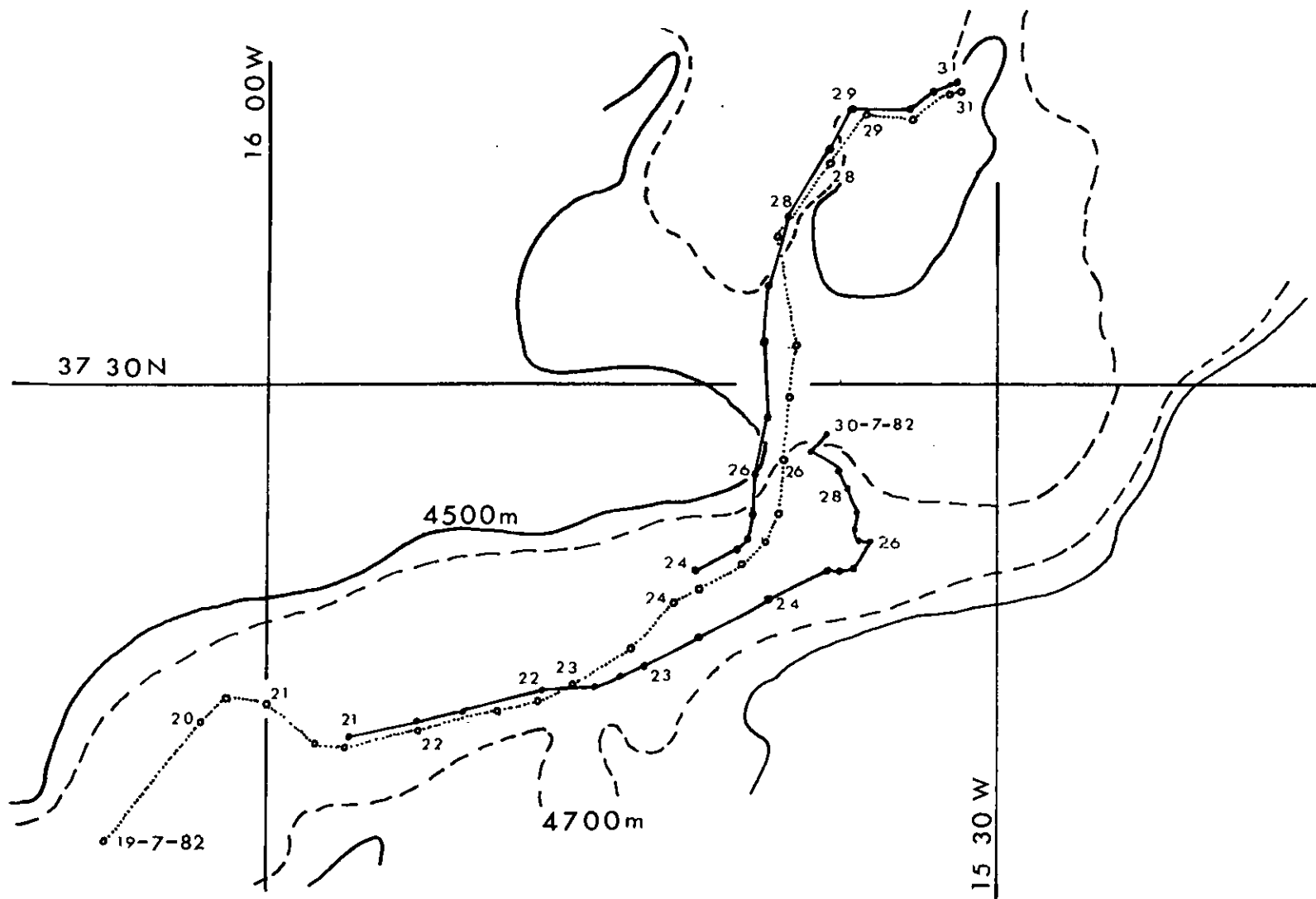
Figure 5. Selected float tracks ; fixes for 22-24z of date
