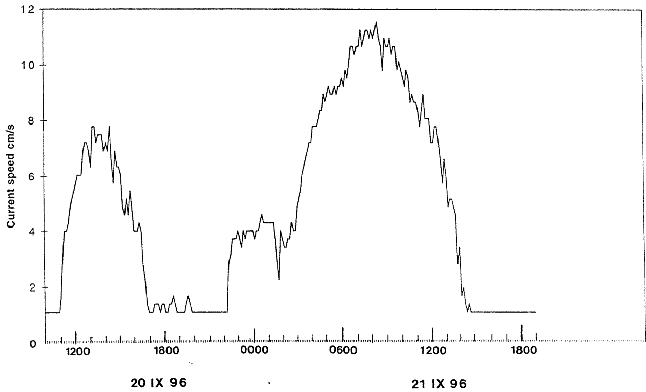
Figure 10 Bathysnack deployment 12930#89 current meter data; variations in current speed with time.
