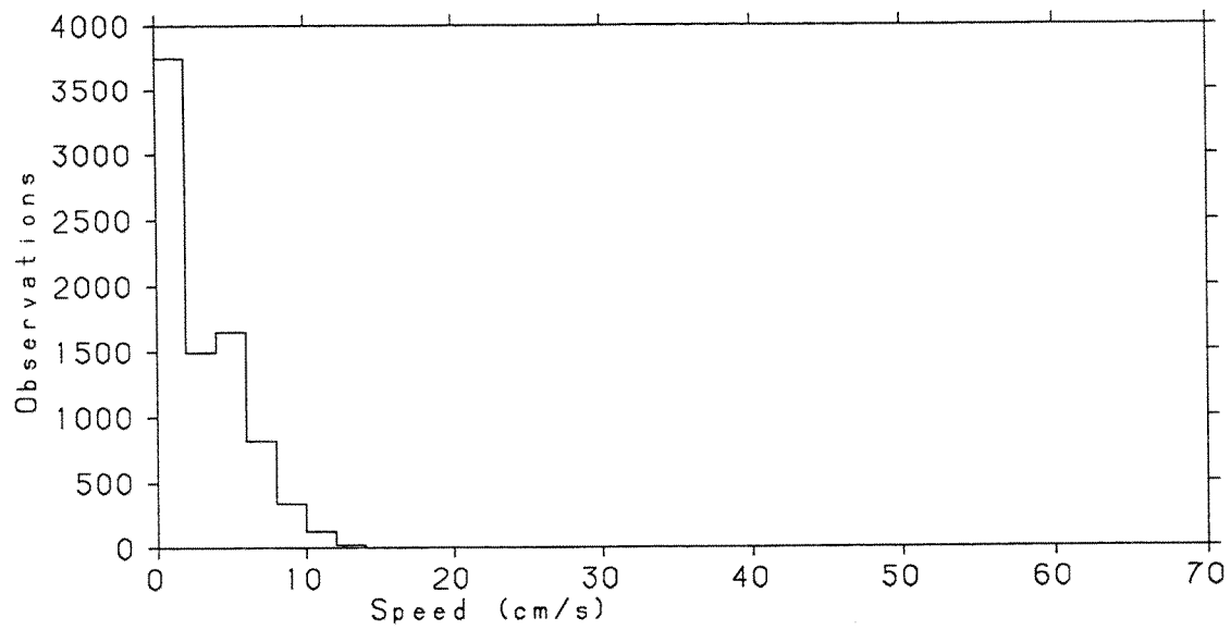
Figure 8 Sediment trap mooring 12812#2; current meter data from c180mab. Distribution of recorded current speeds.
