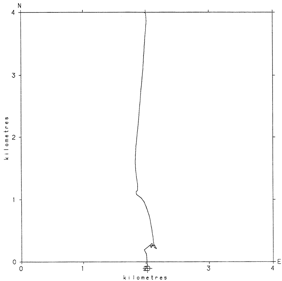
Figure 11 Bathysnack deployment 12930#89 current meter data; progressive vector diagram.
