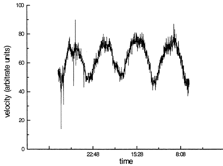
Figure 12 Variations in current speed c30cm above the bottom measured during the NIOZ lander deployment #23.
