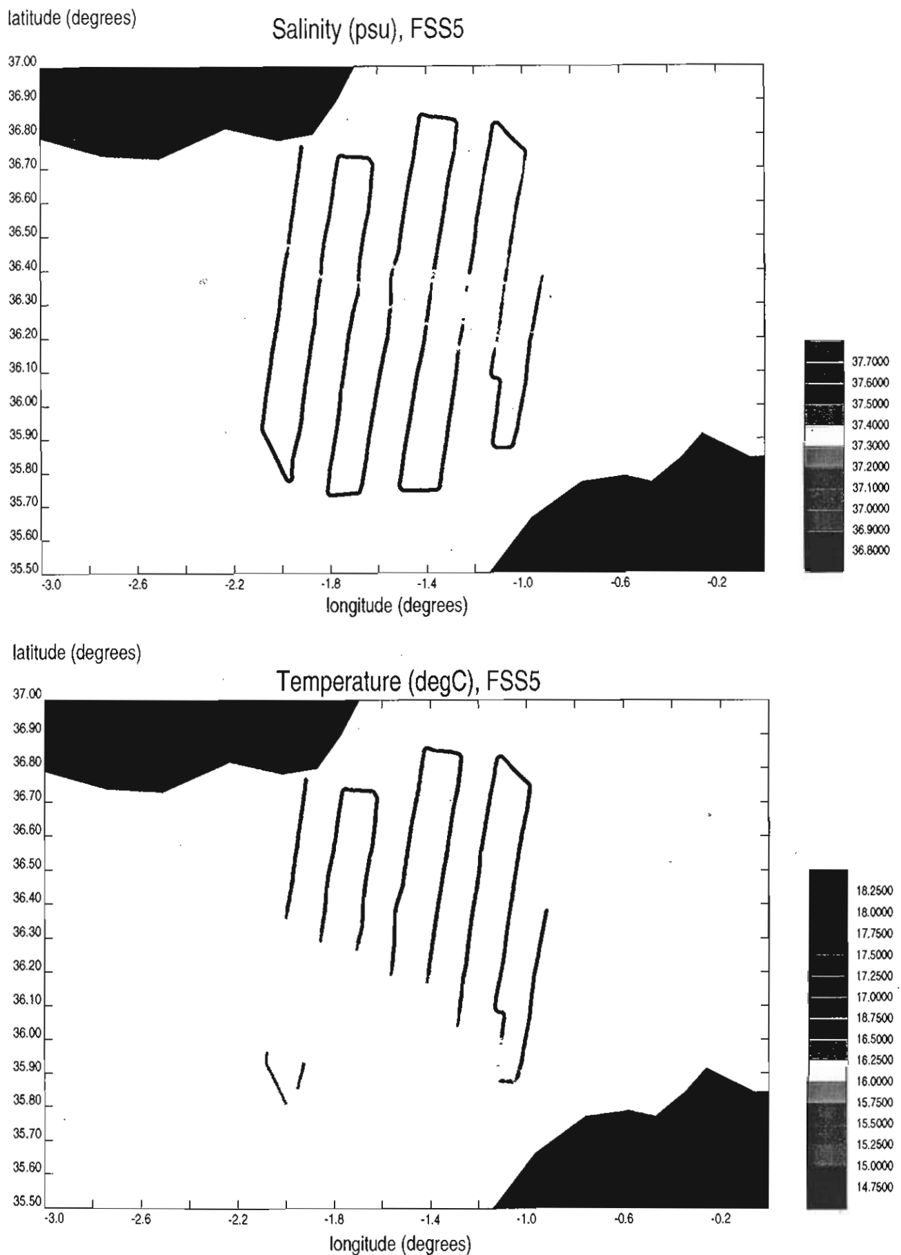
Figure 3. Near-surface profiles of salinity and temperature recorded by the shipborne thermosalinograph during the fine-scale SeaSoar survey (FSS5) at the end of Discovery Cr. 224 leg 2.
