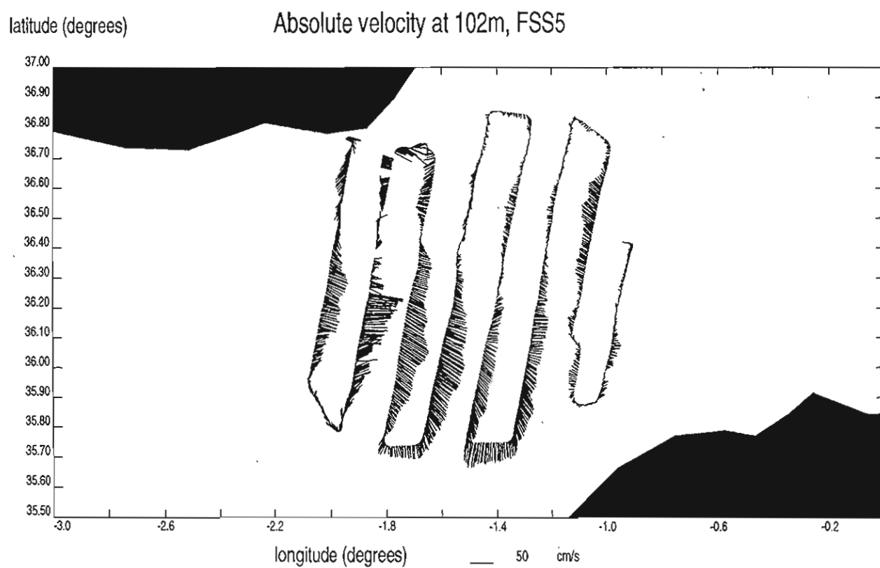
Figure 5. VM-ADCP current vectors at 14 and 102 m for the fine-scale SeaSoar survey (FSS5) at the end of Discovery Cr. 224 leg 2.
