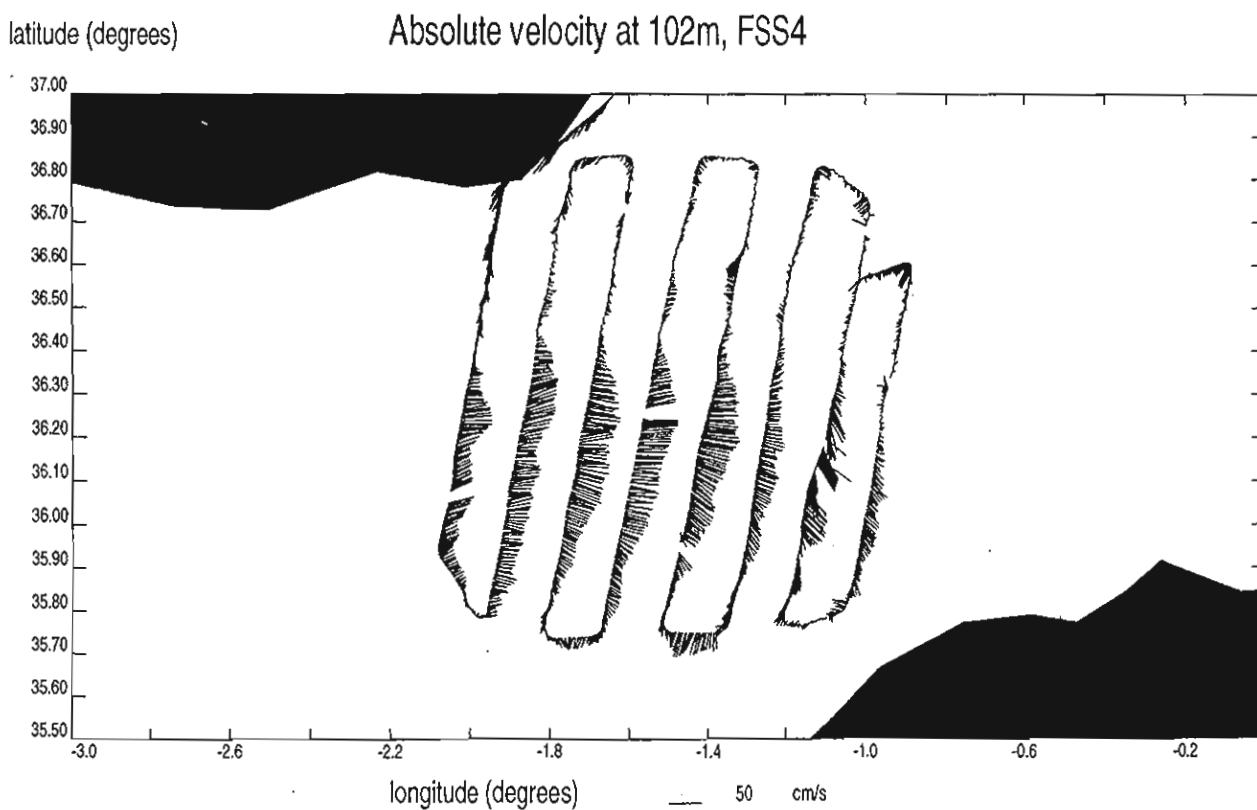
Figure 4. VM-ADCP current vectors at 14 and 102 m for the fine-scale SeaSoar survey (FSS4) at the start of Discovery Cr. 224 leg 2.
