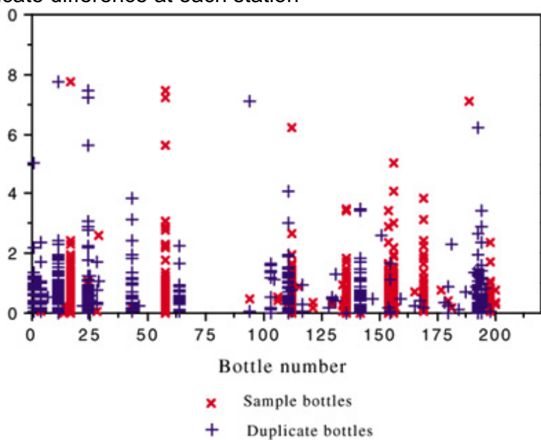
Figure 7.2b: Comparison of duplicate difference with bottles used
