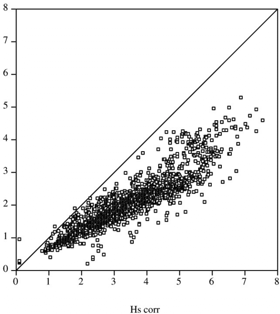
Figure 6.1: Comparison of Hs corrected (Hs corr) and Hs uncorrected (Hs raw)
