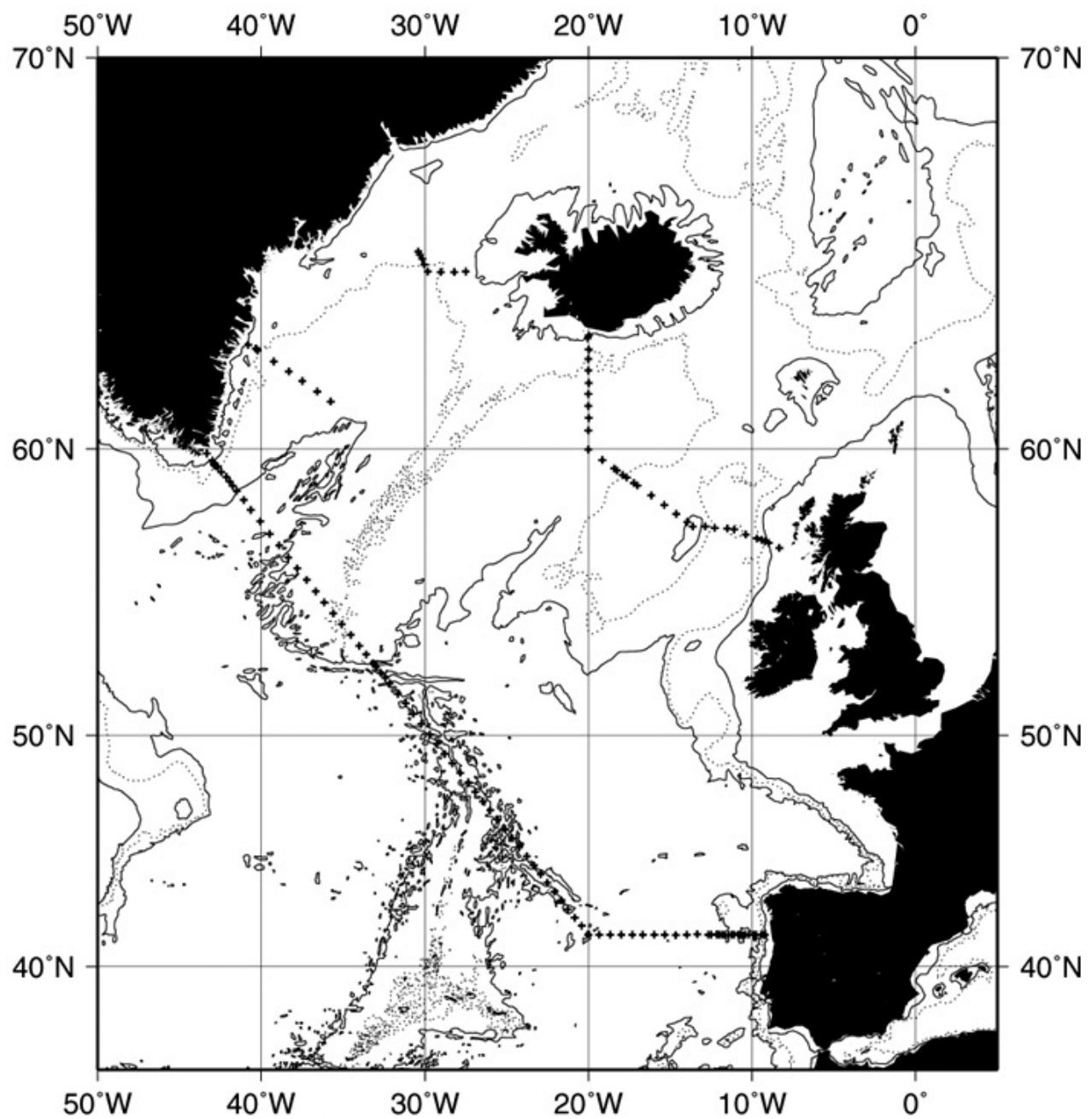
Figure 1.2: Discovery Cruise 230 station positions. Bathymetry is 200m (solid), 1500m (dots), 3000m (solid).
