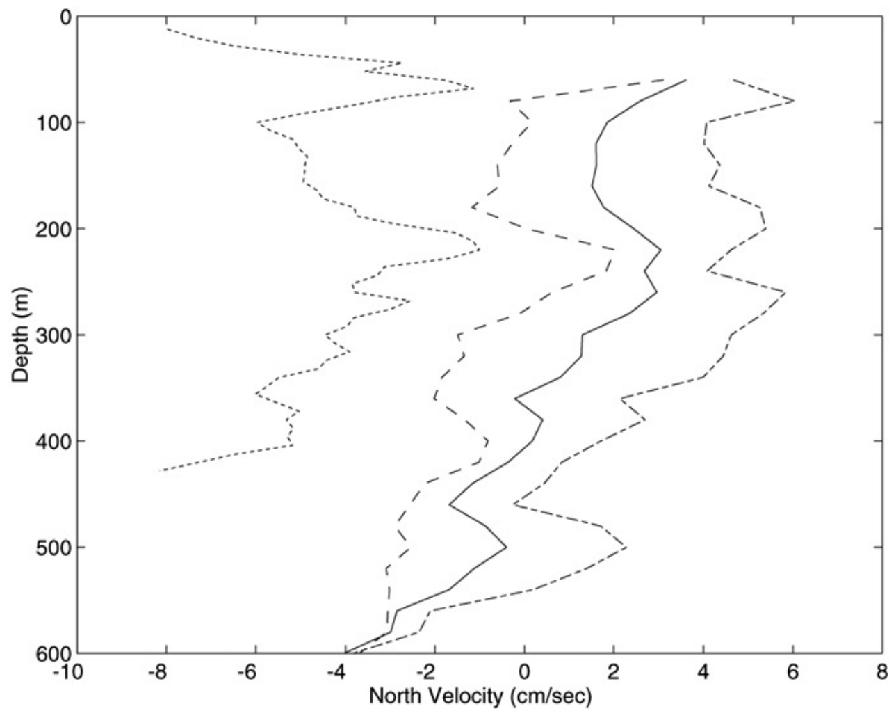
Figure 3.1: VM- and L-ADCP profile comparisons for station 85; VM-ADCP: short dash; L-ADCP: down (chain), up (long dash), mean (solid).
