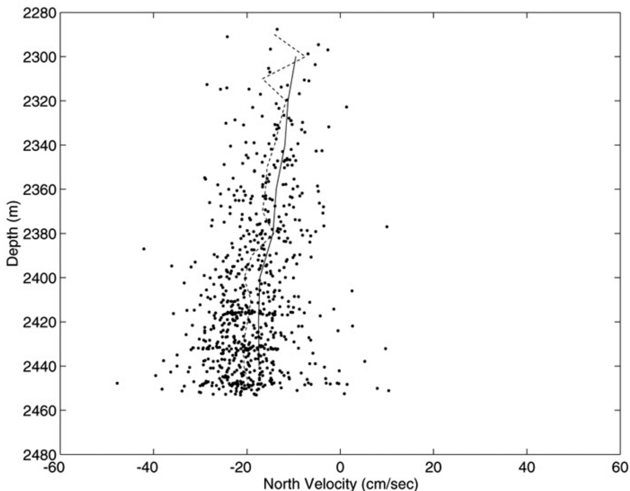
Figure 3.2: LADCP water track/bottom track comparison: station 85 bottom track velocity scatter plot with 10m bin average (dashed line) and water track velocity (solid line).
