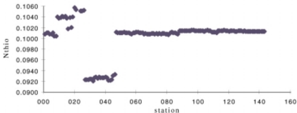
Figure 7.1: Variations in thiosulphate normality
