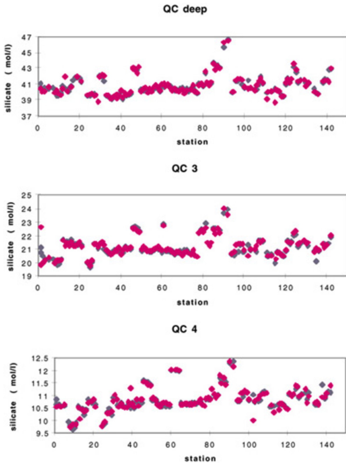
Figure 7.3a:Silicate QC Deep, QC 3, QC 4.
