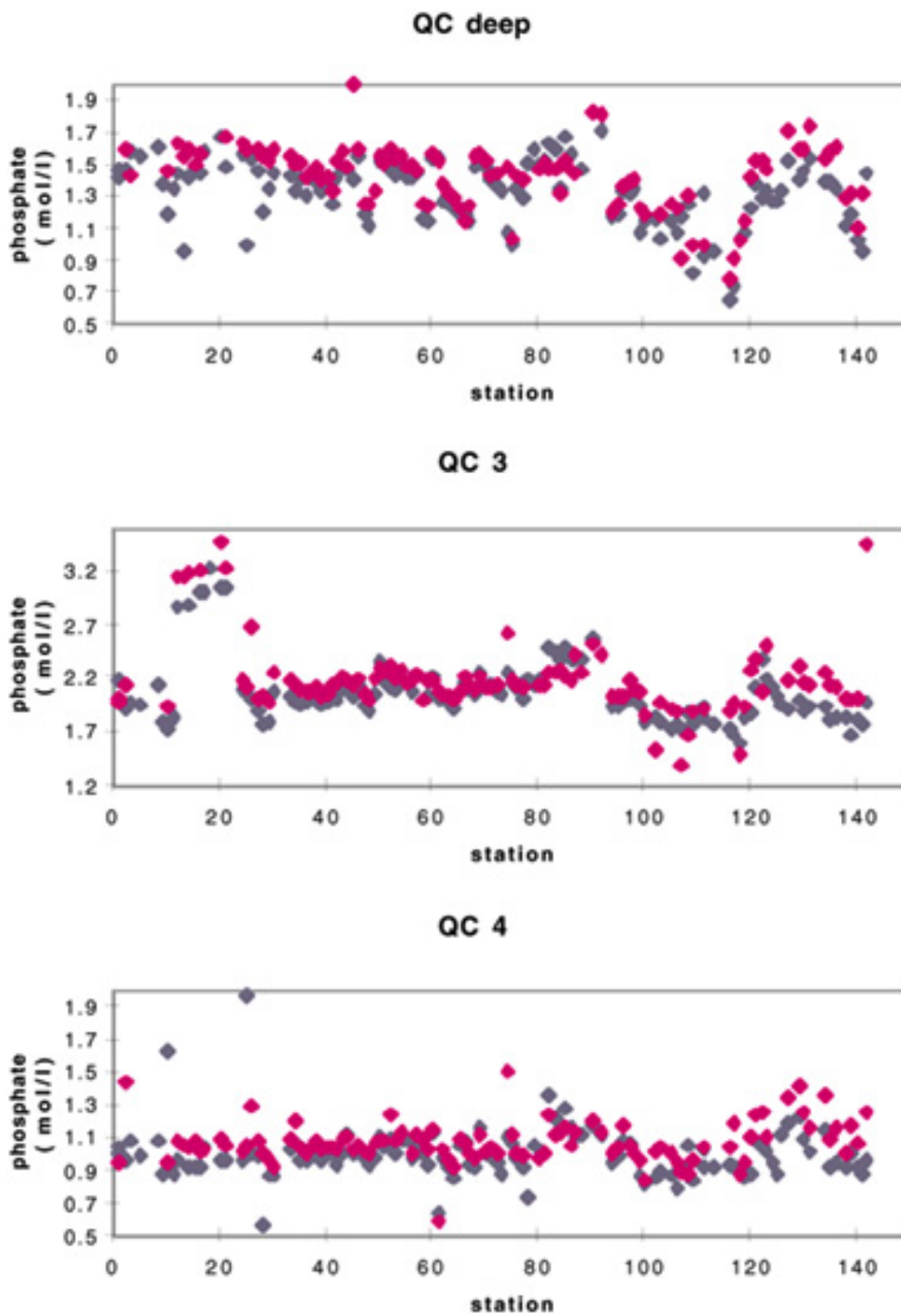
Figure 7.3c: Phosphate QC Deep, QC 3, QC 4.
