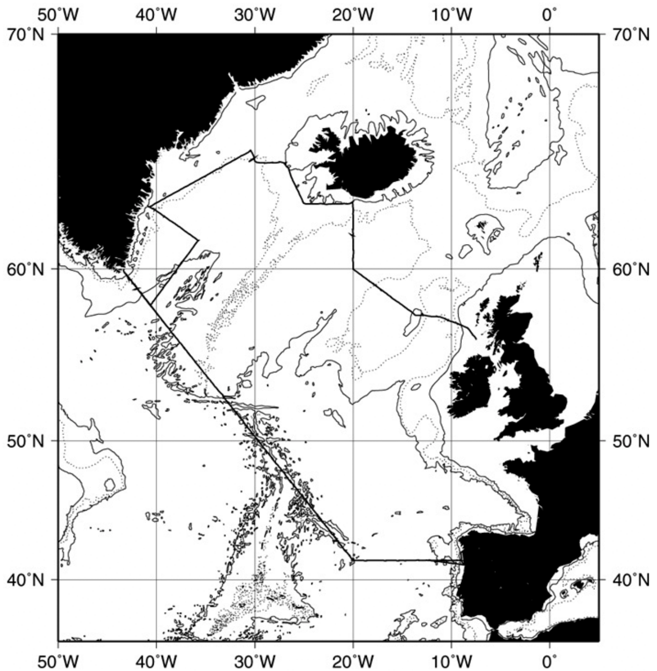
Figure 1.1: Discovery Cruise 230 track Vigo to Southampton. Bathymetry is 200m (solid), 1500m (dots), 3000m (solid).
