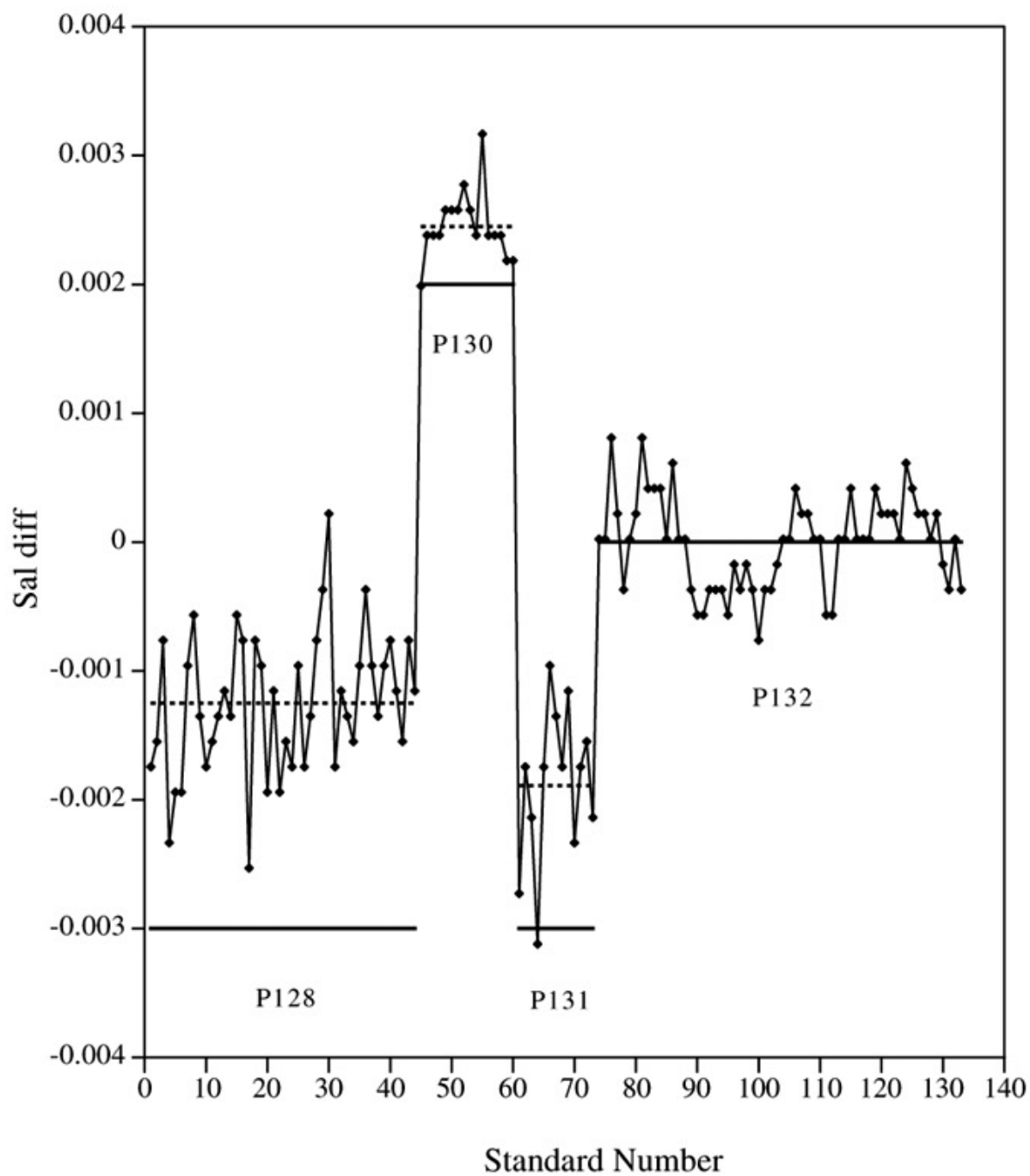
Figure 7.4: Salinity standard history. Broken lines show measured mean over each batch, full lines show mean assuming correct batch label salinity and P132 measured mean correct (same as label).
