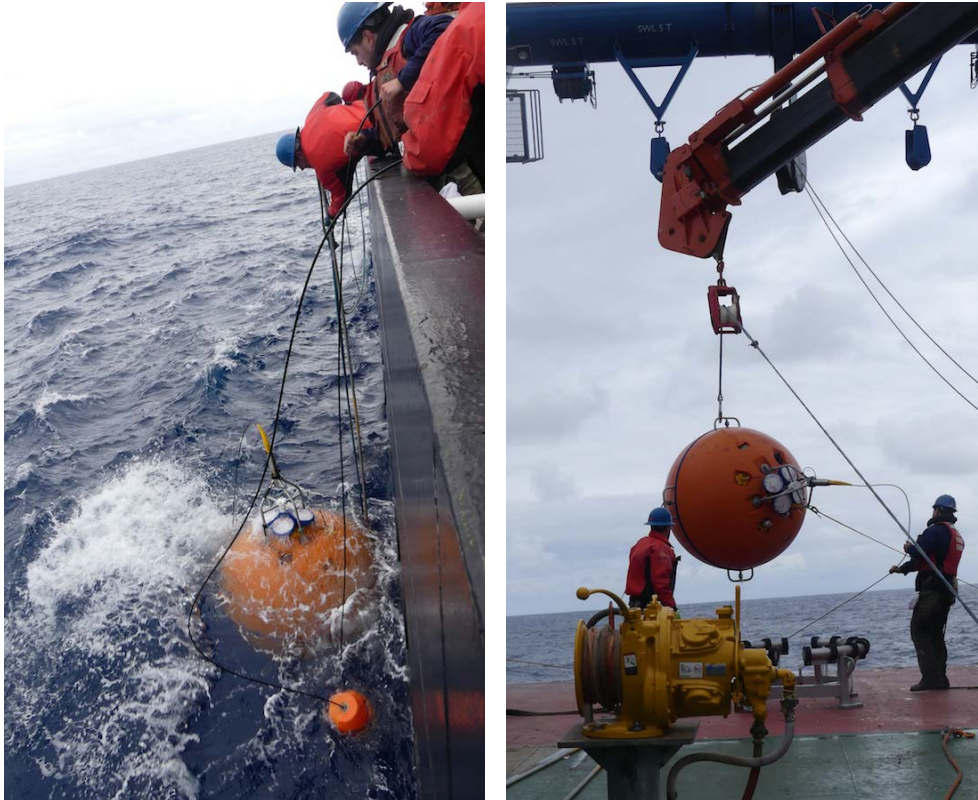
Figure 12 – Hooking the FLMA-3 62" sphere (left) and bringing it on deck (right).
