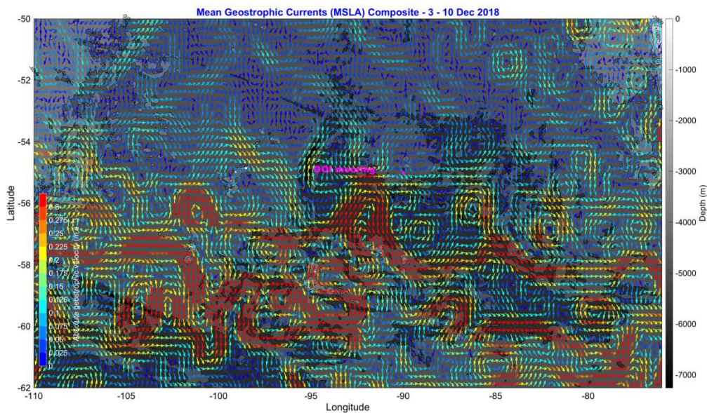
Figure 29: Mean Geostrophic Currents from Mean Sea Level Anomaly (MSLA)
