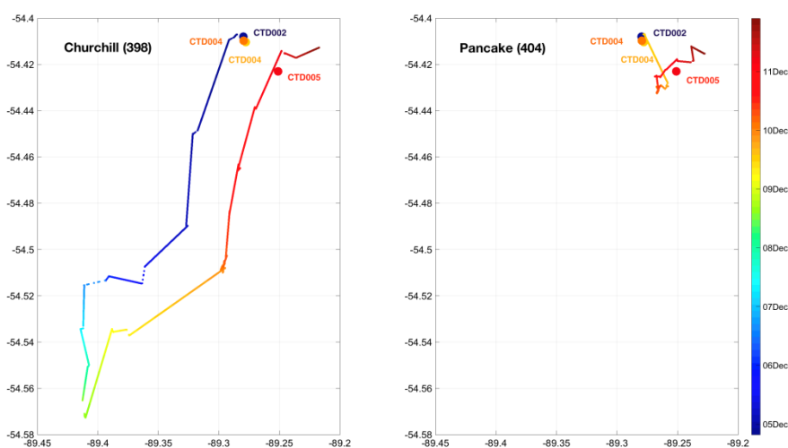
Figure 20: Location of CTD calibration casts (large dots) and glider tracks. Colour indicates time, so large dots close to the track with the same colour indicate that glider was nearby when cast happened.
