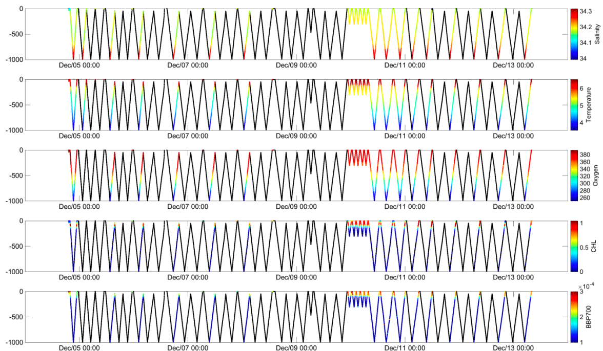
Figure 17: Sampling scheme for Churchill (unit 398) since deployment. Black line indicates glider dives. Colour indicates when respective variable was sampled. Glider has been alternating between (1) 3 yo's per segment, sampling in the last upcast ("low power mode"), (2) double dives, sampling on the last upcast, (3) single dives sampling both casts (for calibration purposes – CTDs occurred during this period), and (4) single dives, sampling in the upcast.
