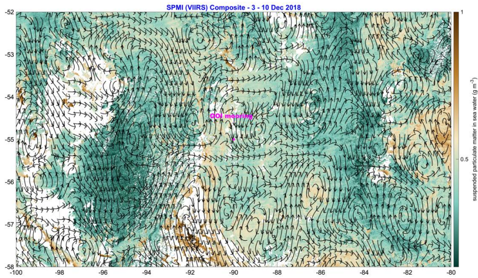
Figure 32: Total Suspended Particulate Matter (SPMI) from VIIRS
