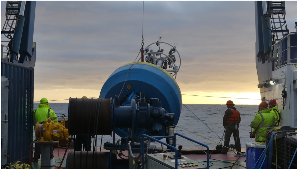
Figure 5 – GS01SUMO-00004 Buoy Deployment.
