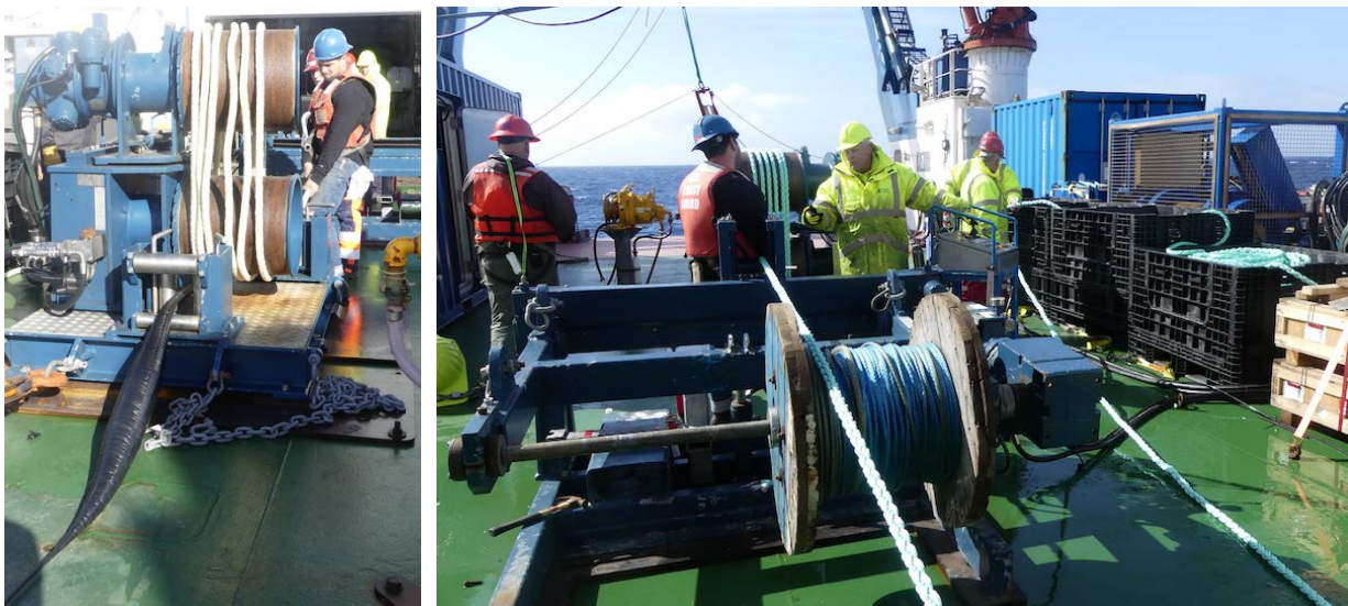
Figure 7 – Wire to rope transition (left) and Colmega (right) passing through the Lebus winch
