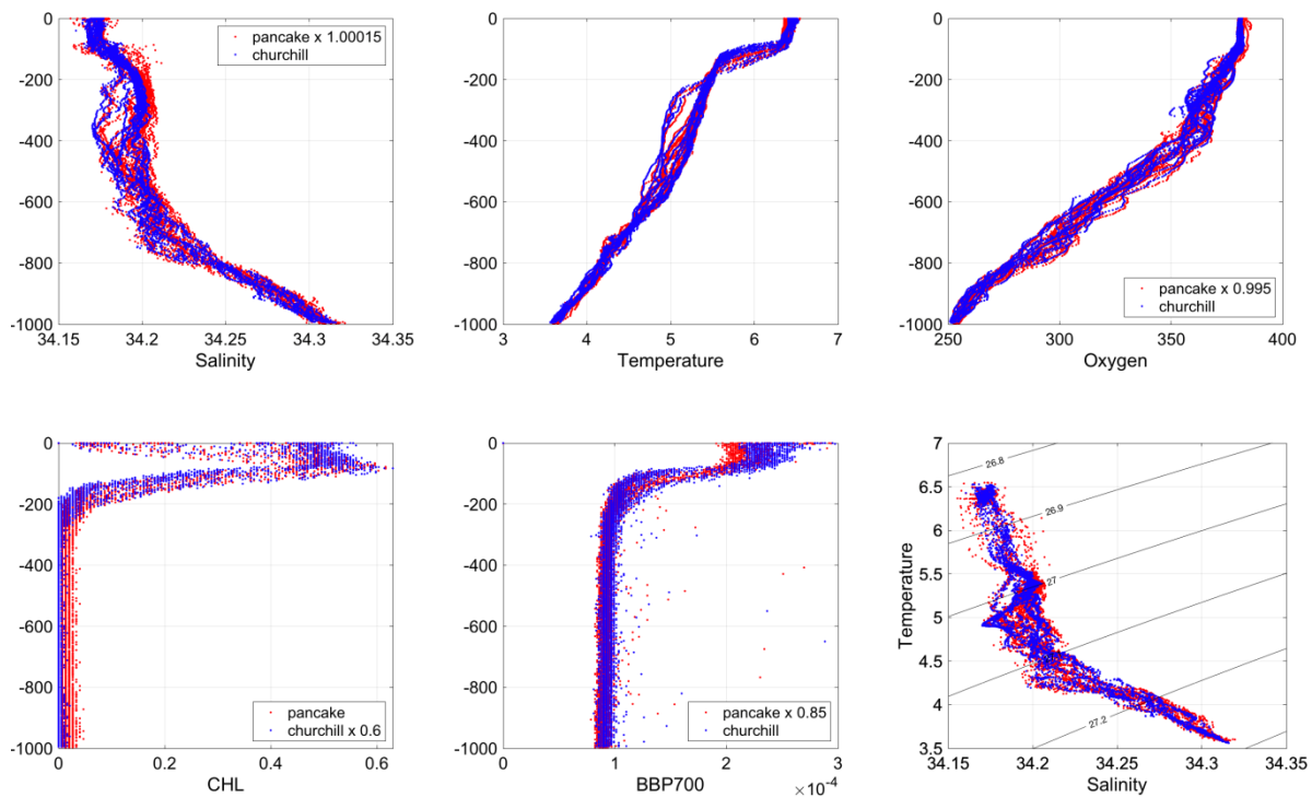
Figure 19: Depth profiles of Salinity, Temperature, Oxygen, Chlorophyll (CHL) and Backscattering at 700nm (BBP700) as well as a TS diagram. Colours indicate glider (Pancake in red and Churchill in blue). Scale shown was just illustrative, as no inter-calibrations have been done.
