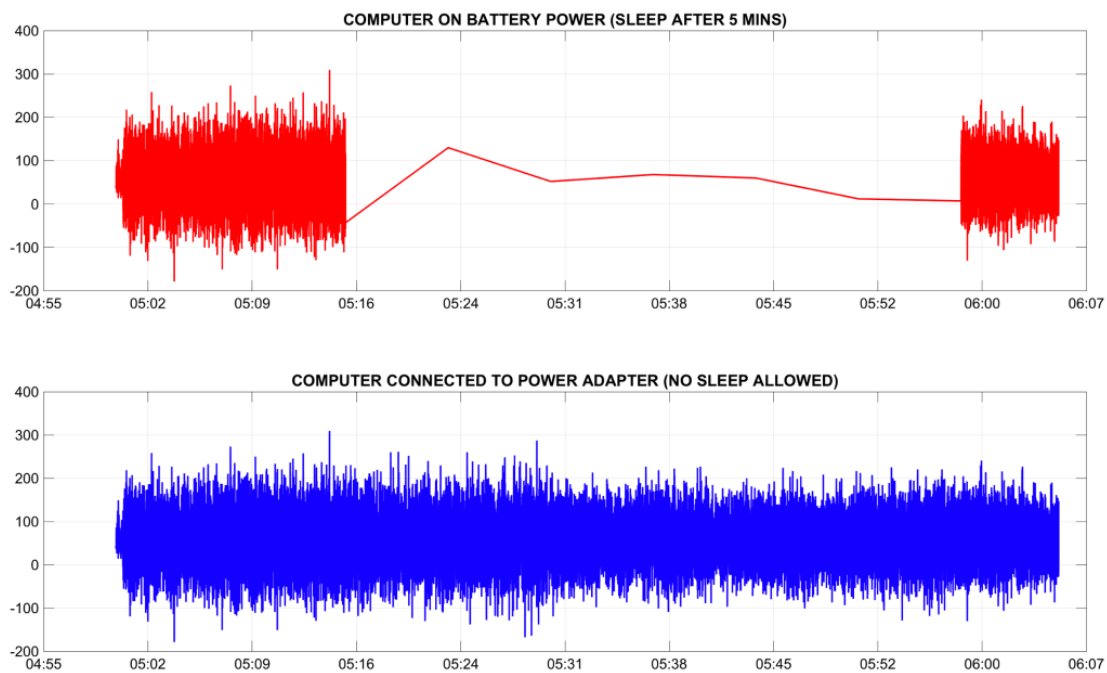
Figure 25: Data transfer for the same file with: (top) computer on battery power and energy setting to let computer sleep after 5 minutes; (bottom) computer connected to a power source, without going to sleep during the transfer
