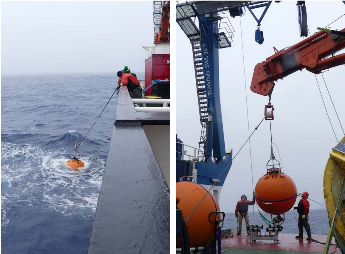
Figure 14 – Hooking the FLMB-3 62" sphere, and using the starboard A-frame winch to level it.
