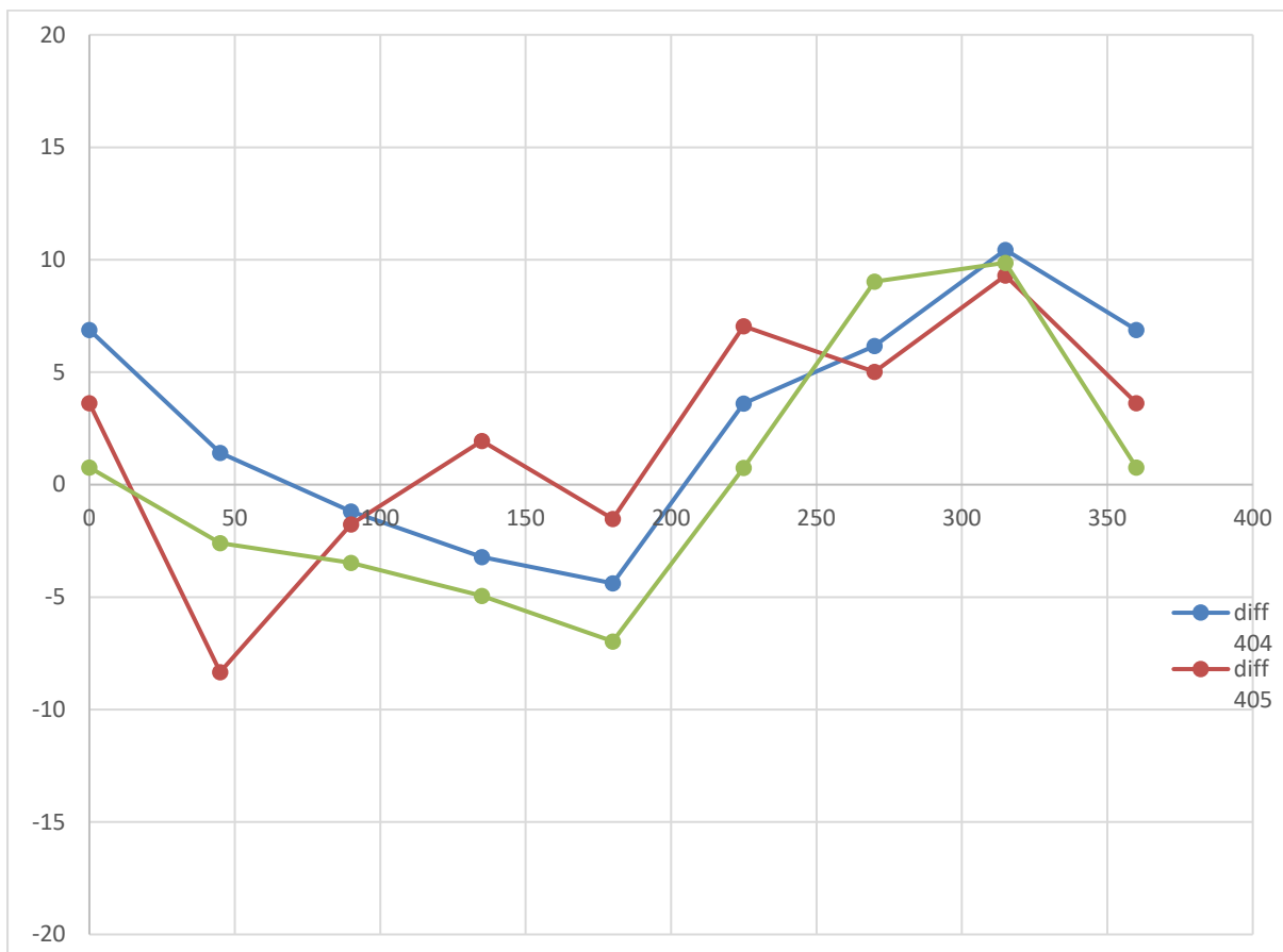
Figure 15: glider compass check
