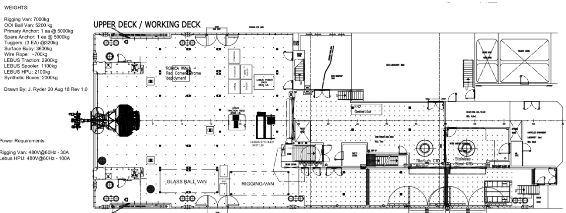
Figure 2 – Planned Deck Layout
