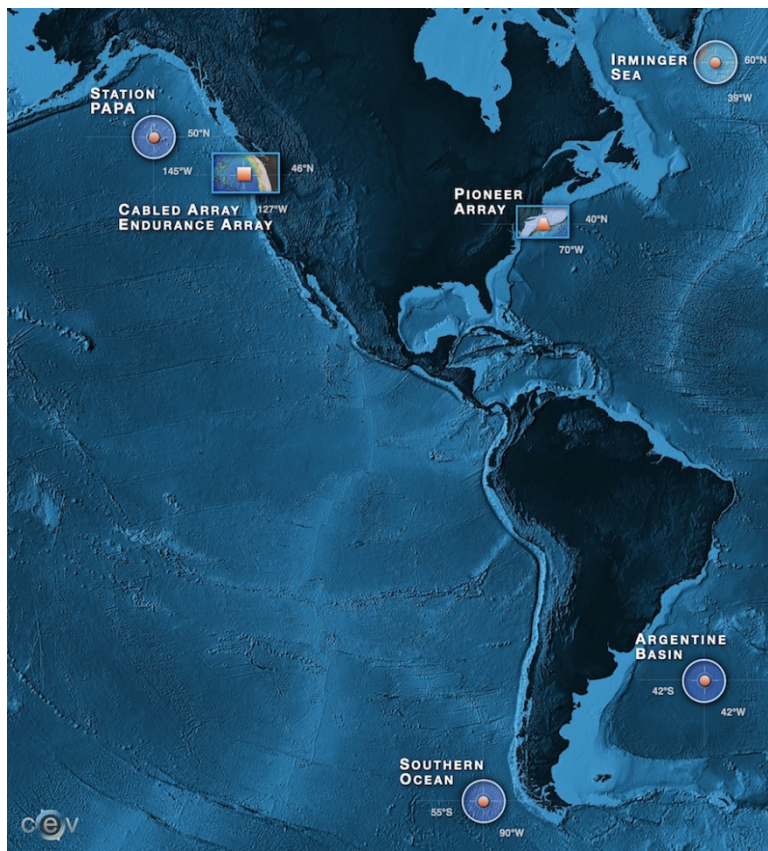
Figure 1 – Ocean Observatories Initiative (OOI) Array Map
