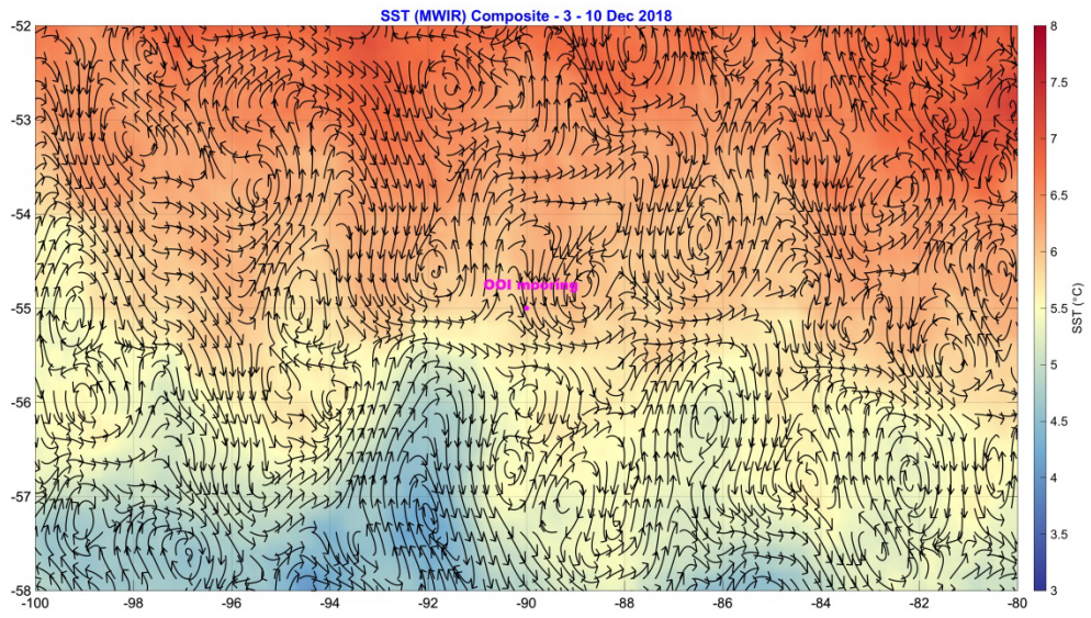
Figure 30: Sea Surface Temperature (SST) from MWIR with mean geostrophic currents overlaid
