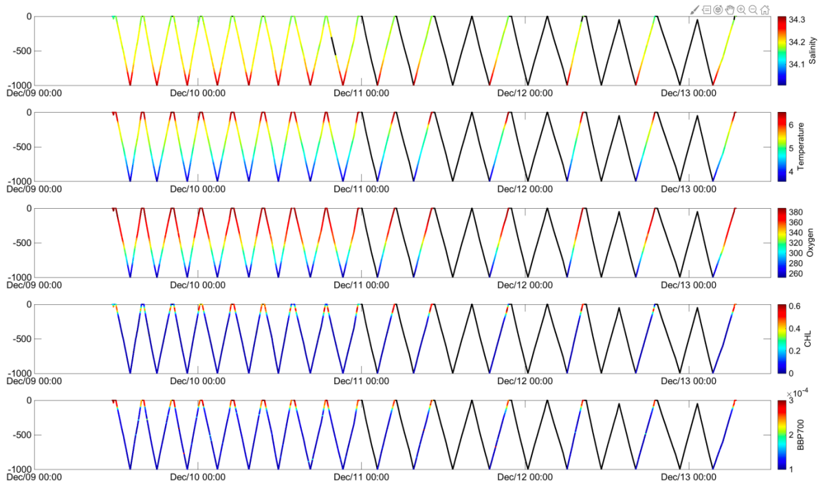
Figure 18: Sampling scheme for Pancake (unit 404). Later deployment for Pancake as it was the backup glider. Same flight details as Churchill.
