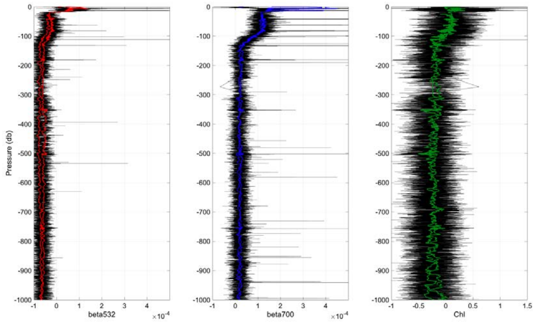
Figure 21: Depth profiles of data collected using the ECO triplet ( EcoPuck_003_201812091347.mat ) on CTD003 (event 11). Black lines are unaveraged. Solid thick lines for beta532 (red), beta700 (blue) and chlorophyll (green) are smoothed using a 11-point (1 s, or 0.2 m) running median followed by a 51-point (5 s, or 1 m) running mean.
