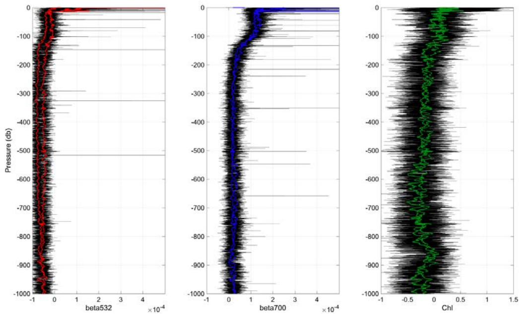
Figure 22: Depth profiles of data collected using the ECO triplet ( EcoPuck_005_201812110703.mat ) on CTD005 (event 18). Black lines are unaveraged. Solid thick lines for beta532 (red), beta700 (blue) and chlorophyll (green) are smoothed using a 11-point (1 s, or 0.2 m) running median followed by a 51-point (5 s, or 1 m) running mean. Raw profiles are very noisy due to lack of internal averaging, but backscattering spikes due to large particles are very well resolved.
