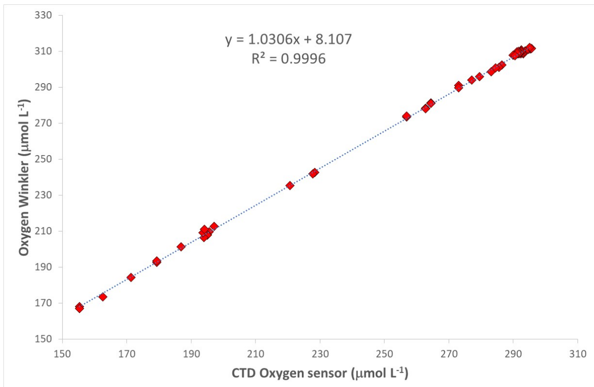
Figure 27. CTD oxygen measurement against oxygen concentration determined by Winkler
