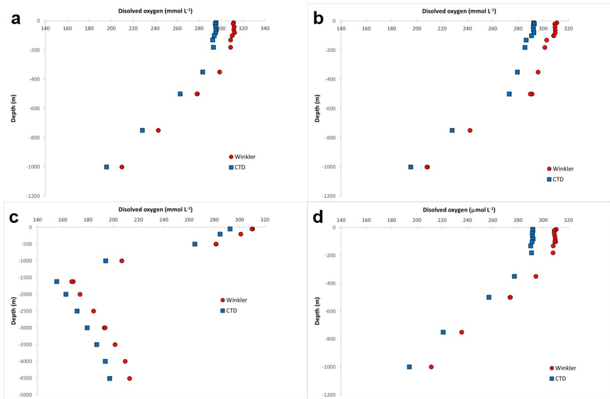
Figure 28. Profile comparison between CTD measurements and Winkler oxygen determination. a) Cast 002, b) Cast 003, c) Cast004, d) Cast 005.
