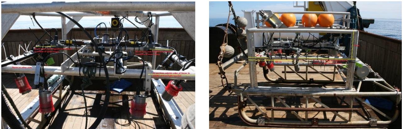
Figure 3 – Sledge used during CEnd 10/18, showing the equipment setup. Photos by Chris Firmin (Cefas).
