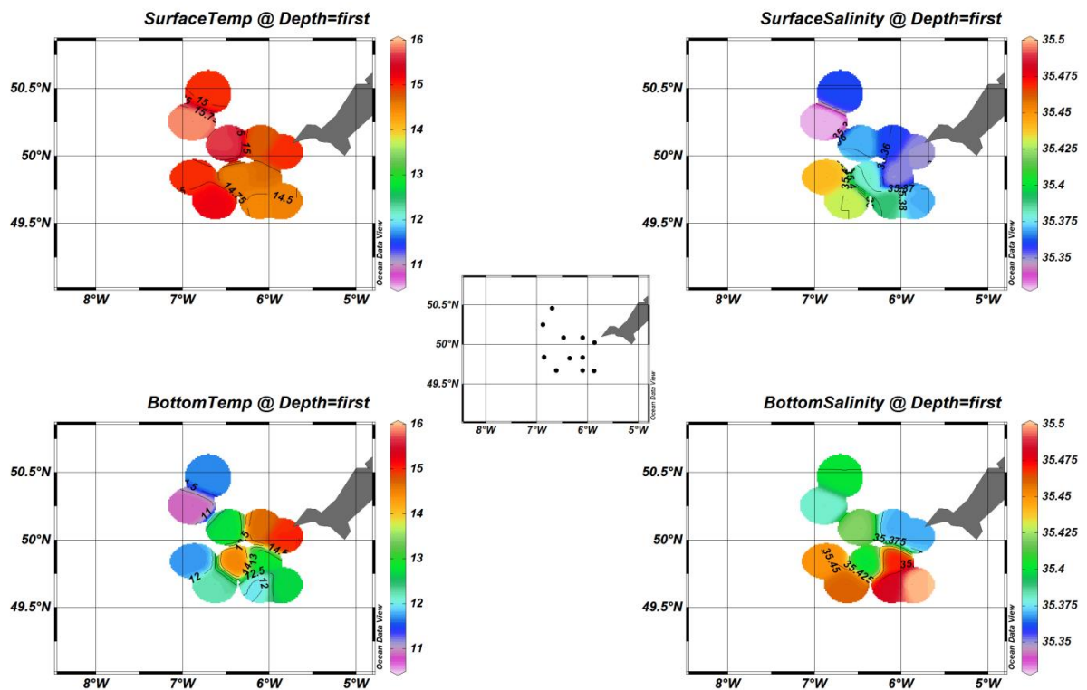
Figure 11. Values of temperature (°C) and salinity at the surface and bottom at the stations in the Isles of Scilly (SI), as measured by the SAIV MiniCTD.
