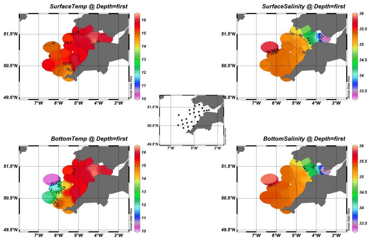
Figure 12. Values of temperature ( ^{\circ}\text{C} ) and salinity at the surface and bottom at the stations in the Bristol Channel (BC), as measured by the SAIV Mini CTD.
