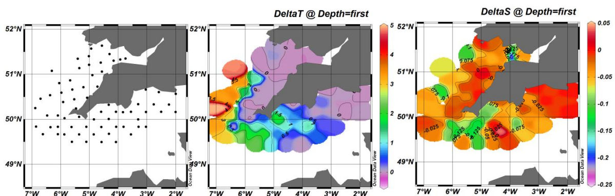
Figure 13. Values of \Delta T (surface temperature – bottom temperature; ^{\circ}\text{C} ) and \Delta S (surface salinity – bottom salinity) at the 70 sampling stations, as measured by the SAIV MiniCTD. The water column is considered stratified when \Delta T > 0.5\text{ }^{\circ}\text{C} .
