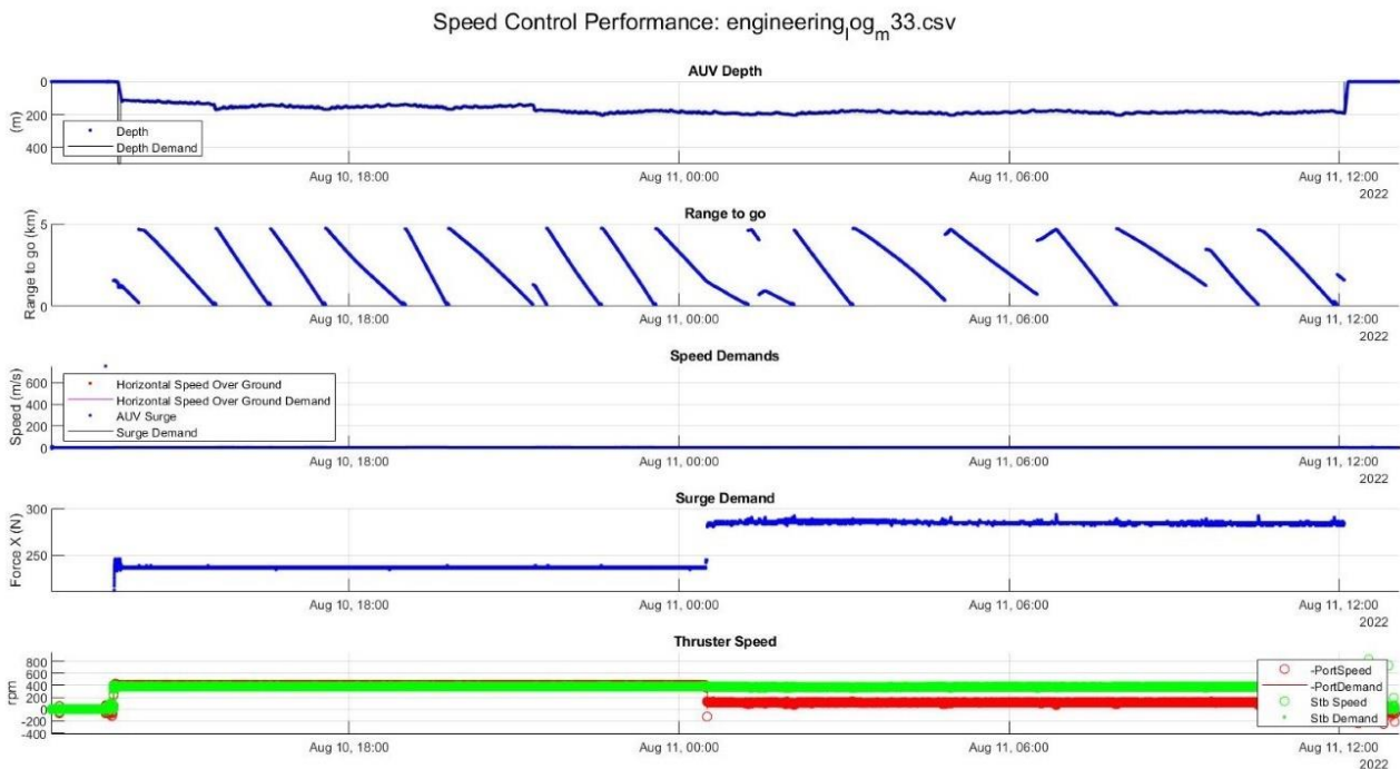
Fig. 7.24 Speed control performance during A5M33
