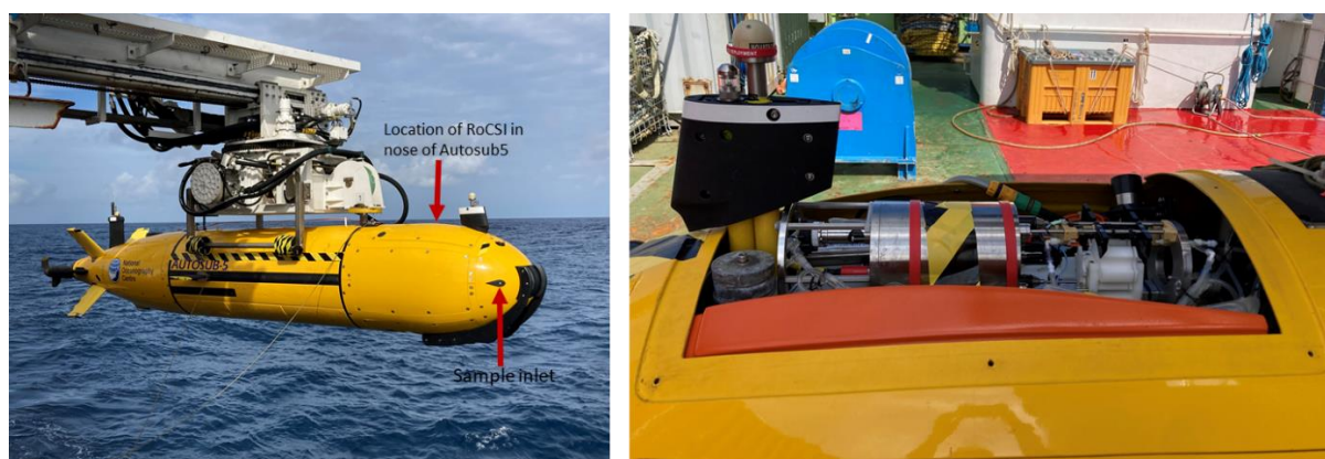
Fig. 6.87 RoCSI in the nose of Autosub5
