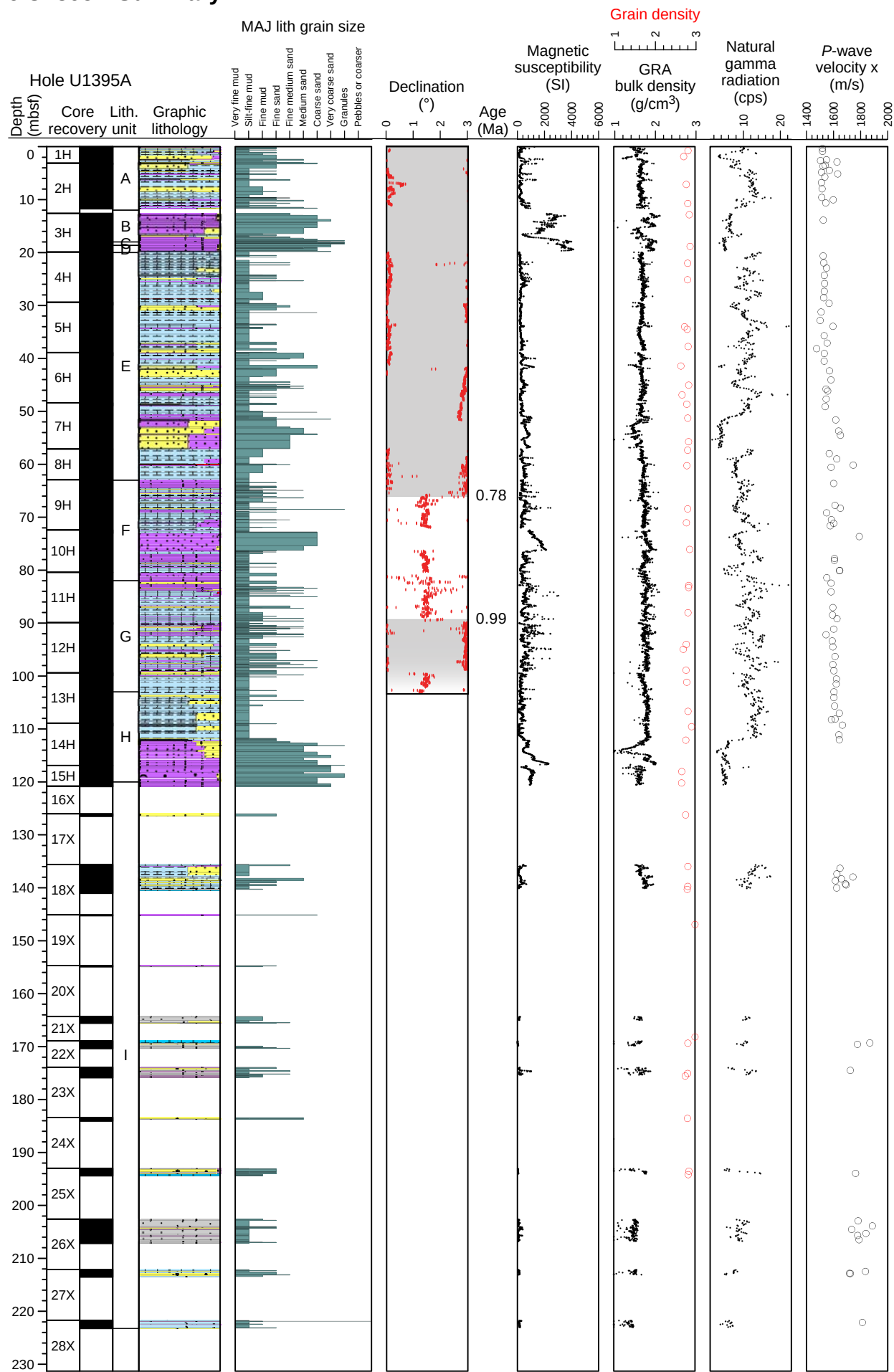
Figure F8. Hole U1395A summary. MAJ = major, GRA = gamma ray attenuation, cps = counts per second. See Figure F5B for graphic lithology key.
