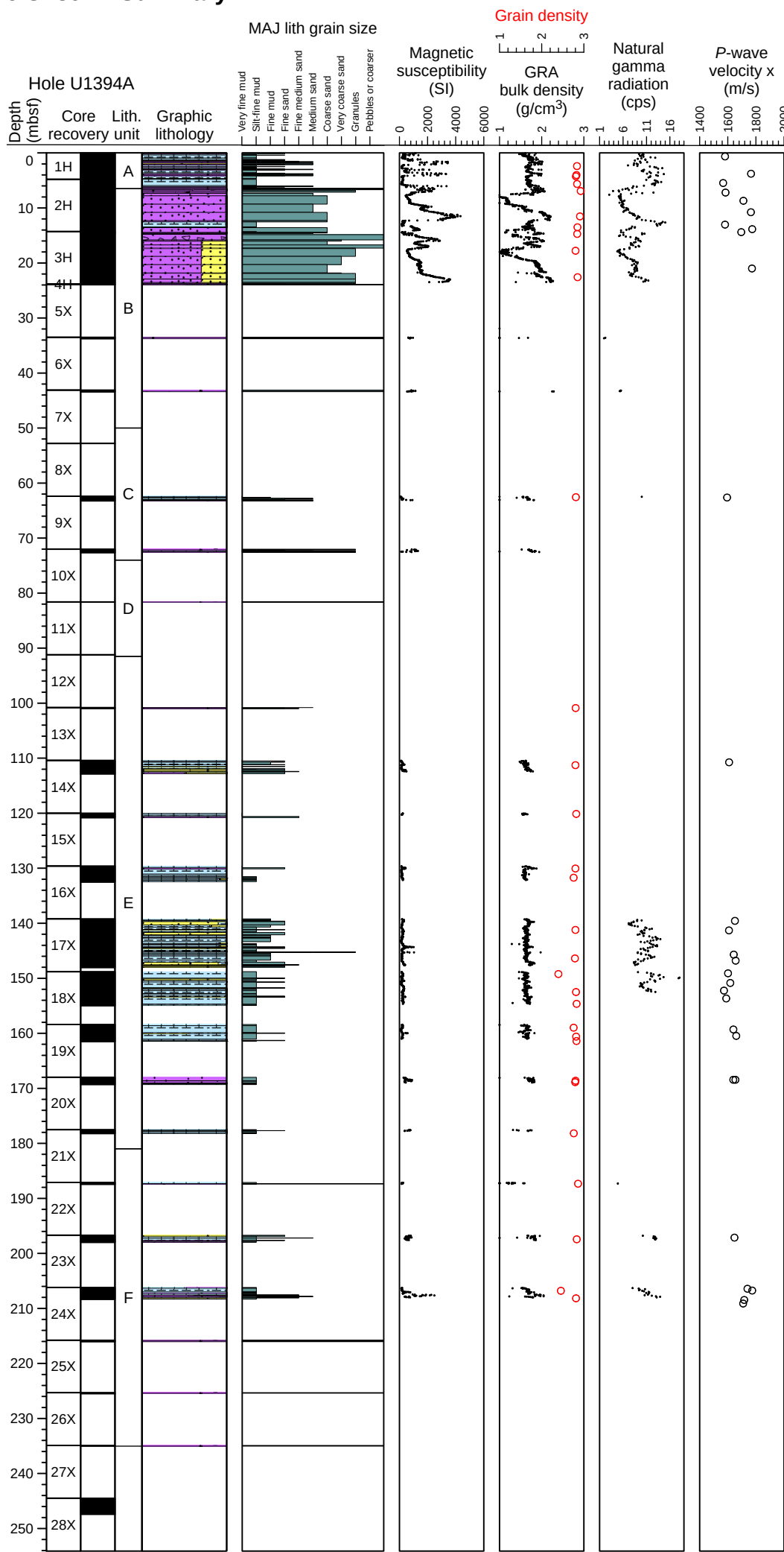
Figure F6. Hole U1394A summary. MAJ = major, GRA = gamma ray attenuation, cps = counts per second. See Figure F5B for graphic lithology key.
