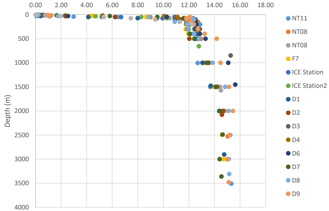
Figure 3.7: Nitrate + nitrite (uM/l)
