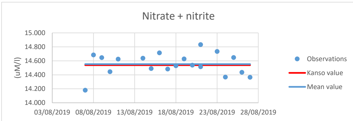
Figure 3.3: Analysis of KANSO Batch CI Standard Reference material, Nitrate + nitrite results.
