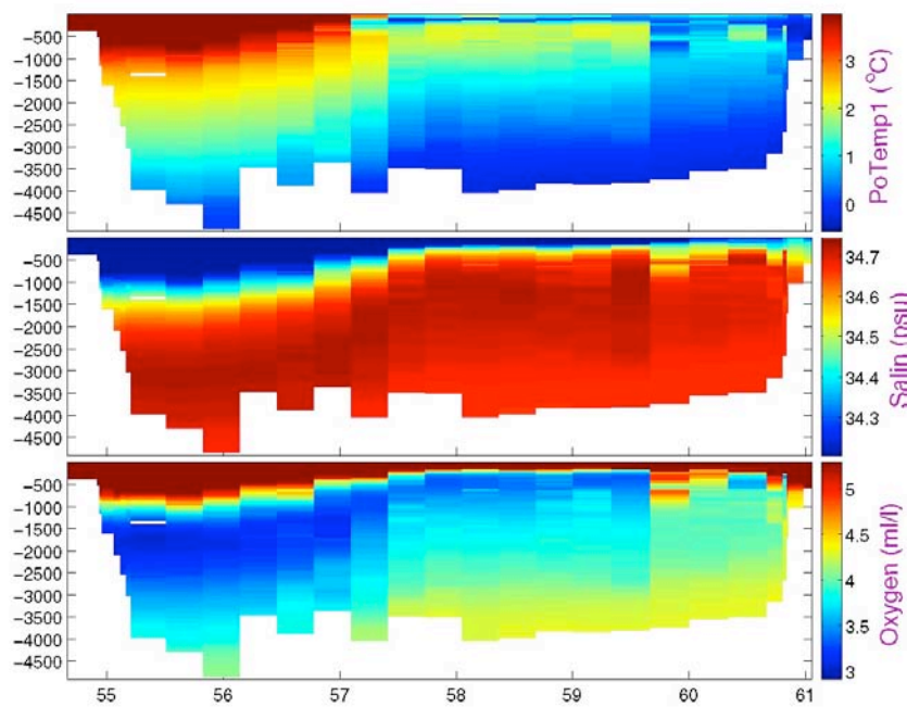
Figure 2.2: Plot of potential temperature ( ^{\circ}\text{C} ), salinity and oxygen concentration) for Drake Passage section of JR194.
