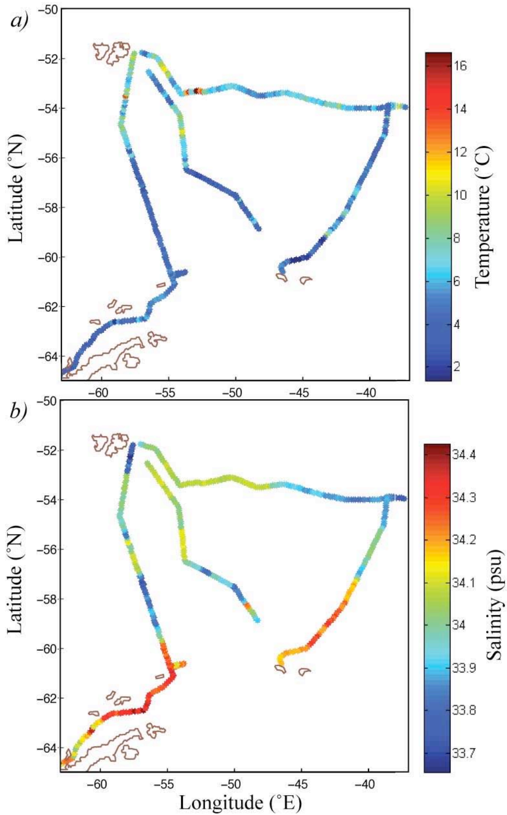
Figure 8.2: Physical surface parameters in the southern S. Atlantic, from the combined JR187 and JR194 cruises; a) Temperature; b) Salinity.
