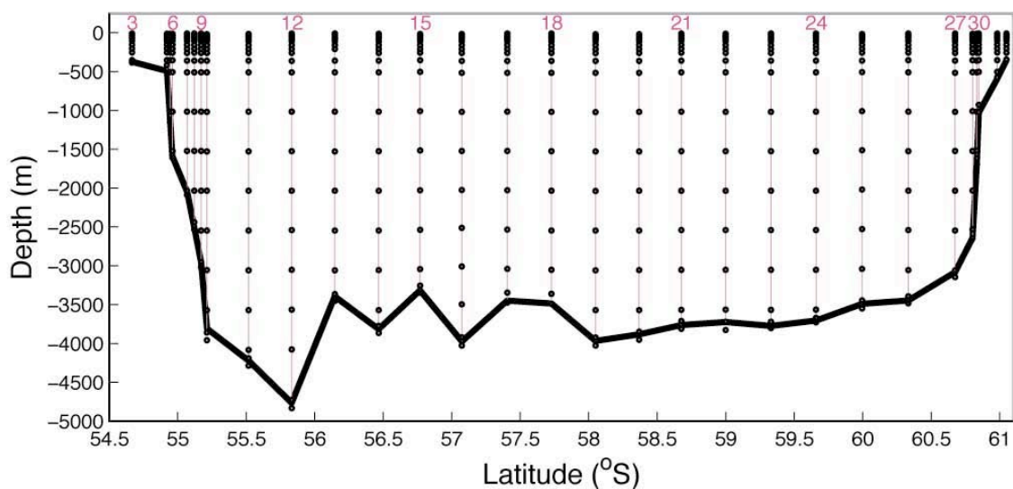
Figure 2.1: Depths of CTD bottle firing. Note the bathymetry profile is from the echo sounder (estimated in m), whereas values shown for bottles are pressure (in db), hence the fact that some bottles appear to be below the seabed. In most cases, the bottom bottle is 5-10 m above the bottom (according to the altimeter).
