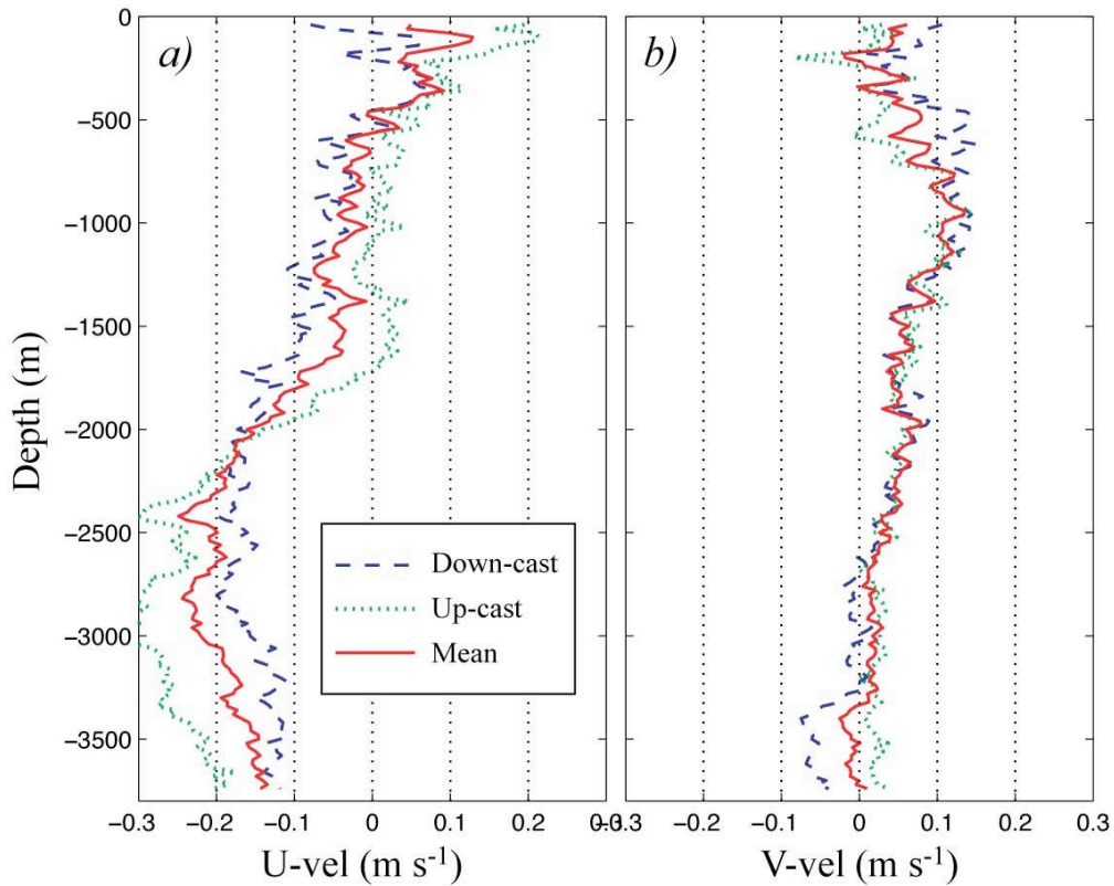
Figure 4.1: Vertical profiles of LADCP-derived velocity at CTD station 23 (depth 3775m); a) Eastward component; b) Northward component.
