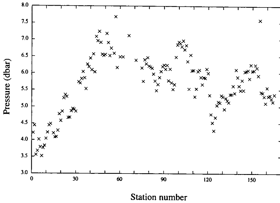
Figure 2.2: Uncorrected CTD deck pressures.
