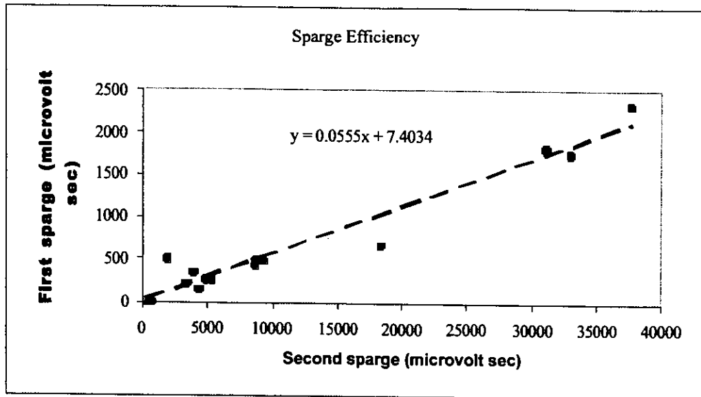
Figure 2.8: Sparge efficiency.
