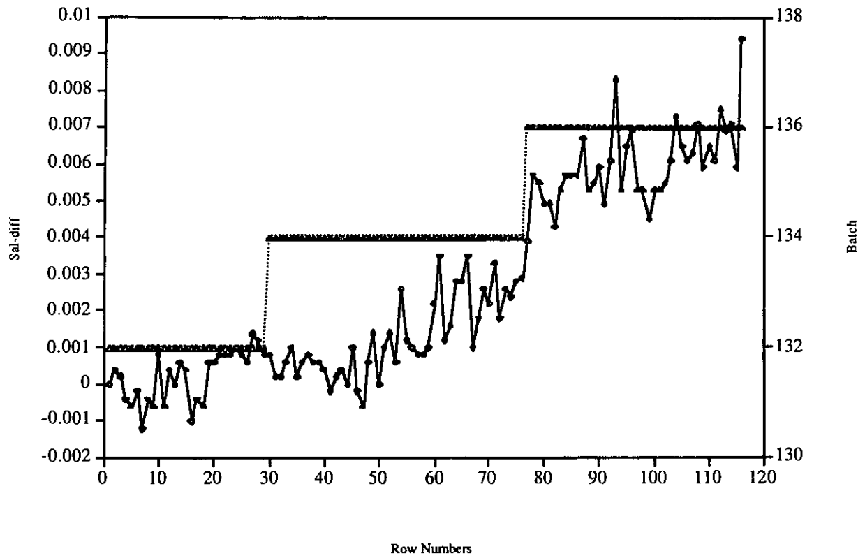
Figure 2.10: Guildline salinometer 8400B standardisation history. Three different standard seawater batches were used, P132, P134 and P136.
