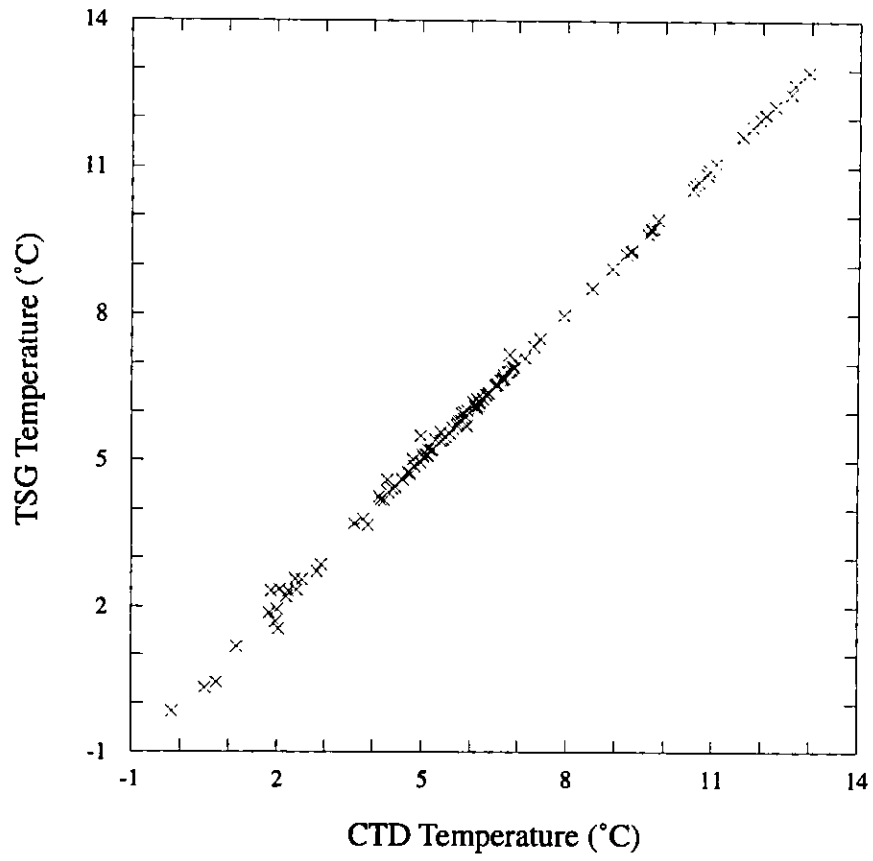
Figure 3.1: Thermosalinograph temperature versus CTD temperature at a depth of 7 m (7 dbar).
