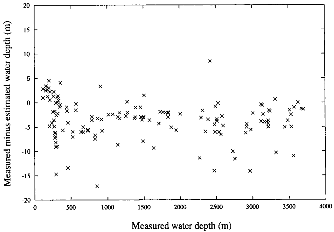
Figure 2.4: Difference between measured (echo sounder) and estimated (CTD plus altimeter) water depth.
