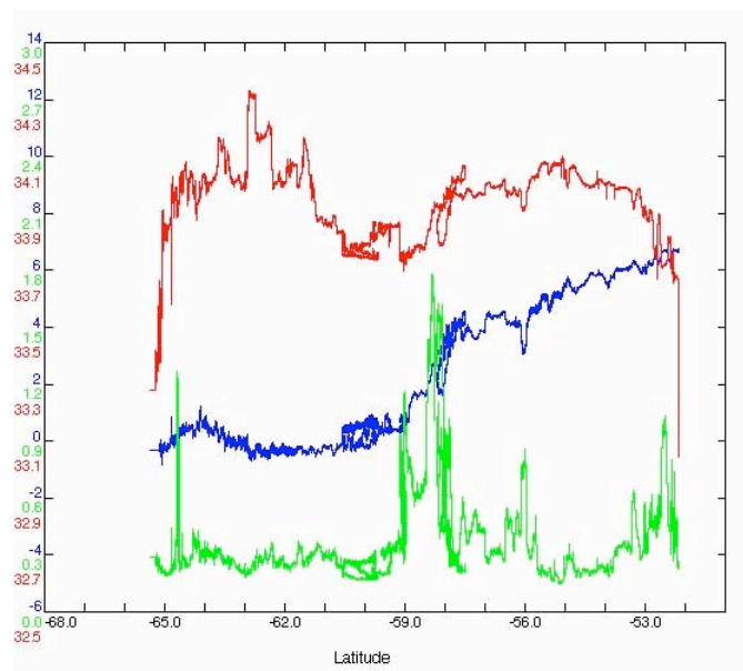
Figure 7.6: Latitudinal variability in surface ocean characteristics (southbound leg). Sea surface temperature ( ^{\circ}\text{C} ) is illustrated in blue, fluorescence ( \mu\text{g}\cdot\text{l}^{-1} ) in green, and salinity in red.
