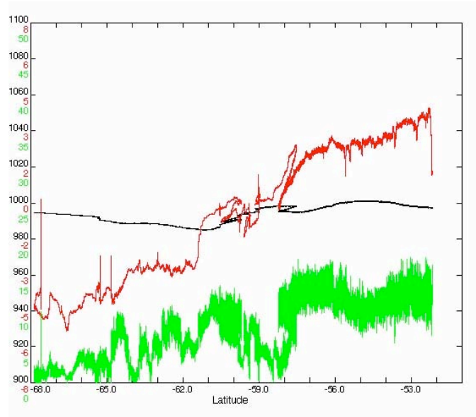
Figure 7.7: Latitudinal variability in meteorological characteristics (southbound leg). Air pressure (mbar) is illustrated in black, air temperature ( ^{\circ}\text{C} ) in red, and true wind speed ( \text{m!s}^{-1} ) in green.
