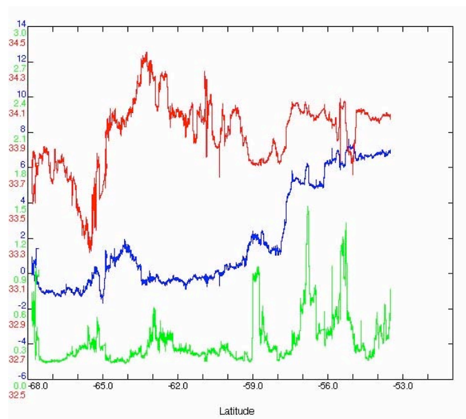
Figure 7.4: Latitudinal variability in surface ocean characteristics (northbound leg). Sea surface temperature ( ^{\circ}\text{C} ) is illustrated in blue, fluorescence ( \mu\text{g l}^{-1} ) in green, and salinity in red.
