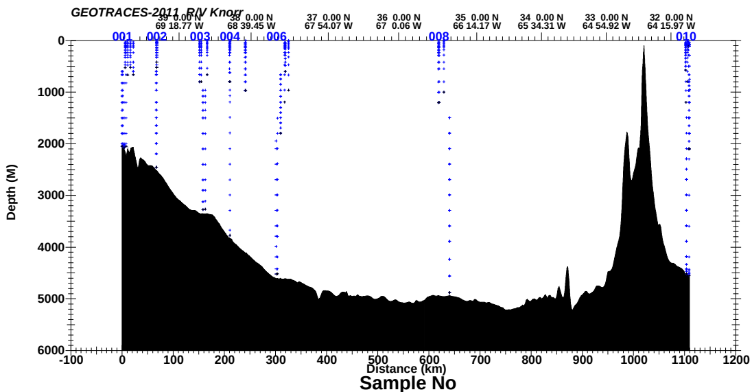
Figure 1.0 GEOTRACES 2011 Sample distribution, Leg 1: stations 1-(10).
