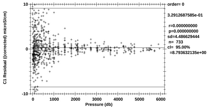
Figure 1.6.3.9 SIOR Corrected C_{\text{Bottle}} - C1 by pressure ( -0.01^{\circ}\text{C} \leq T1 - T2 \leq 0.01^{\circ}\text{C} ).
