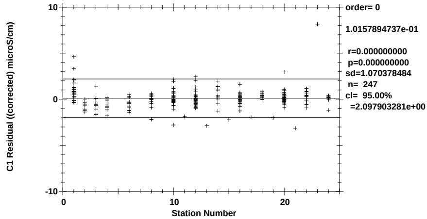
Figure 1.6.3.7 SIOR Deep Corrected C_{\text{Bottle}} - C1 by station (Pressure \geq 1000 dbar).
