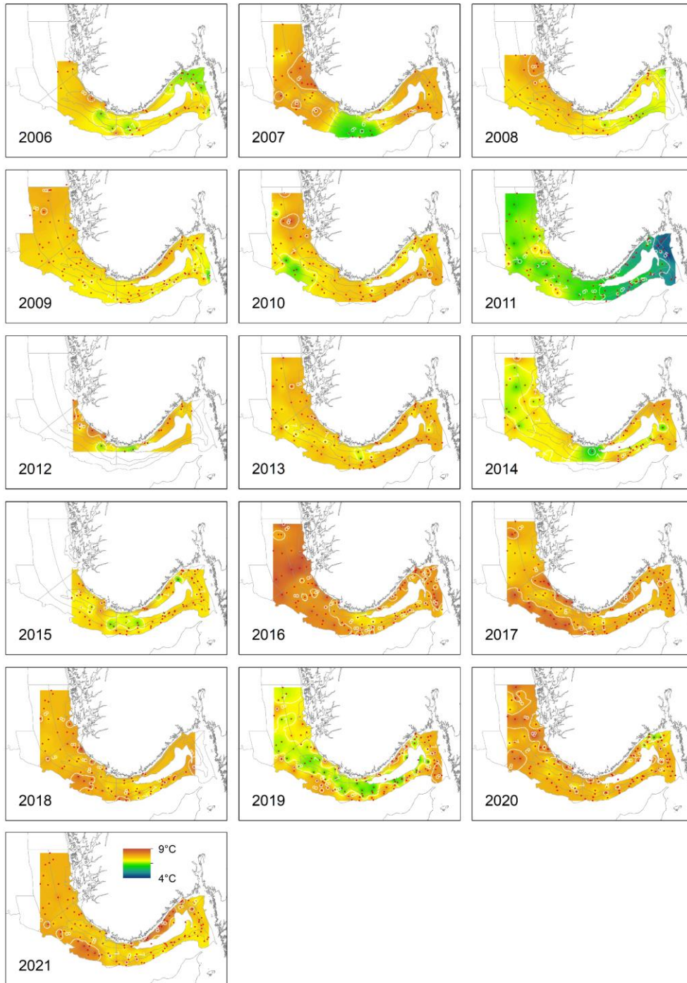
Figure 5. Bottom temperatures (°C) from CTD from the Norwegian shrimp survey in 2006-2021 in ICES Divs. 3.a and 4.a East (Skagerrak and the Norwegian Deep). The 2012 data result from only 22 CTD hauls (8 in the Norwegian Deep and 14 in Skagerrak) due to difficulties with the CTD-winch. Red points show CTD stations.
