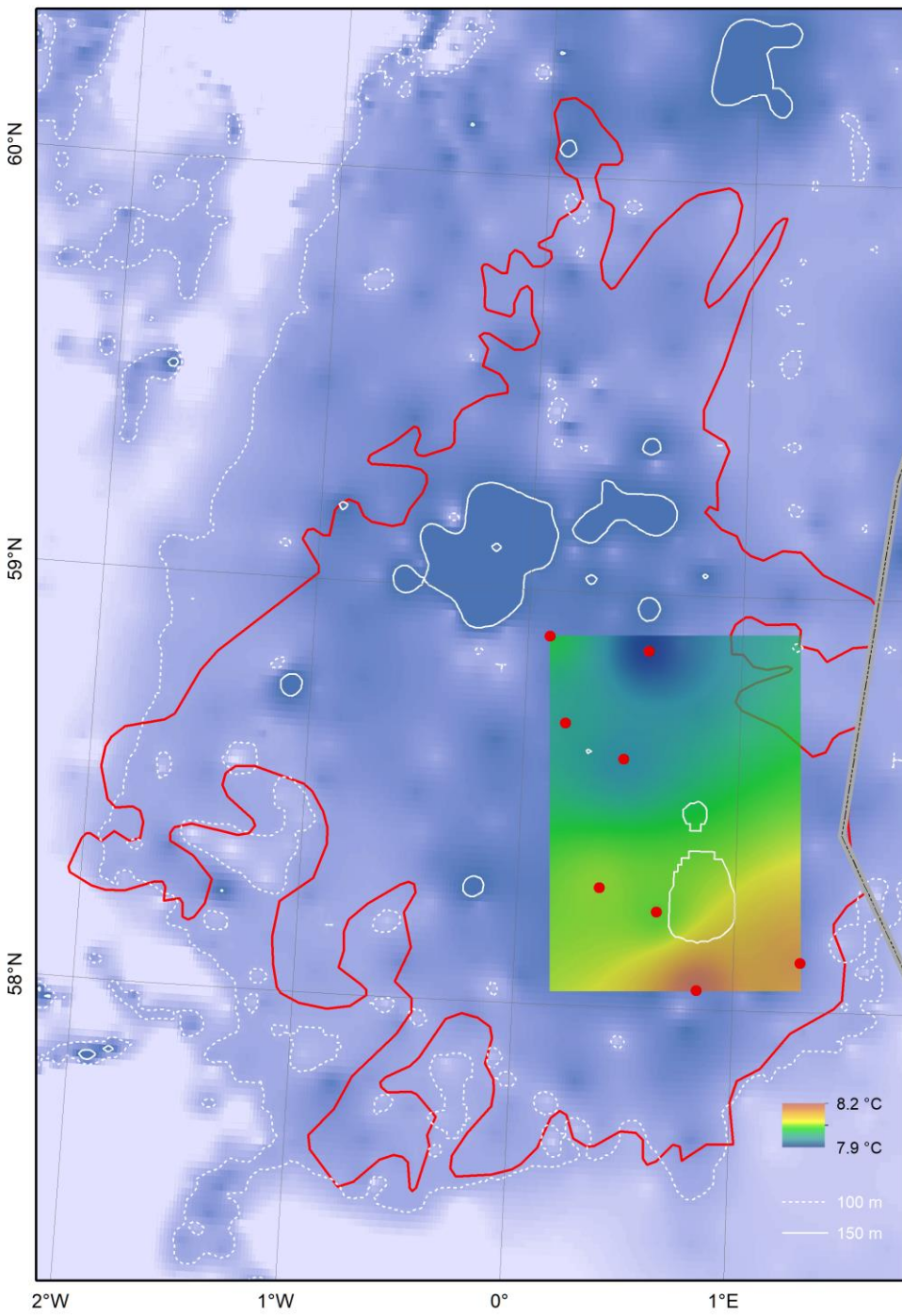
Figure 7. Bottom temperatures (°C) from CTD in the 2021 survey in ICES Div. 4.a west (the Fladen Ground). Red points show CTD stations.
