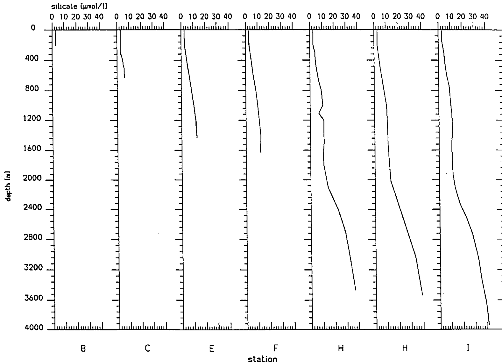
Fig. 42 Winter distribution of silicate along the Goban Spur transect (for notation of stations see Fig. 40).
