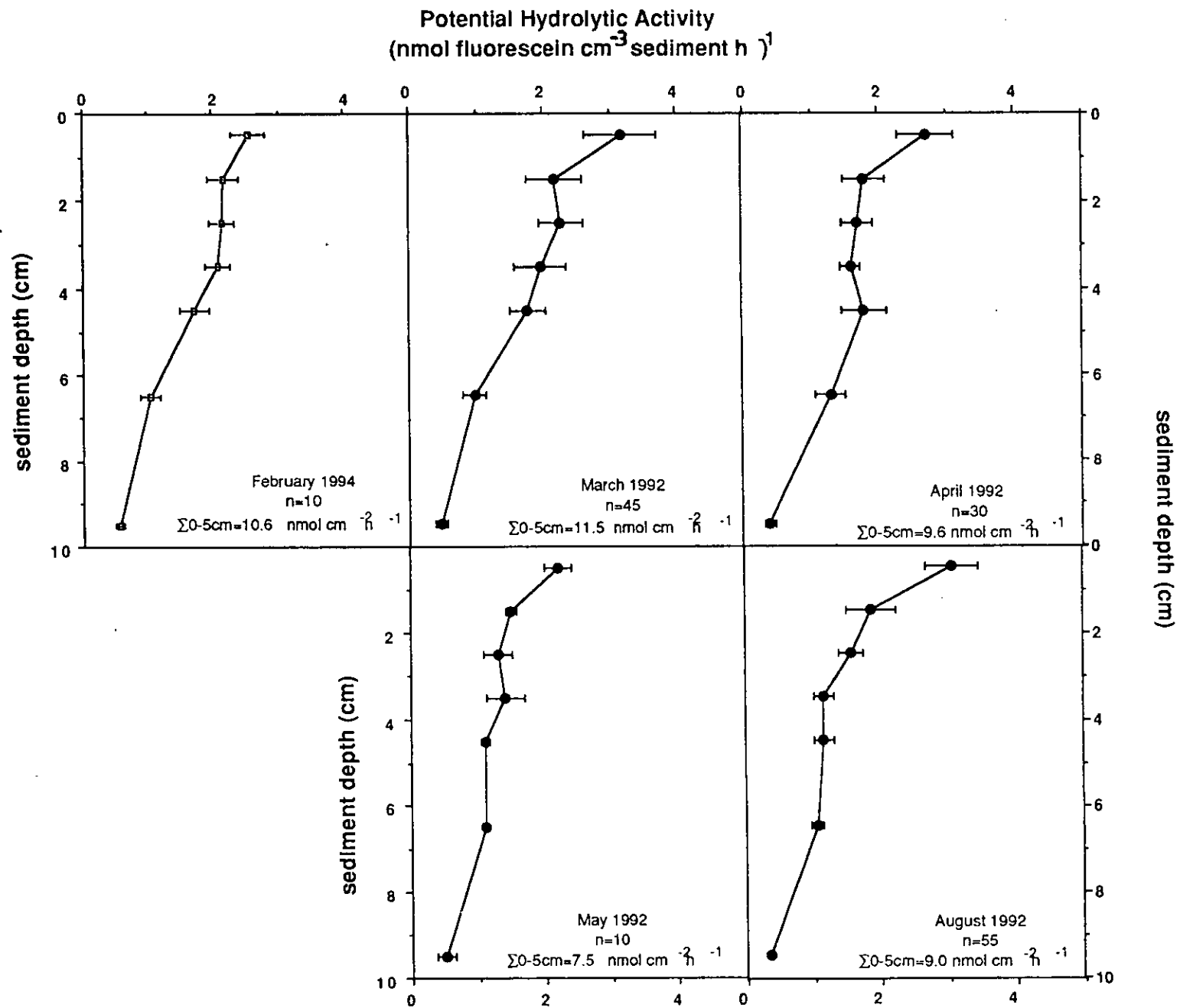
Fig. 53: Benthic activity (FDA reduction rates) at the BIOTRANS-station.
