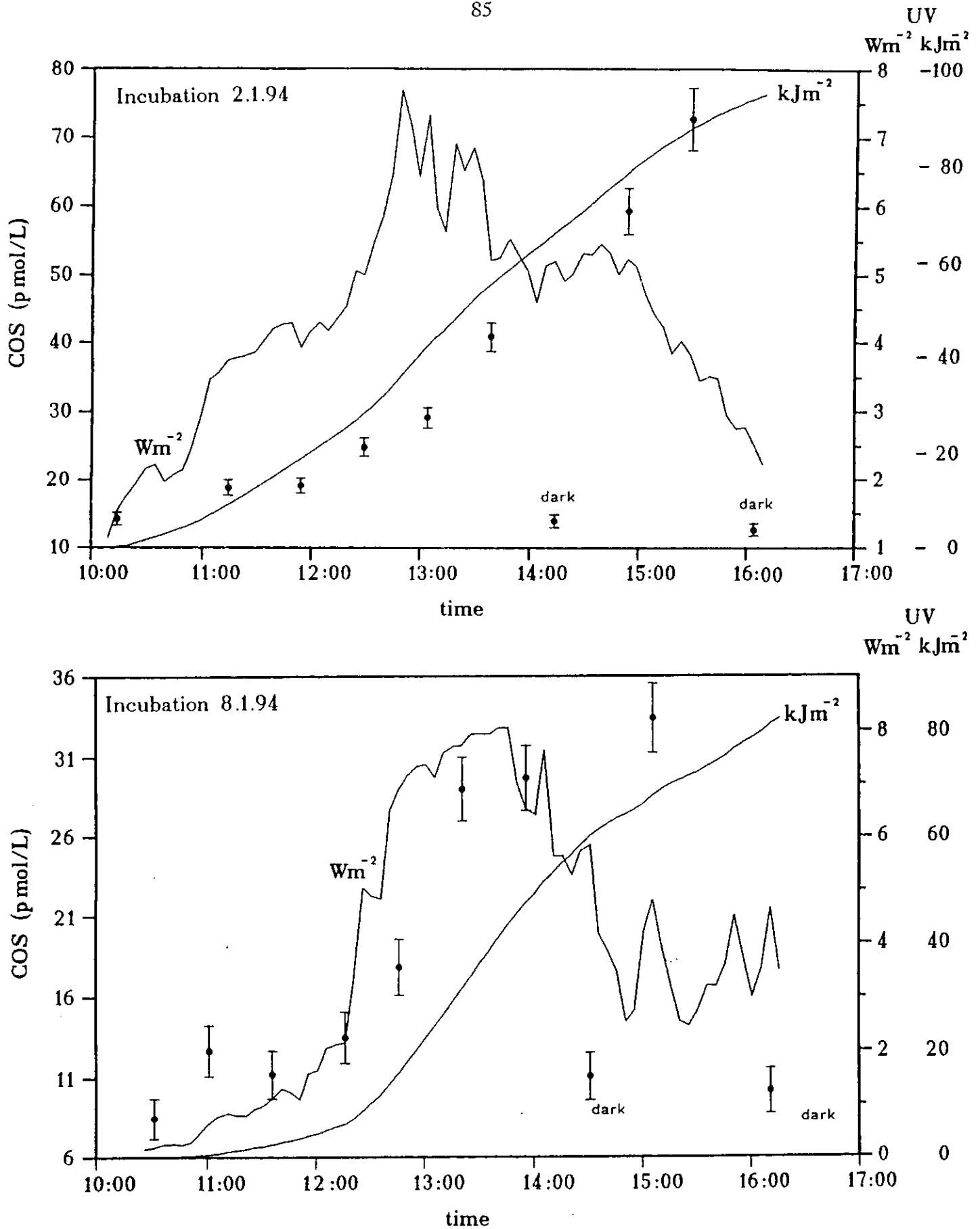
Fig. 48: COS photo-production correlated with the total incident UV sun light energy. Dark controls show little or no increase in COS concentration. Time scale is local time. Sun rise and sun set can be estimated from the UV light intensity curve.
