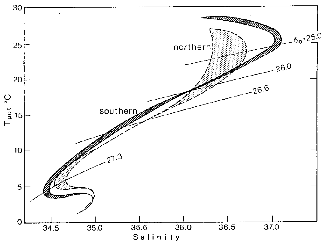
Fig. 14a: Northern and southern water mass contrast \theta S diagram for stations 8-12, along 44°W, (Fig.2) and stations 79-82 along 5°S near the coast.
