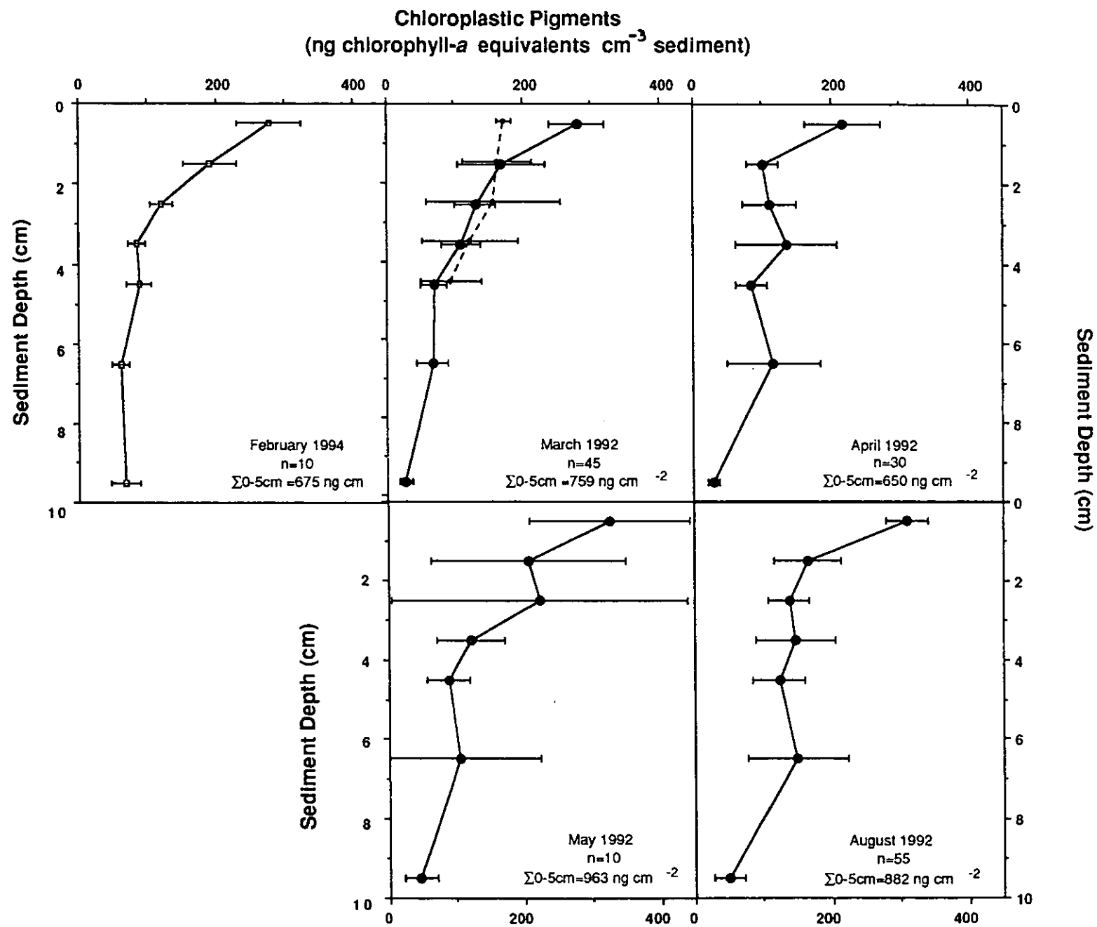
Fig. 52: Sediment bound chloroplastic pigments at the BIOTRANS-station.
