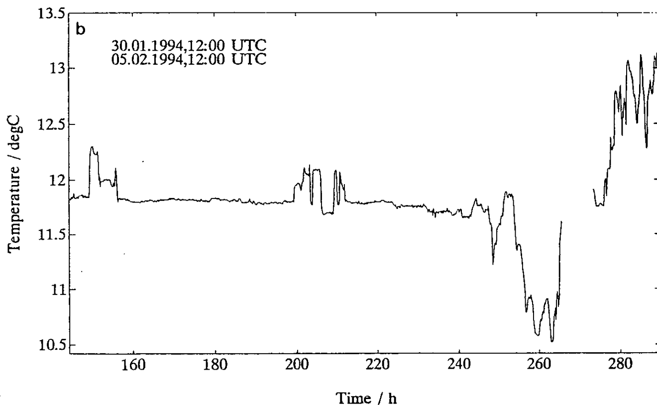
Fig. 13a: Time series of sea surface temperature registrated by thermosalinograph-sensor from January 30, 1994, 12:00 UTC to February 05, 1994, 12:00 UTC.
