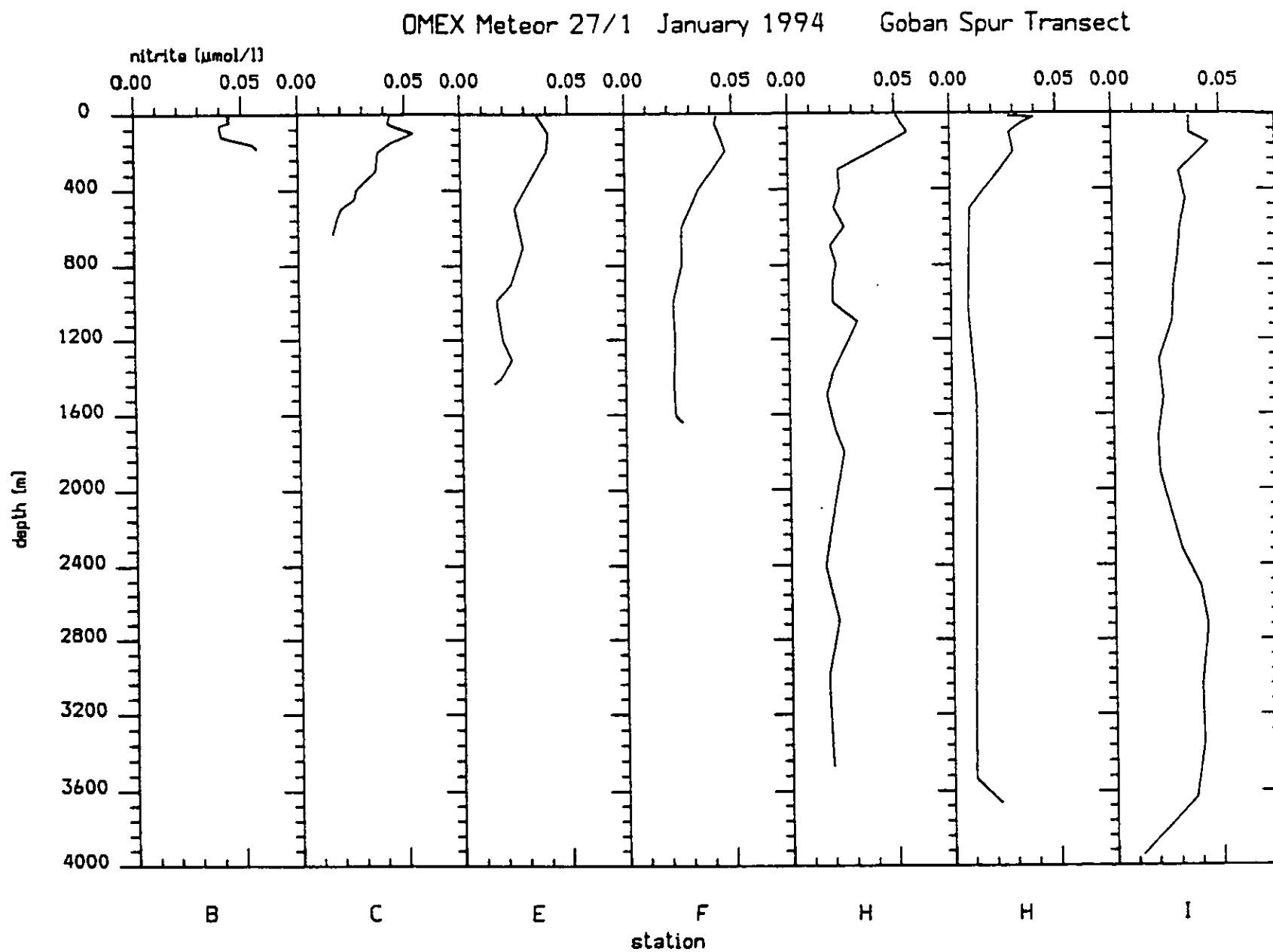
Fig. 44: Winter distribution of nitrite along the Goban Spur transect (for notation of stations see Fig. 40).
