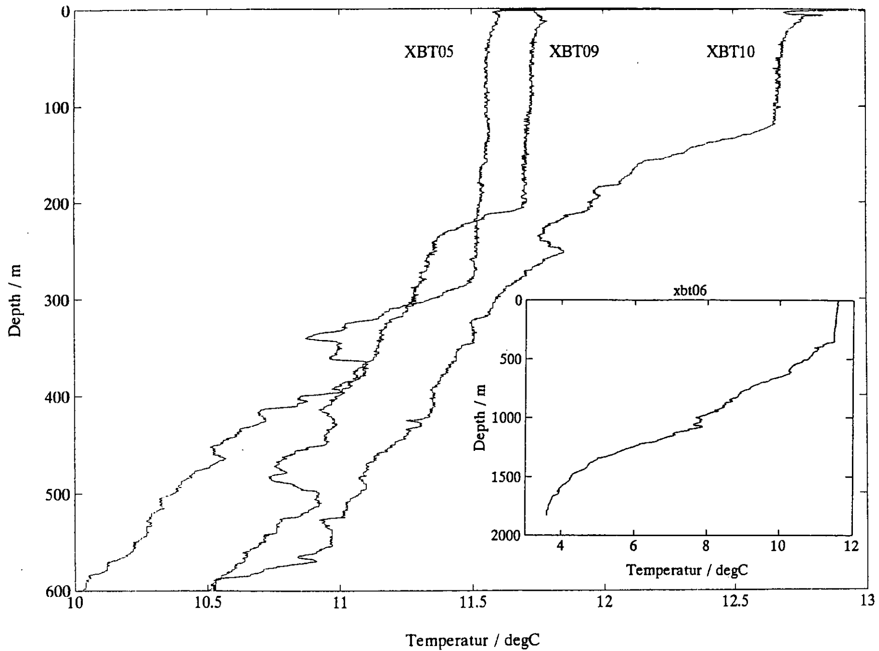
Fig. 11: The upper 600 m of selected temperature profiles versus depth measured by XBT drops during M 27/2. (XBT drops no. 5,9, and 10). Subplot of XBT no. 6.
