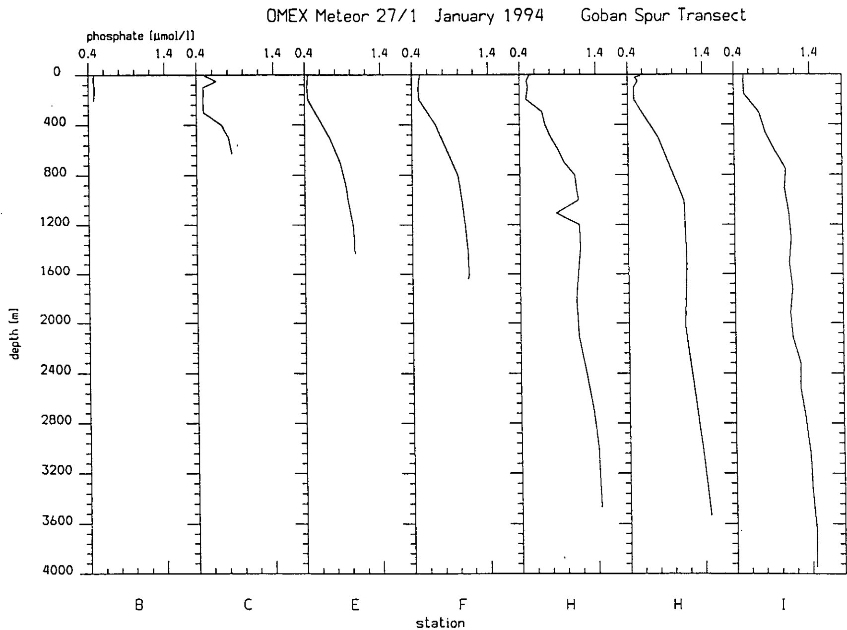
Fig. 41: Winter distribution of phosphate along the Goban Spur transect (for notation of stations see Fig. 40).
