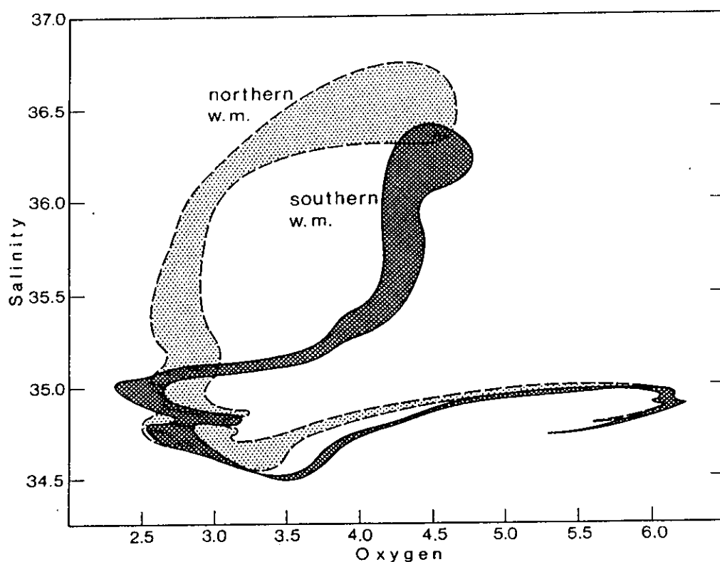
Fig. 14a: Northern and southern water mass contrast S/O 2 diagram for stations 8-12, along 44°W, and stations 60-64 along 35°W near the equator.
