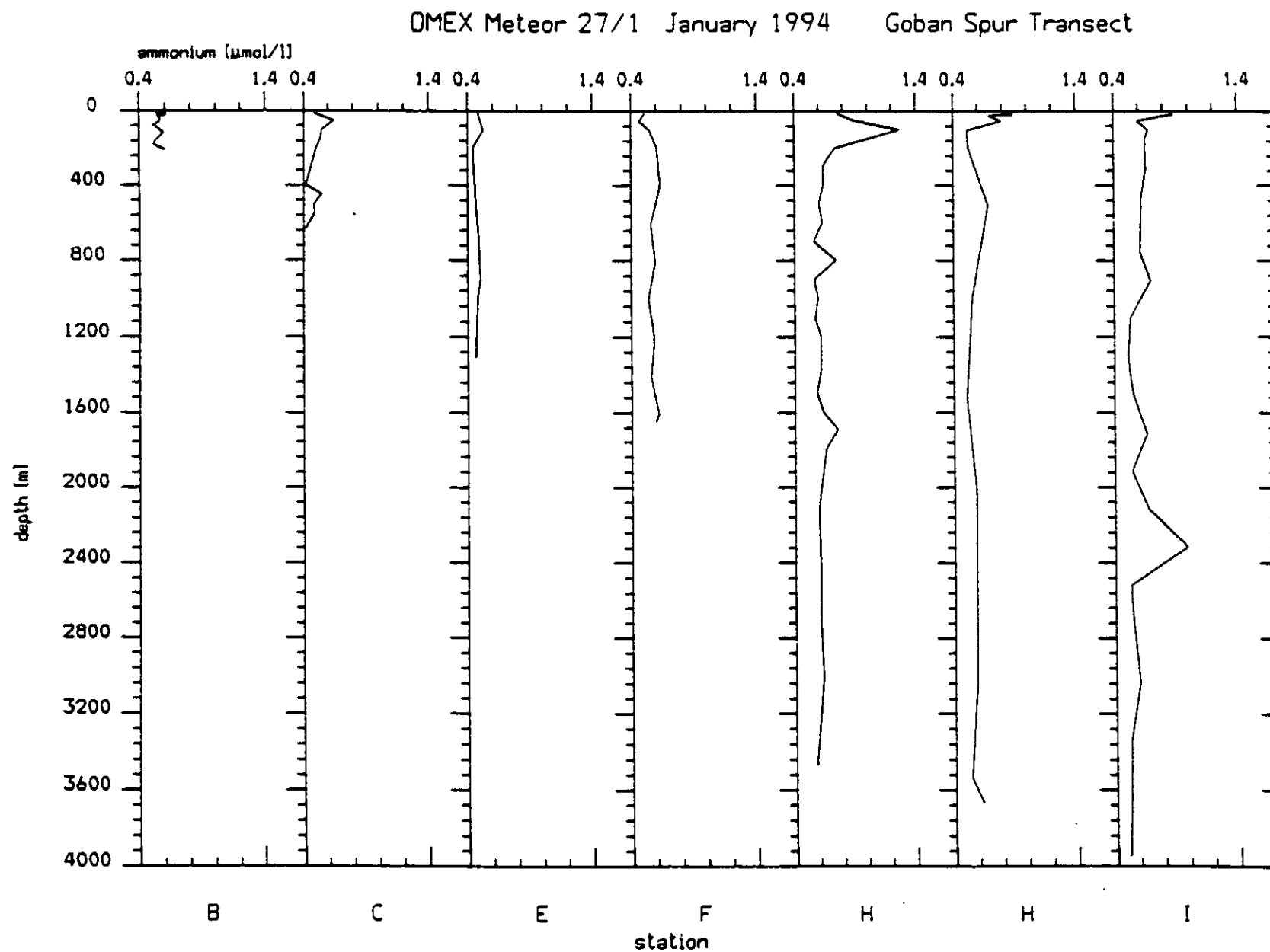
Fig. 43: Winter distribution of ammonium along the Goban Spur transect (for notation of stations see Fig. 40).
