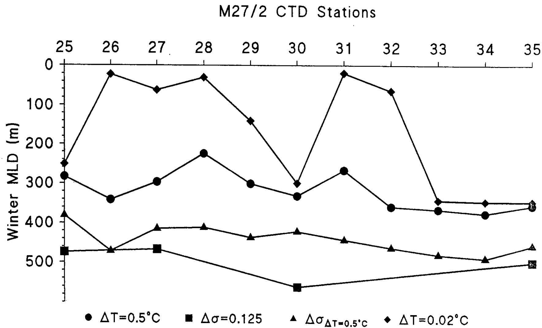
Fig. 7: Depths of the winter mixed layer calculated by different methods for stations 25 to 35 taken before storm event. The circles mark delta temperature 0.5^{\circ}\text{C} , the squares the delta sigma-t 0.125, the triangles the delta sigma depend from delta temperature 0.5^{\circ}\text{C} , and the rhombus the delta temperature 0.02^{\circ}\text{C} criterion.
