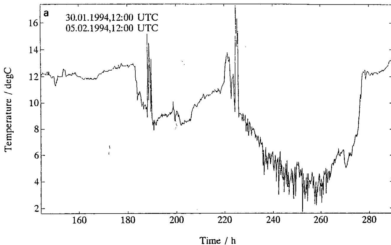
Fig. 13a: Time series of air temperature registrated by shipborn sensors from January 30, 12:00 UTC to February 05, 1994, 12:00 UTC.
