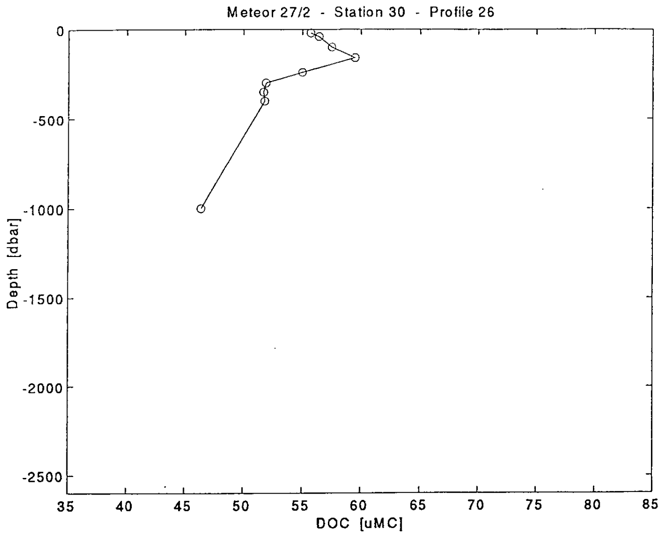
Fig. 38: Depth profile of DOC at the BIOTRANS-site ( 47^{\circ}\text{N} / 20^{\circ}\text{W} , January 30, 1994), shallow mixed layer.
