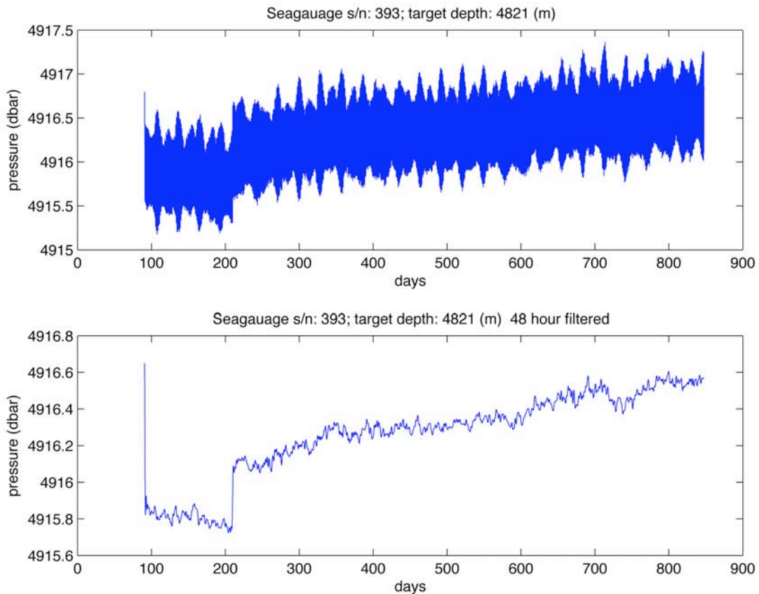
Figure 12.3 The original data record from the BPR at wbl2_2_200706
