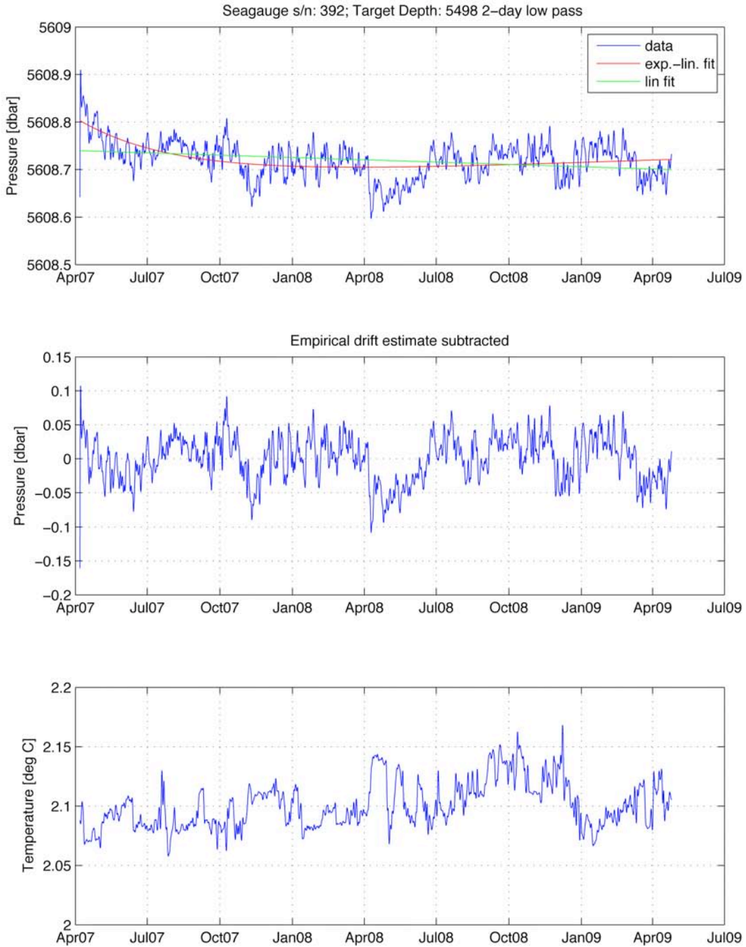
Figure 12.2 The output from the stage 2 processing of wb6_1_200707. Fig 12.2a shows the raw data with the ends removed; Fig 12.2b shows the bottom pressure with the exponential-linear drift removed. Fig 12.2c is the temperature curve.
