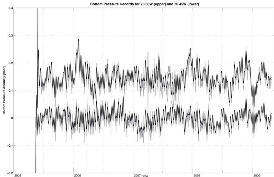
Figure 12.8 The combined bottom pressure records for 76^{\circ} 45'W (lower) and 76^{\circ} 03'W (upper), with a 10-day low pass filter applied to their mean values shown in black. The upper
