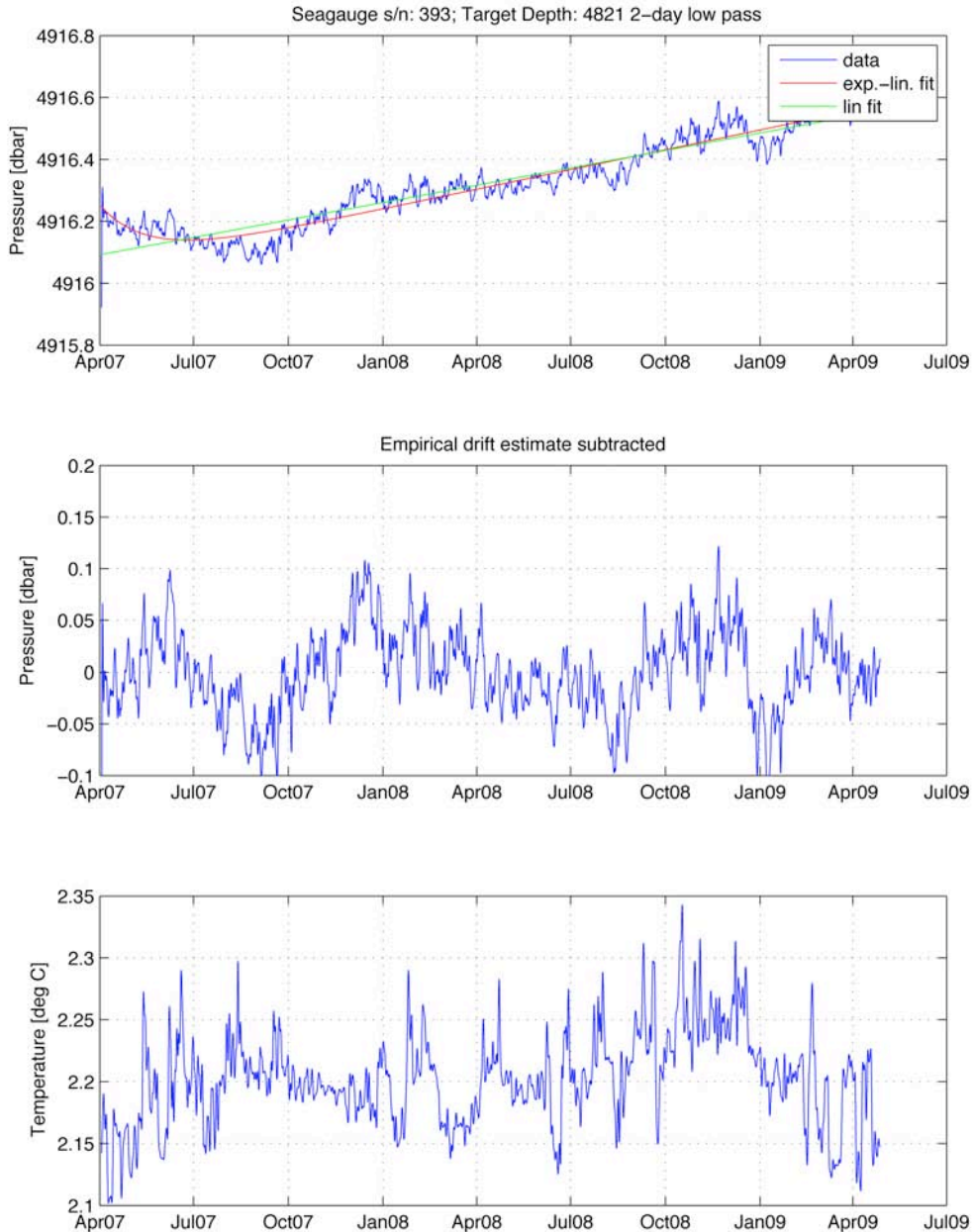
Figure 12.4 The ‘corrected’ plot for the BPR at wbl2_2_200706
