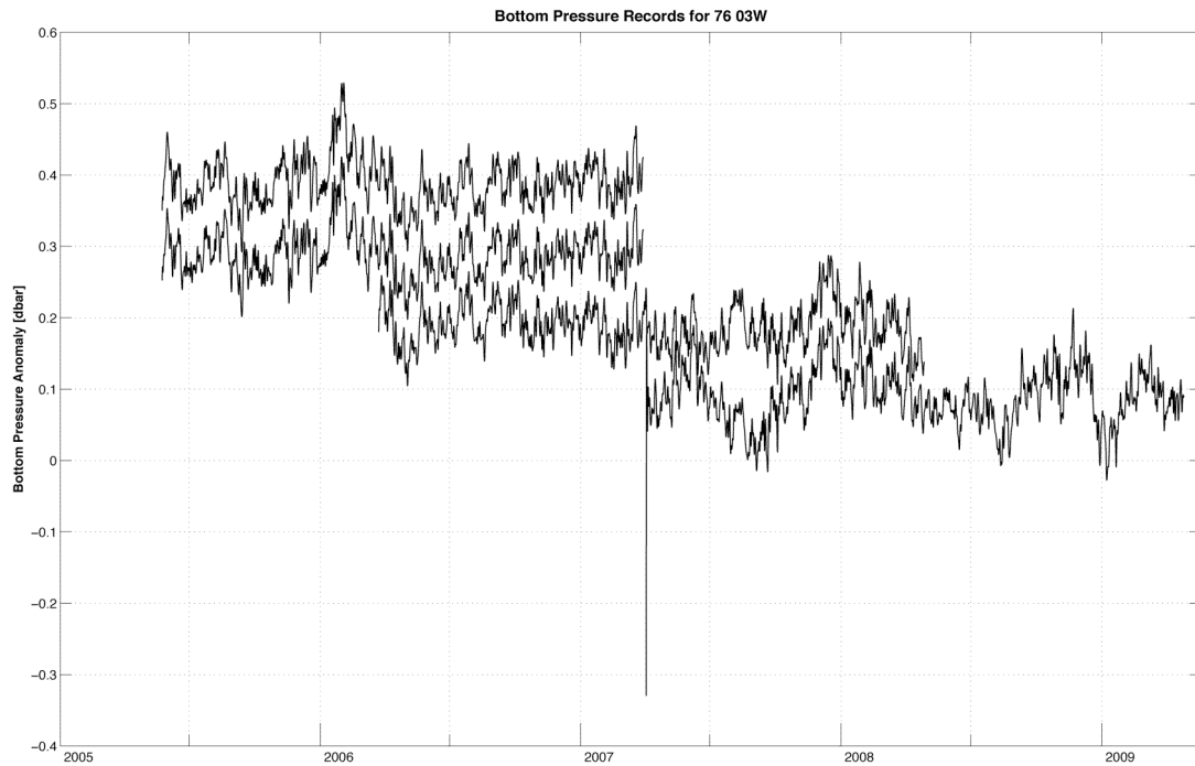
Figure 12.7 Combined plots of the time series for the bottom pressure anomalies at 76^{\circ} 03'W . The data that is widely separated is the corrected BPR from wbl2_2_200706. The curves are offset for visibility.
