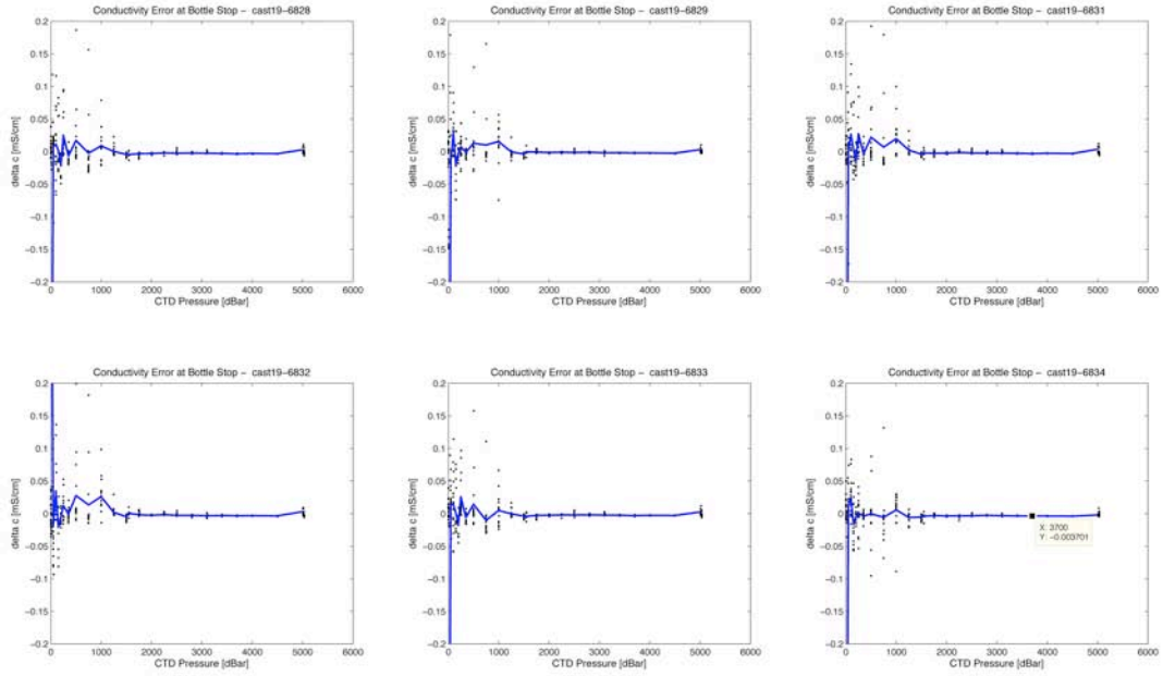
Figure 10.6 Conductivity errors during the bottle stops on cast 19, \Delta C = C - C_{CTD}
