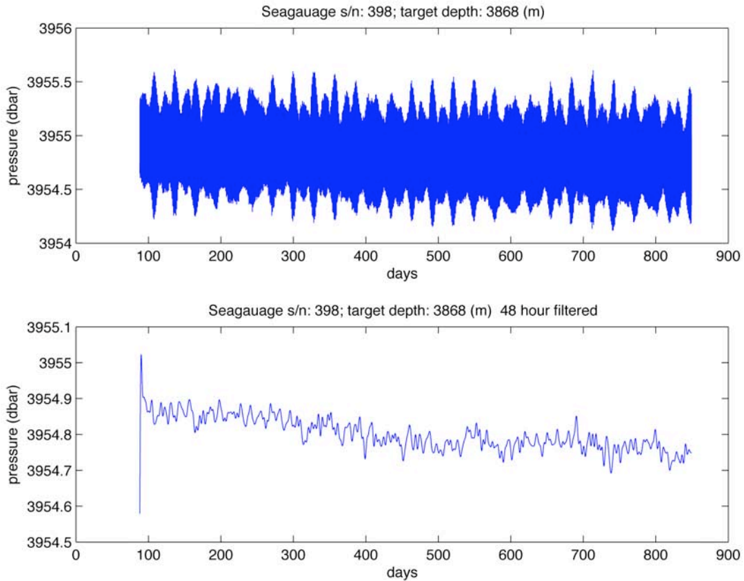
Figure 12.1 Initial output from wbl1_2_200705_0398.raw. Fig 12.1a – raw data, Fig 12.1b - data after the 48-hour low pass filter has removed the tidal effects.
