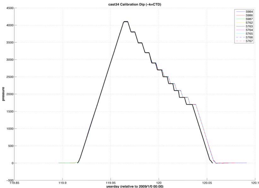
Figure 10.10 Cast 34 showing the very large timing errors.
