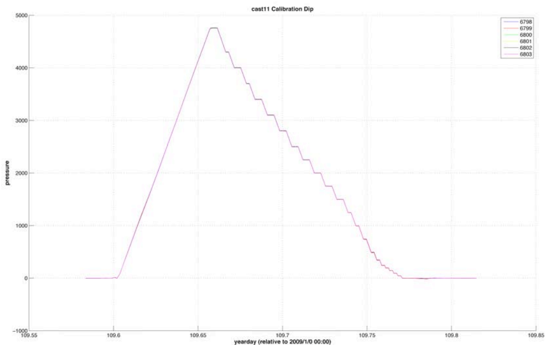
Figure 10.4a A plot of the pressure calibration cast11 from RB0901. The flat steps are the bottle stops.
