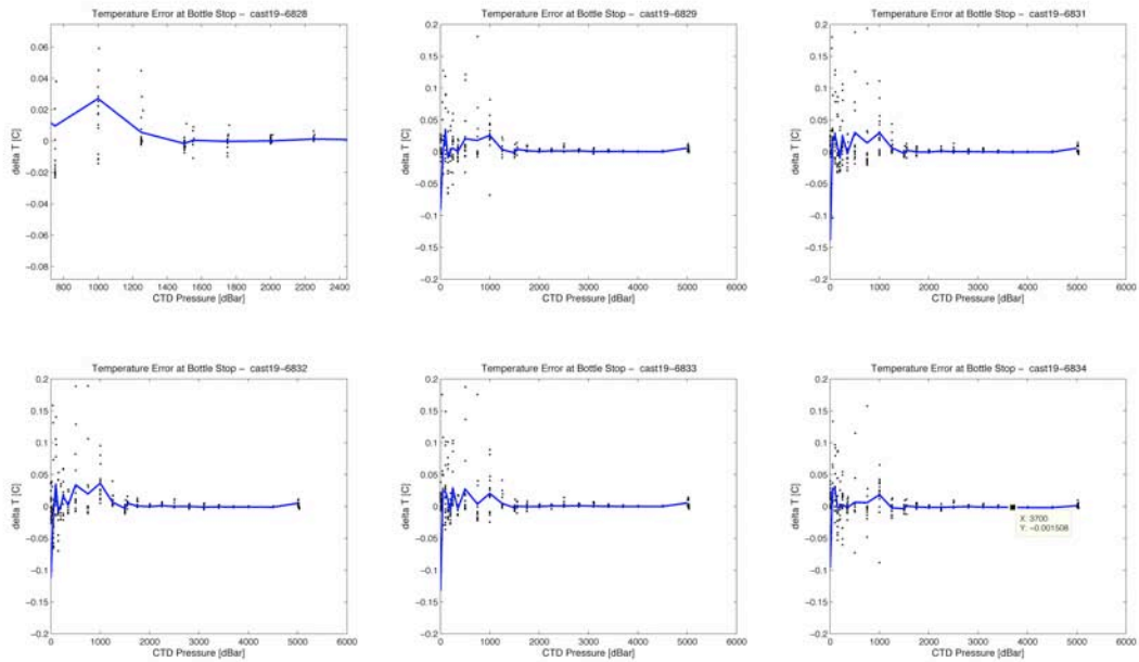
Figure 10.7 Temperature errors during the bottle stops on cast 19, \Delta T = T - T_{CTD} . This is the fast response temperature sensor and not the thermistor associated with the pressure sensor.
