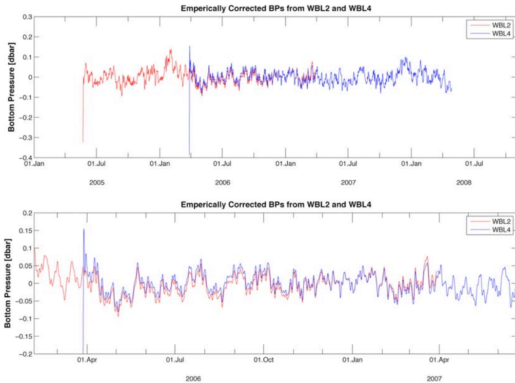
Figure 12.5 An example of the overlapping segments of two BPR records at 76° 45' W. The lower plot is the detail of the overlap. Moorings used were wbl2_1_200531_0392 and wbl4_1_200605_0004.
