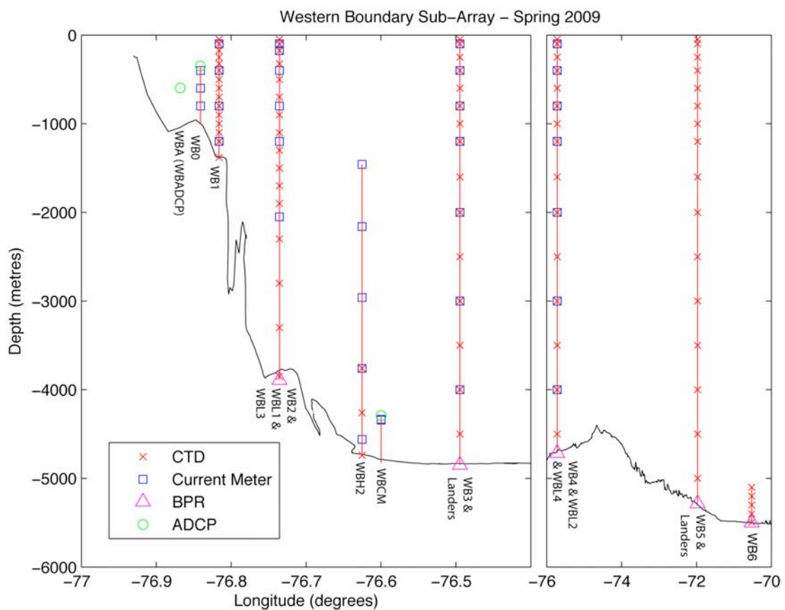
Figure 5.2 Western boundary sub_array as deployed on cruise RB0901.
