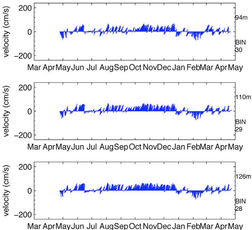
Figure 9.1 Quiver plots of bins 28, 29 and 30 of the wbadcp_5_200805 data.
