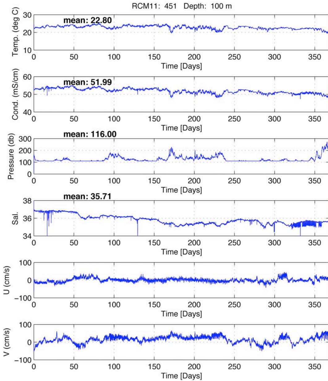
Figure 11.1 The output plot of stage 2 processing of the RCM11 data from wb2_6_200803
