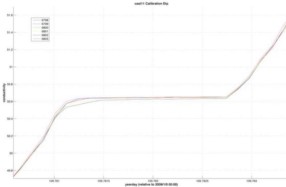
Figure 10.4b Detail of a conductivity calibration dip cast bottle stop.
