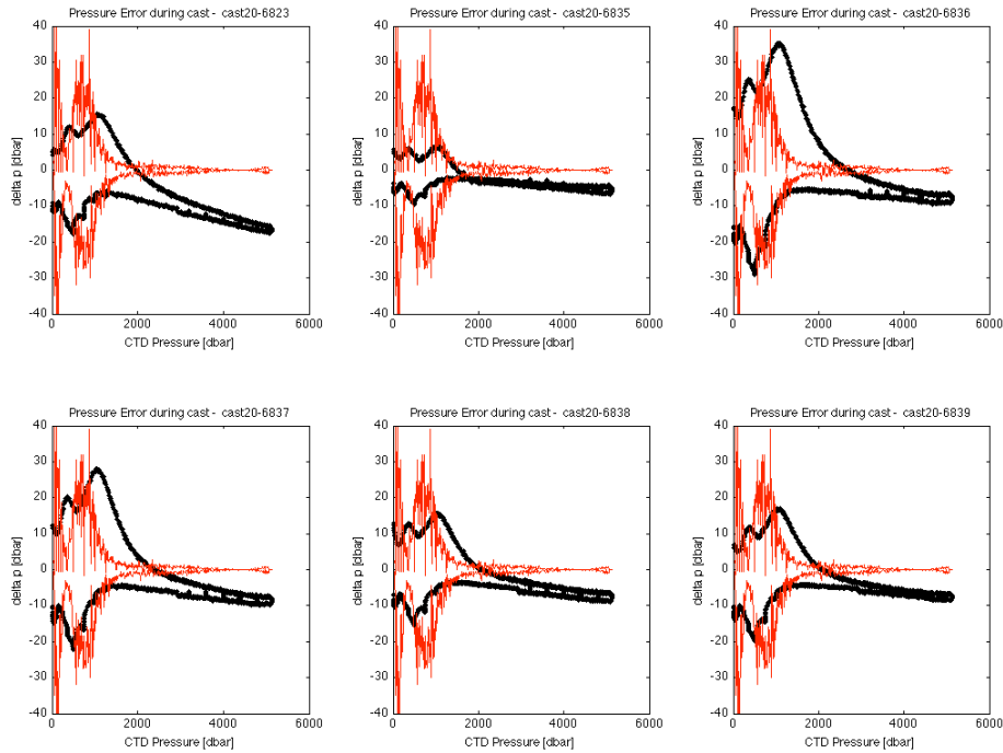
Figure 10.8 The pressure errors (black) for cast 20 with the rate of change of temperature superimposed in red. The dT/dt curves have been greatly exaggerated, by a factor of 1000, for visibility. \Delta p is generally positive on the downcast and negative on the upcast.
