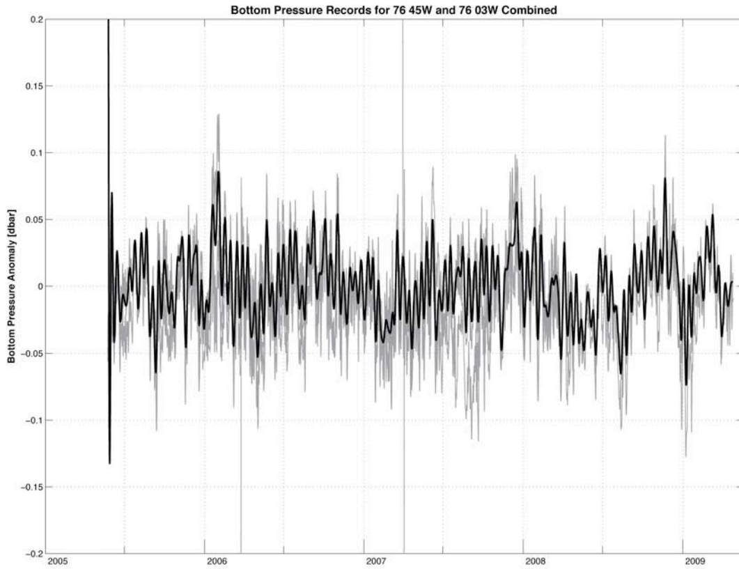
Figure 12.9 The combined bottom pressure records for the locations 76° 45'W and 76° 03'W, with a 10-day low pass filter applied to the mean value shown by the black curve.
