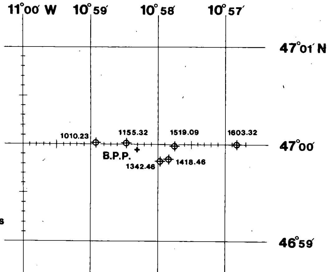
Drift of ship during Buoyant Programmed Pinger deployment, day 245 .
