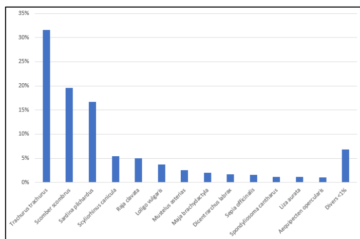
Figure 3b: Distribution of biomass dominance in the Eastern English Channel (>1%)
