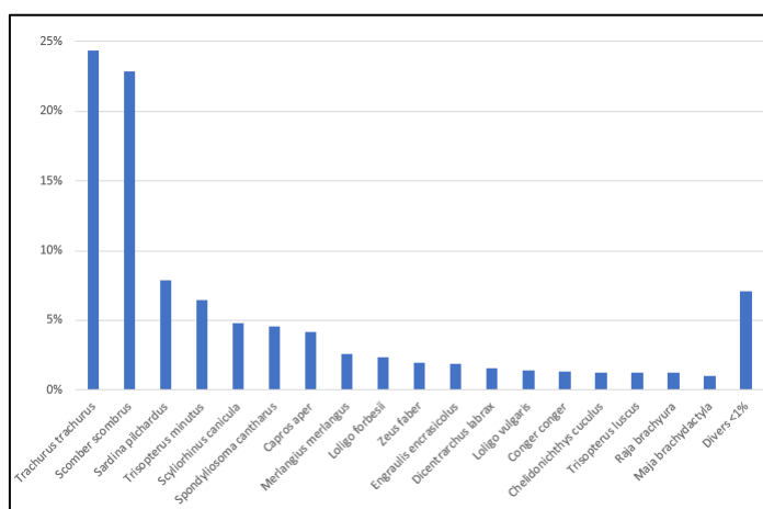
Figure 7b: Distribution of biomass dominance (>1%)
