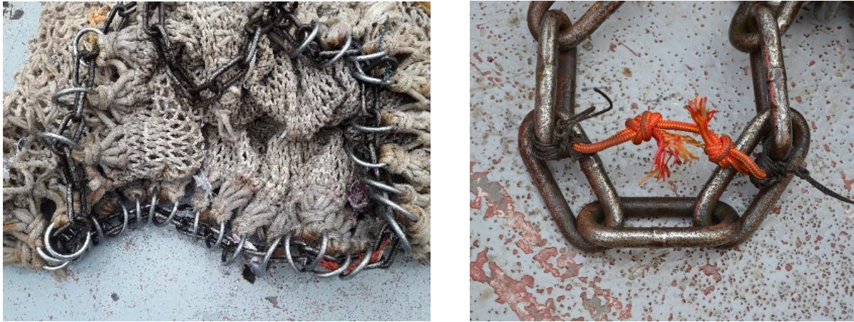
Figure 20 – Left: End of codend skirt showing the coupling chain fed through rings fixed to the netting. Right: Test twine set up as “weak-line” within a bight of chain [Source: J. Saltskår].
