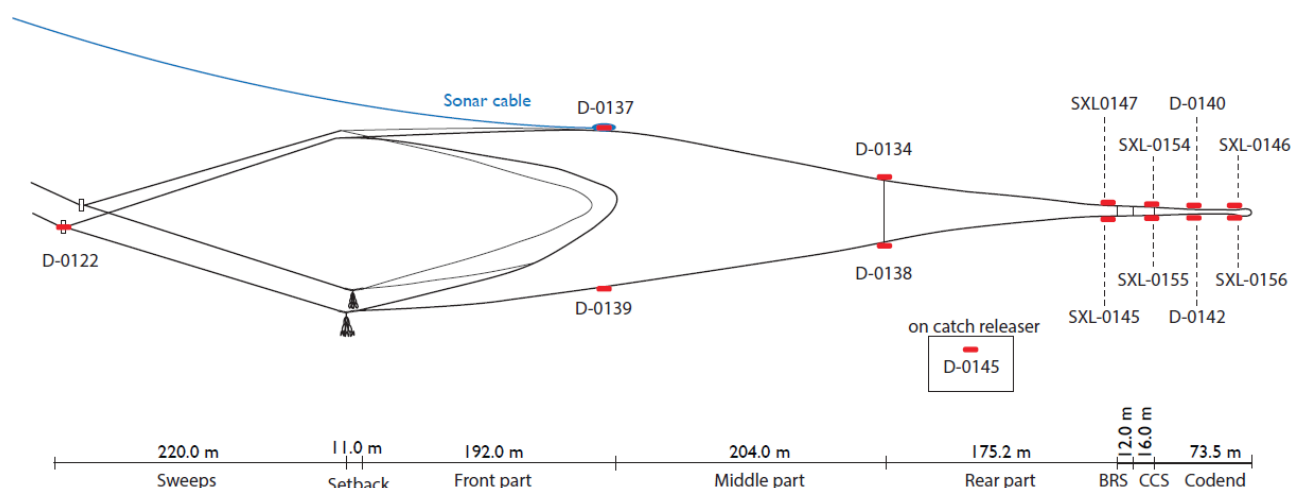
Figure 9.1 - Positions and Identity Code for depth sensors on the trawl. Detailed positions for the cod-end depth sensors are detailed in table 9.1. [Source: Liz Kvalvik].
