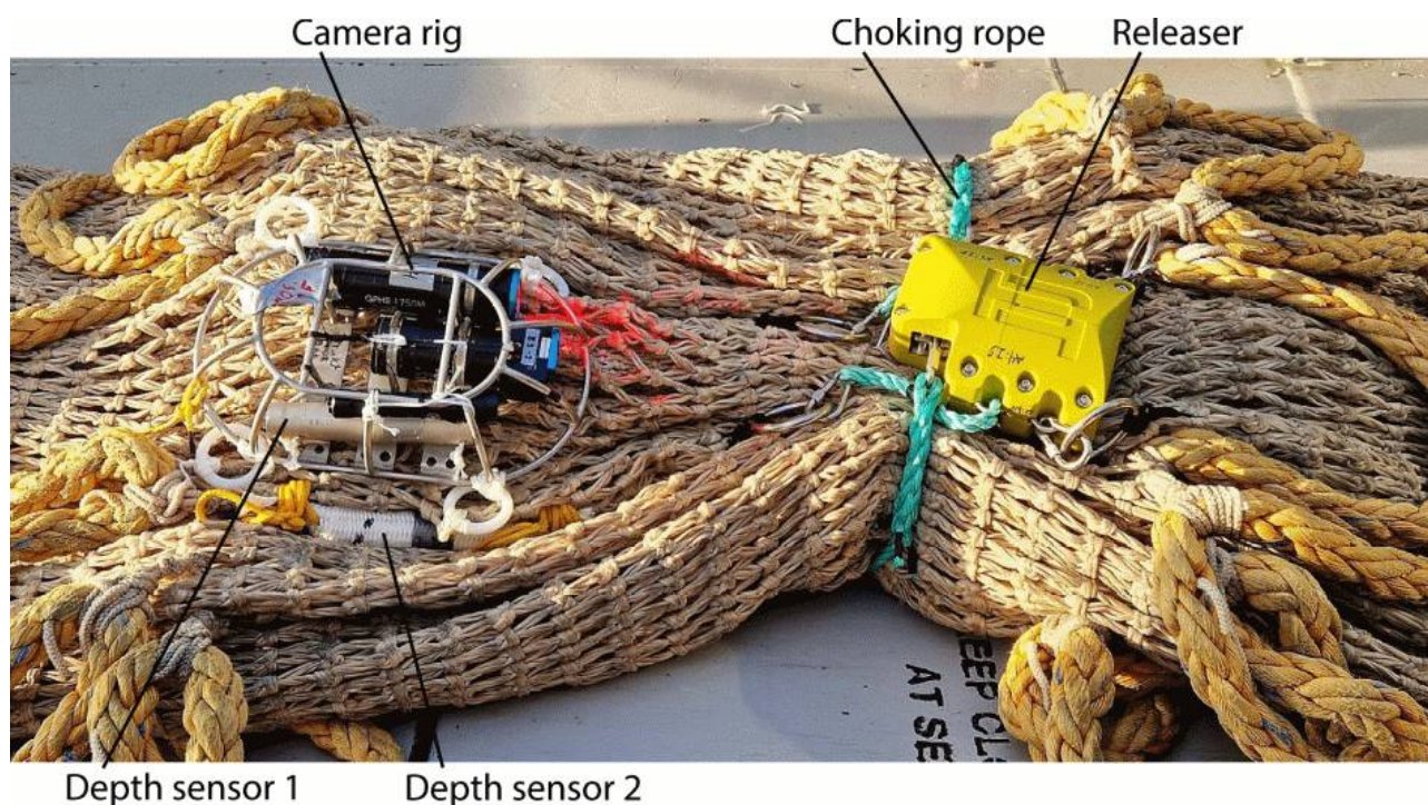
Figure 5.2: Haul A01, depth triggered cod-end choking unit (CCU) with a choking rope set at the 25m (~200t) position. Also shown is the camera and depth sensor assembly, in a protective steel frame, for monitoring the release depth of the CCU [Source: Ingolfsson et al, 2022].
