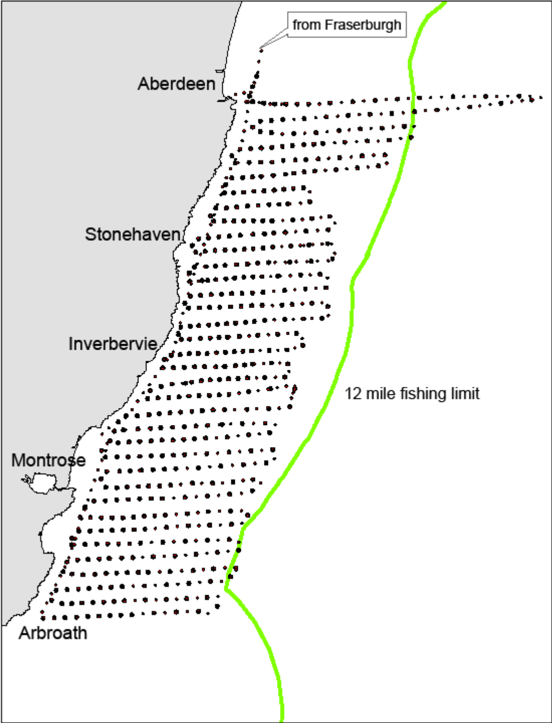
0308C cruise track and water sampling locations
