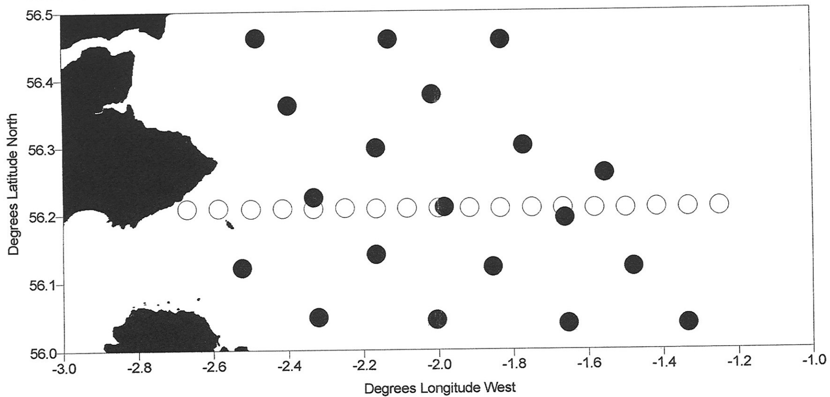
Fig 4. Chart showing CTD stations. Filled circles show main CTD grid, open circles show extra CTD transect.
