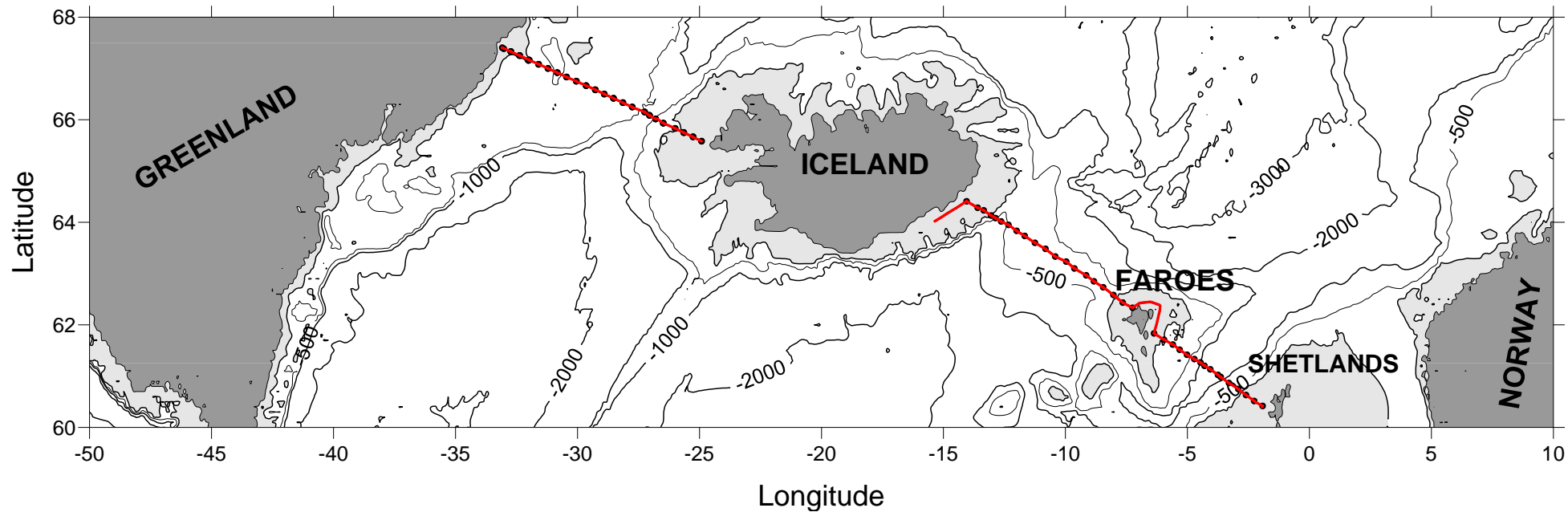
Fig. 1 Station locations (black circles) and ship track (in red). The shelf area with depth less than 200 m is shaded.
