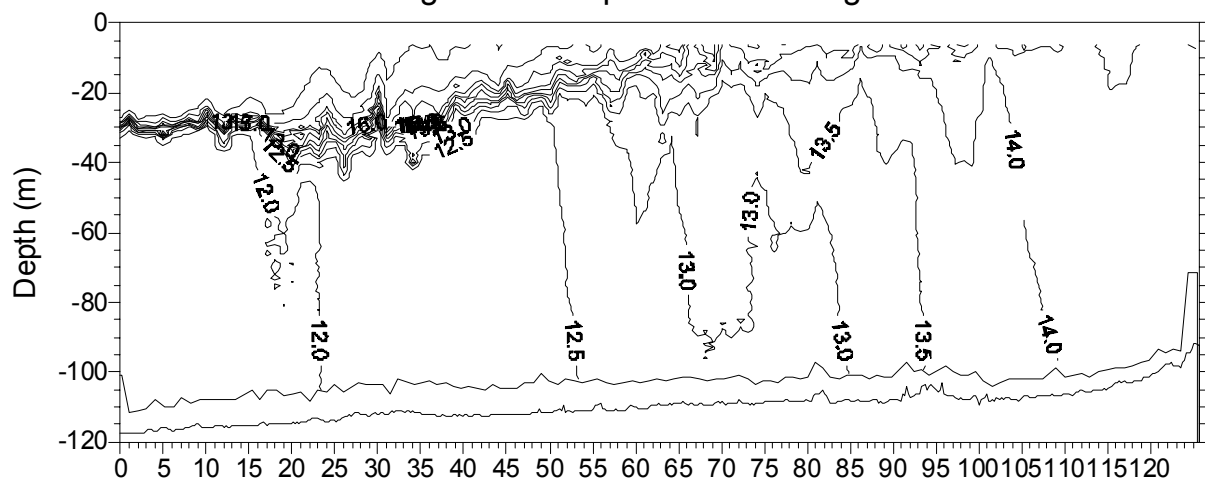
Density Sigma-t
