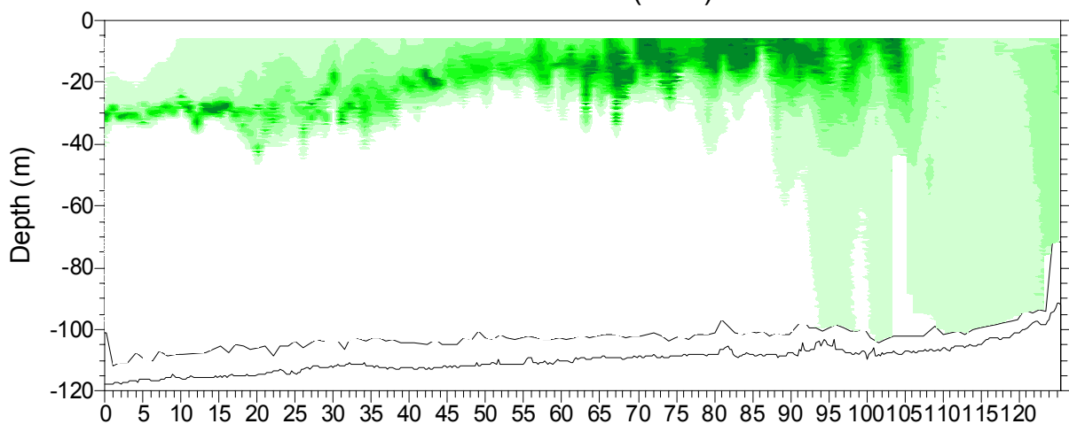
Fluorescence (volts)
