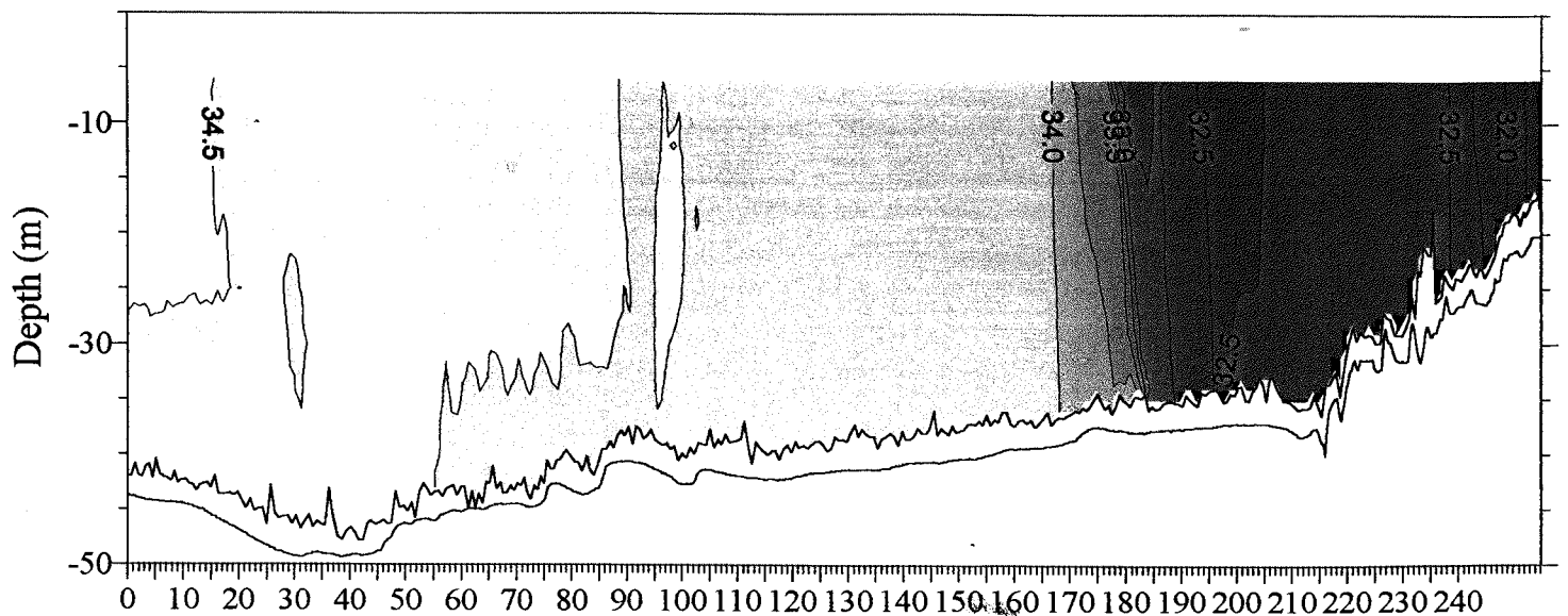
Salinity ppt Leg co08179
