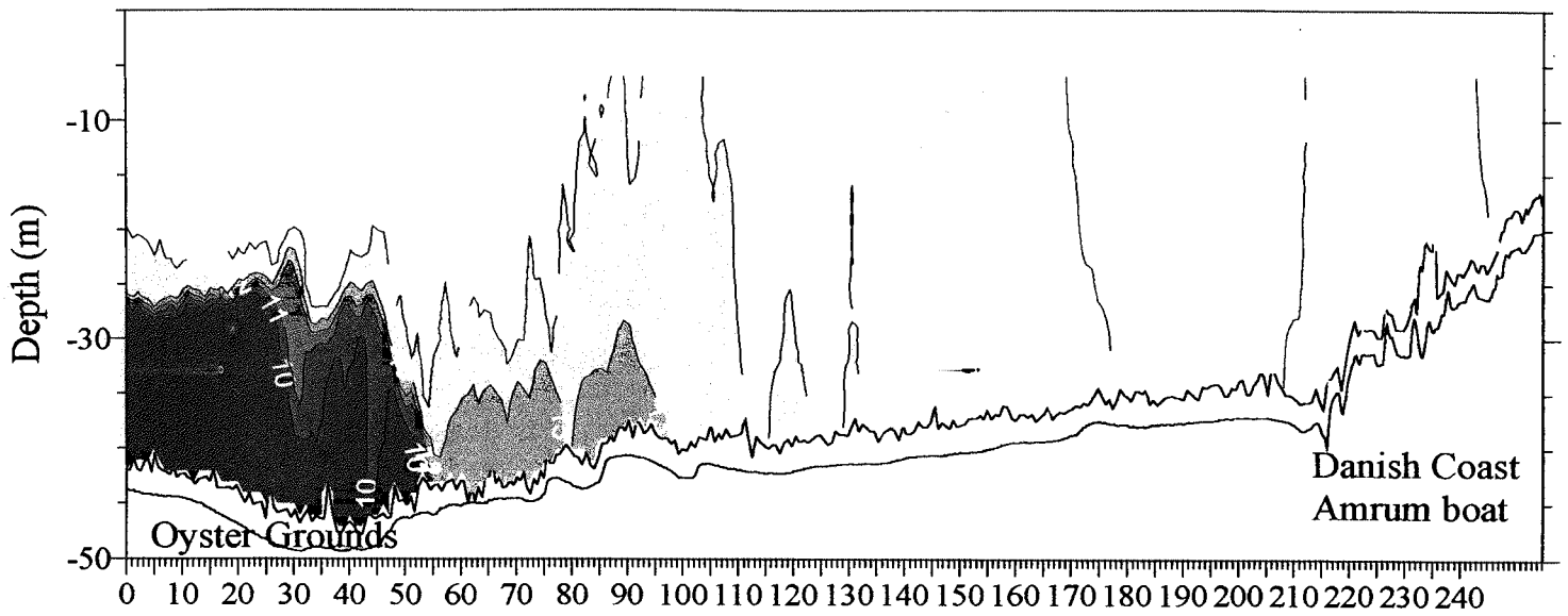
Density Sigma-t Leg co08179
