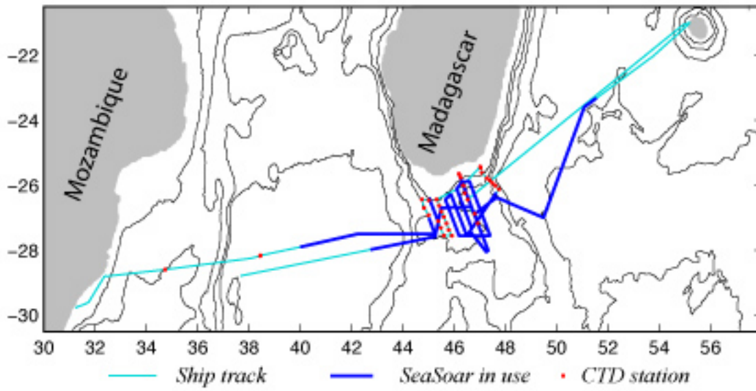
Cruise track of MadEx (D288) plus depth contours every 1000m
