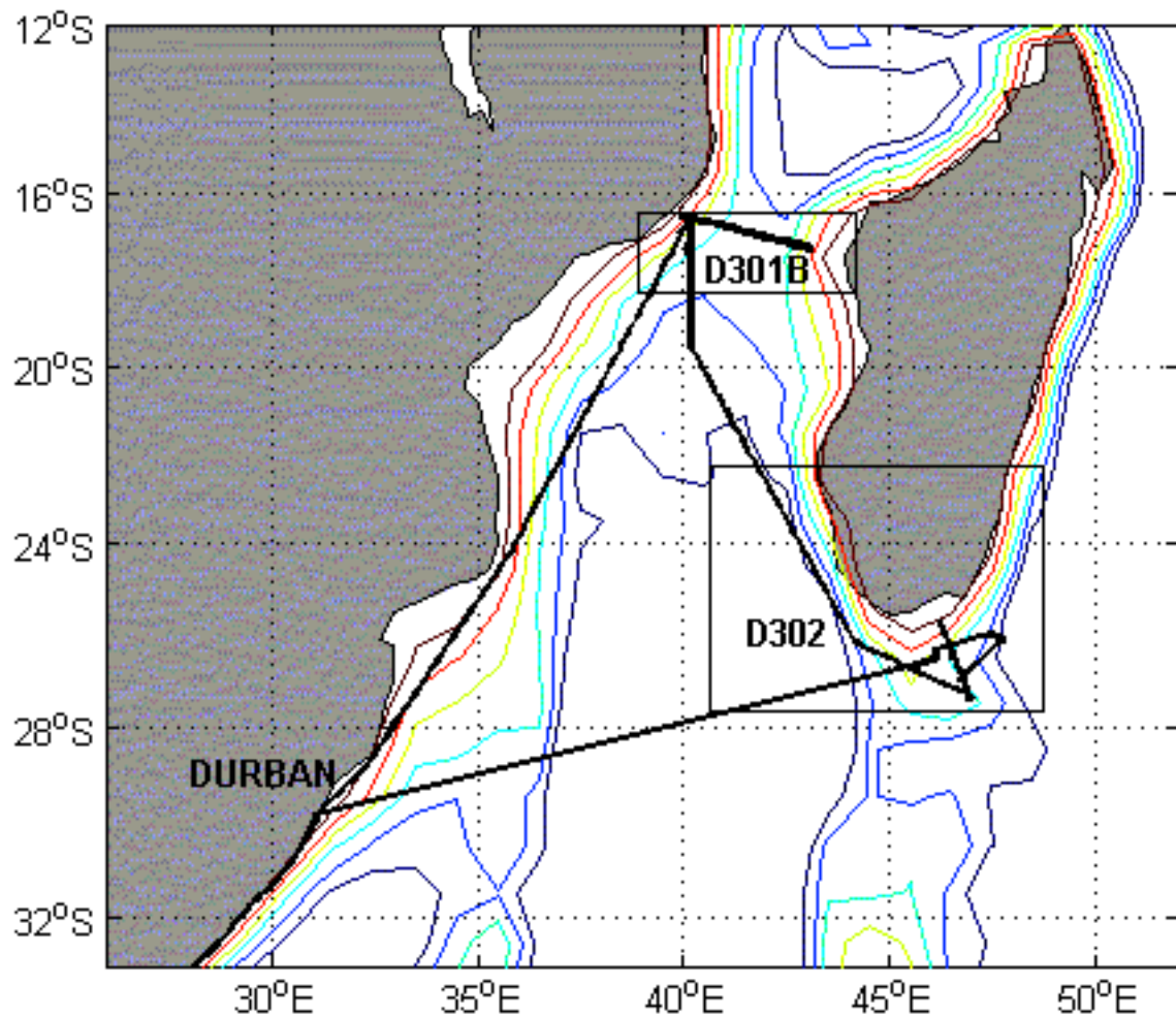
Figure 1. Cruise track of RRS Discovery cruise D301B-D302
