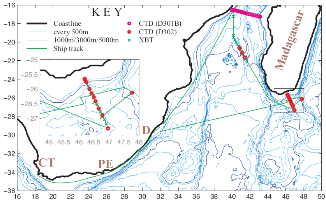
Bathymetry plot with ship track and CTD & XBT stations marked. [ Start was at Cape Town (CT) on day 075, with a port call at Durban (D) on day 079, then transit up western side of Mozambique Channel, down eastern side and back to Durban for a boat transfer, and finishing at Port Elizabeth (PE). ]
