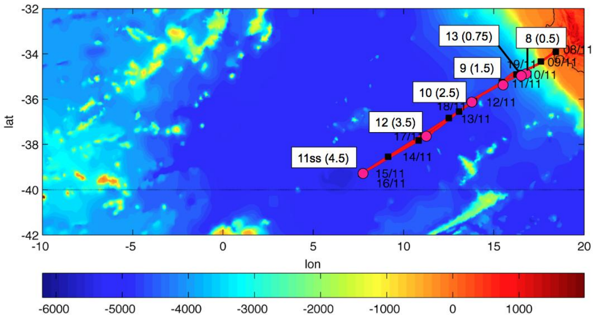
Figure 1: Cruise tracks for Leg 1 (upper) and Leg 2 (lower) superimposed on GEBCO bathymetry in metres. Dates are midnight start of day. Station locations and numbers are shown in white boxes.
