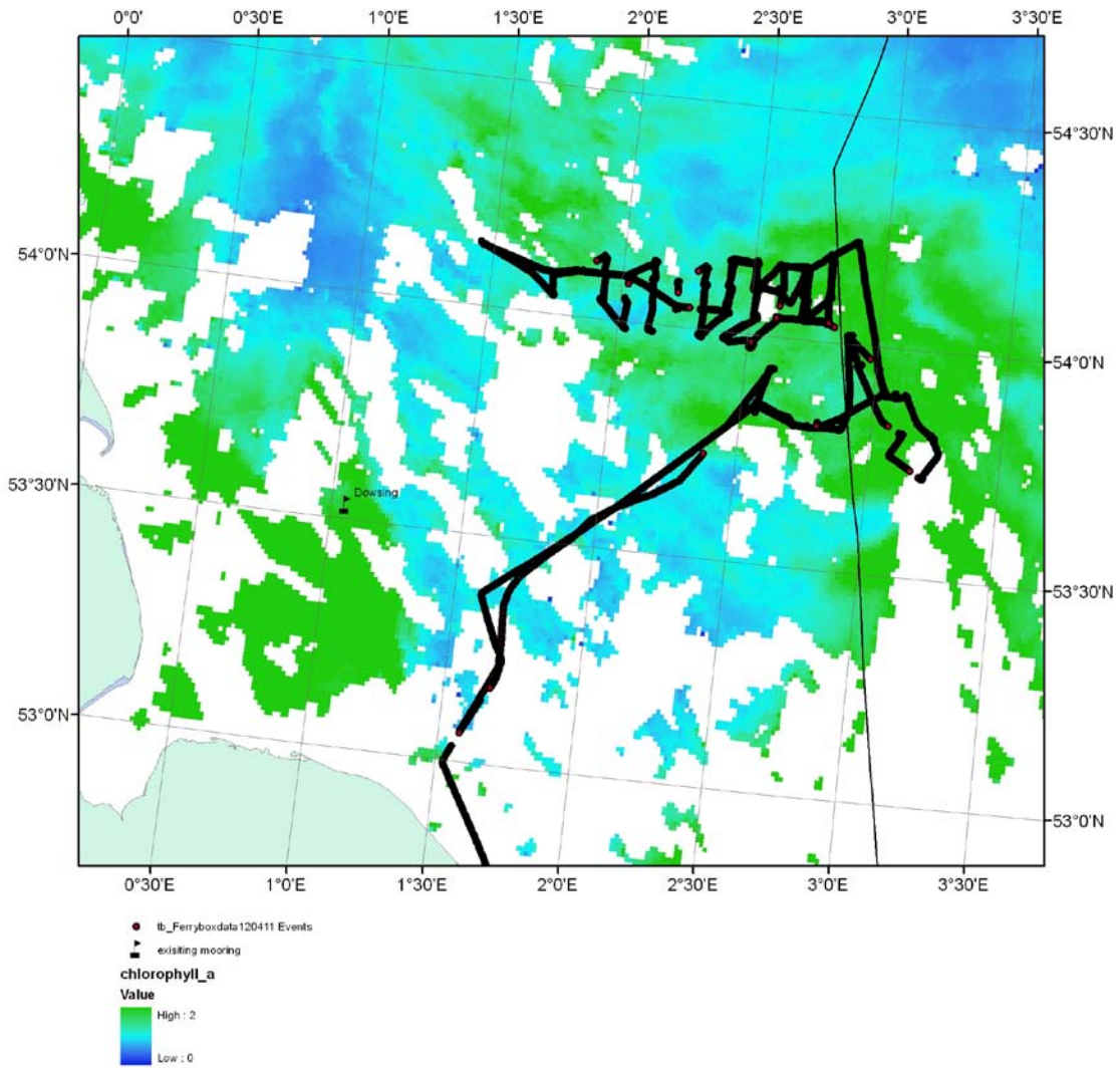
Overlay of cruise track from Ferrybox on an ocean colour image of the North Sea from Tuesday 10 th April, showing surface chlorophyll concentrations in the region.
