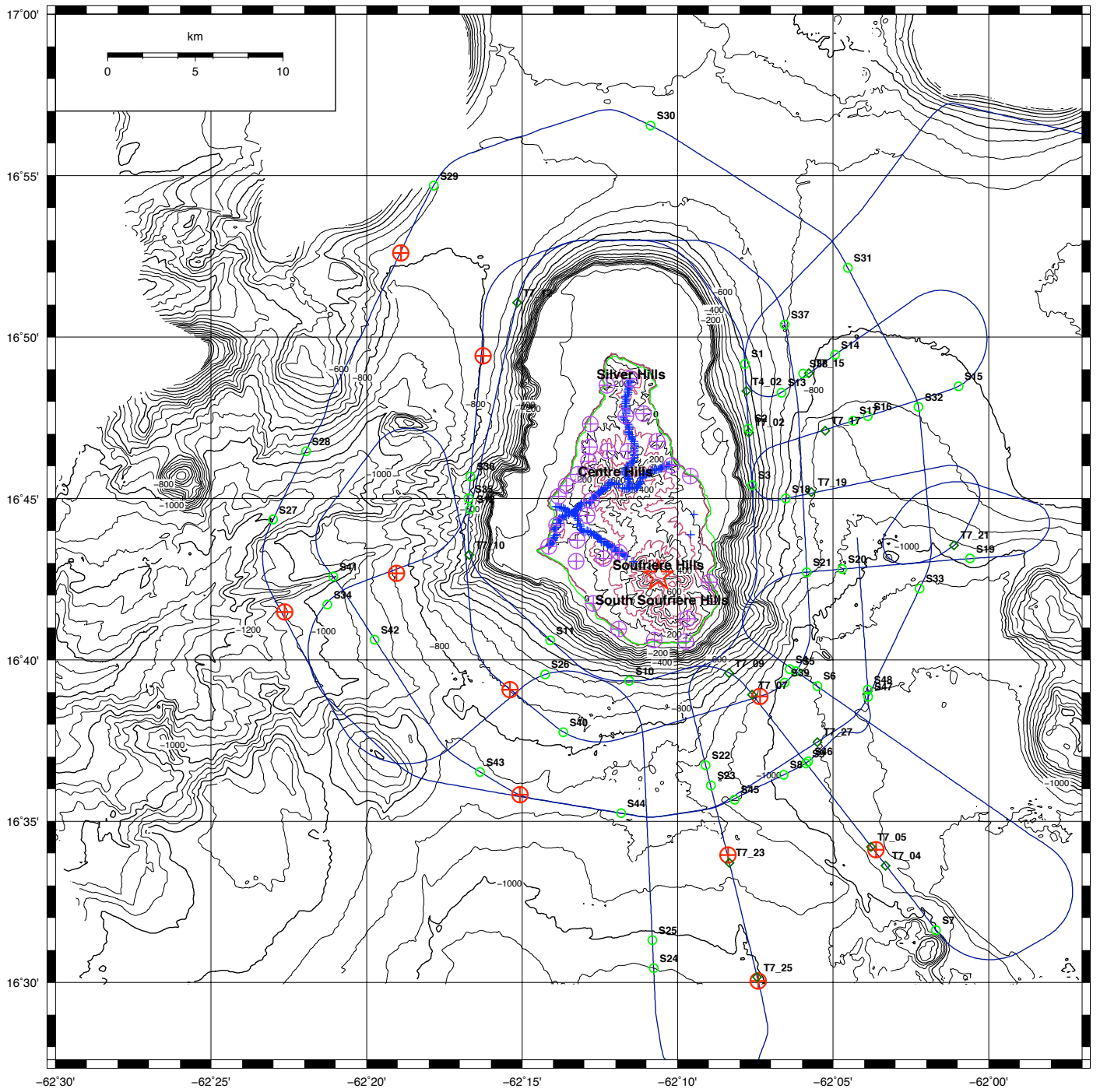
Figure 1: Track chart of JC19. OBSs = \oplus , refteks = \oplus , texans = + , sonobuoys = \circ , XBTs = \diamond
