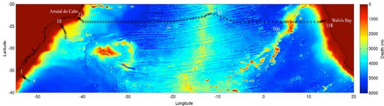
Figure 1: Bathymetric map of the JC032 study area and the positions of the stations sampled (*).
