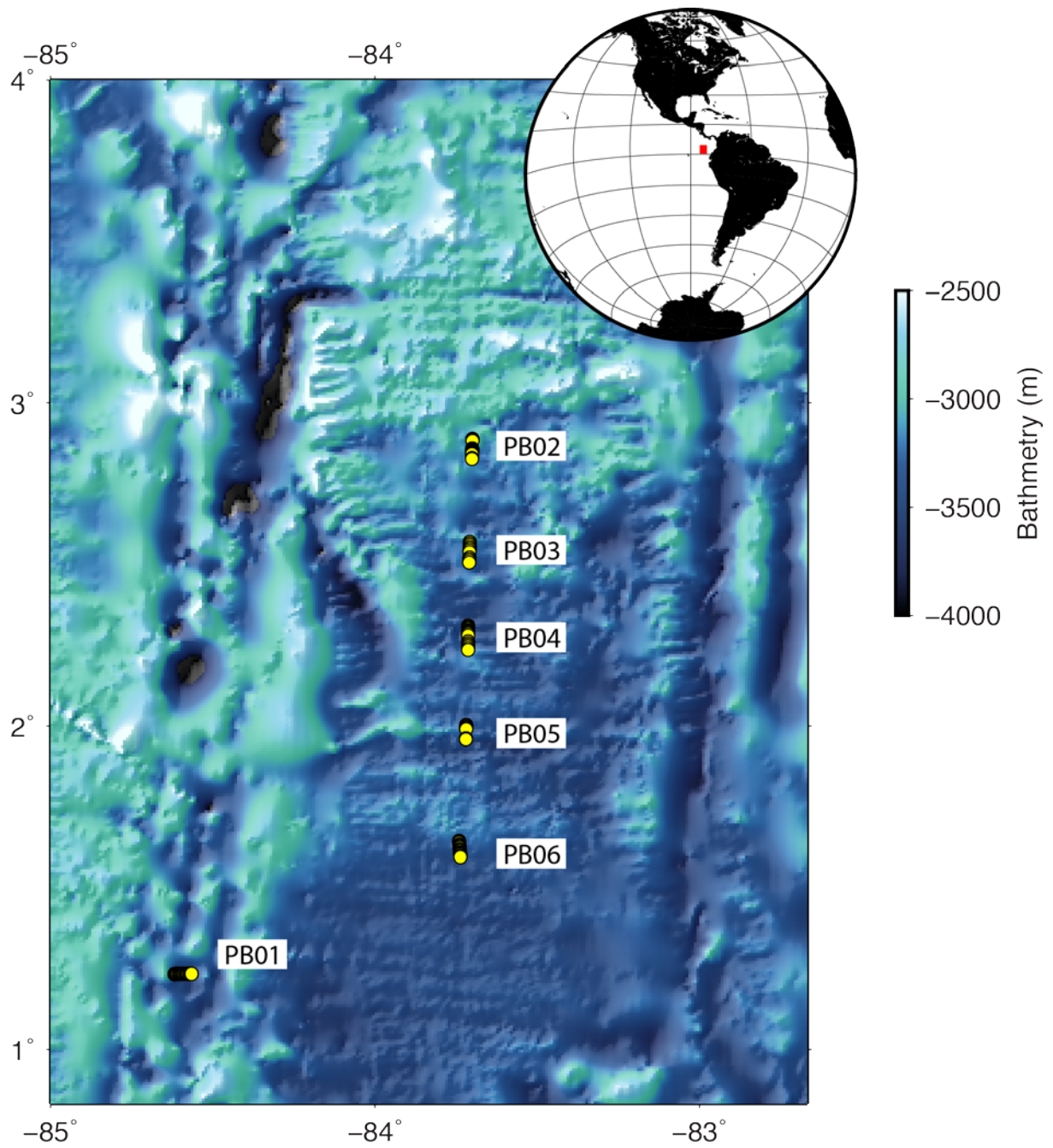
Figure 2. Position of heat flow measurements. Heat flow stations are labeled.
