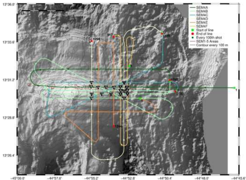
Map of the SEM4 survey covering the SEM4 and SEM3 deposits. Black inverted triangles represent the 18 OBXs deployed during the survey.
