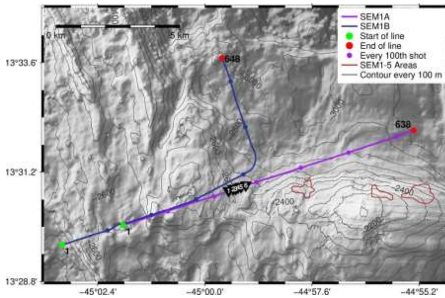
MAP of SEM1 GI-gun data acquisition. GI-gun data is acquired into two surveys: the planned SEM1A survey and the opportunistic SEM1B survey which completed the western part of the profile. The black triangles show the position of OBXs along SEM1.
