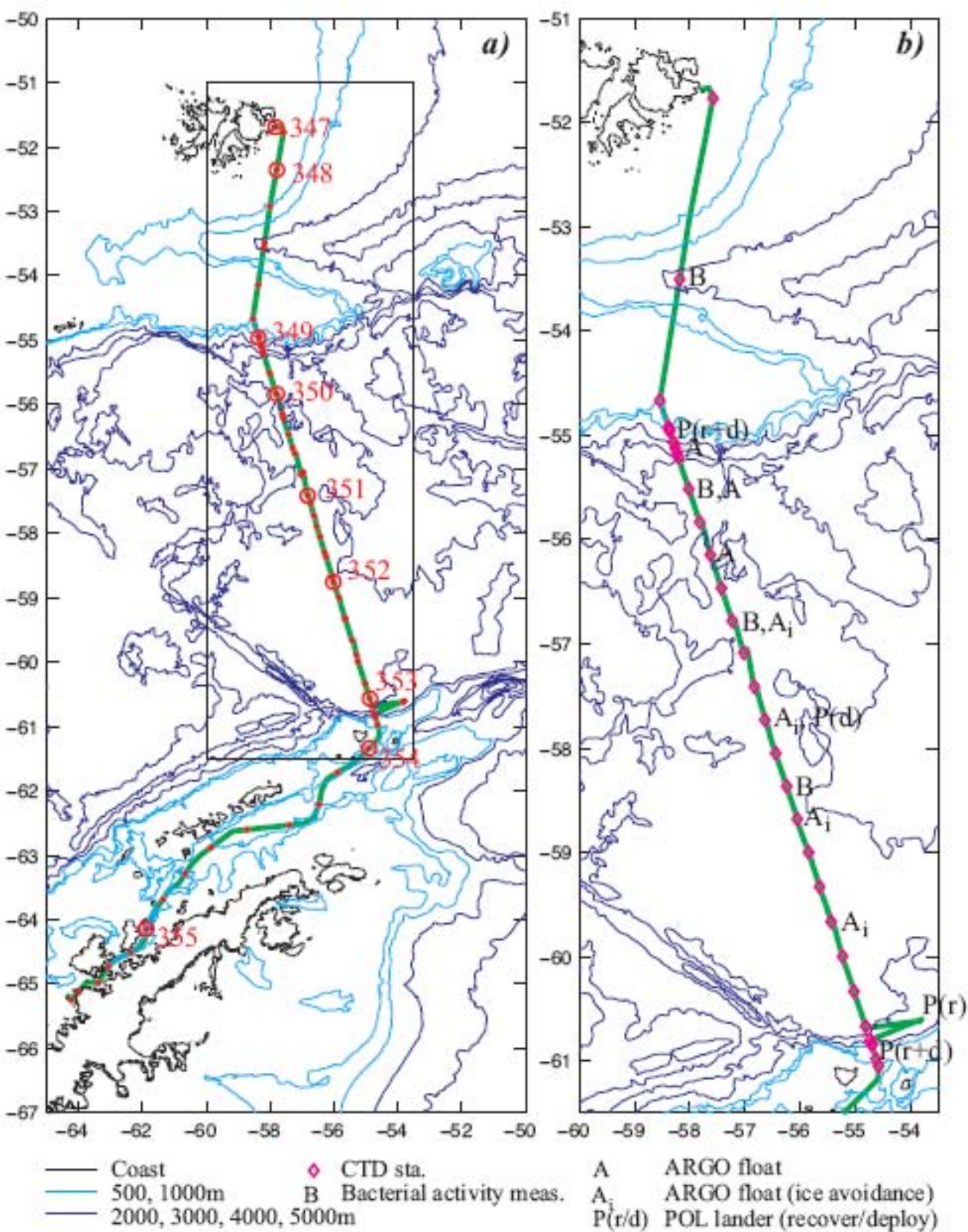
a) Overall cruise track, with small red dots every 3 hrs, b) CTD stations including stations where bacterial activity was estimated, plus ARGO deployments and POL's recovery/deployment work.
