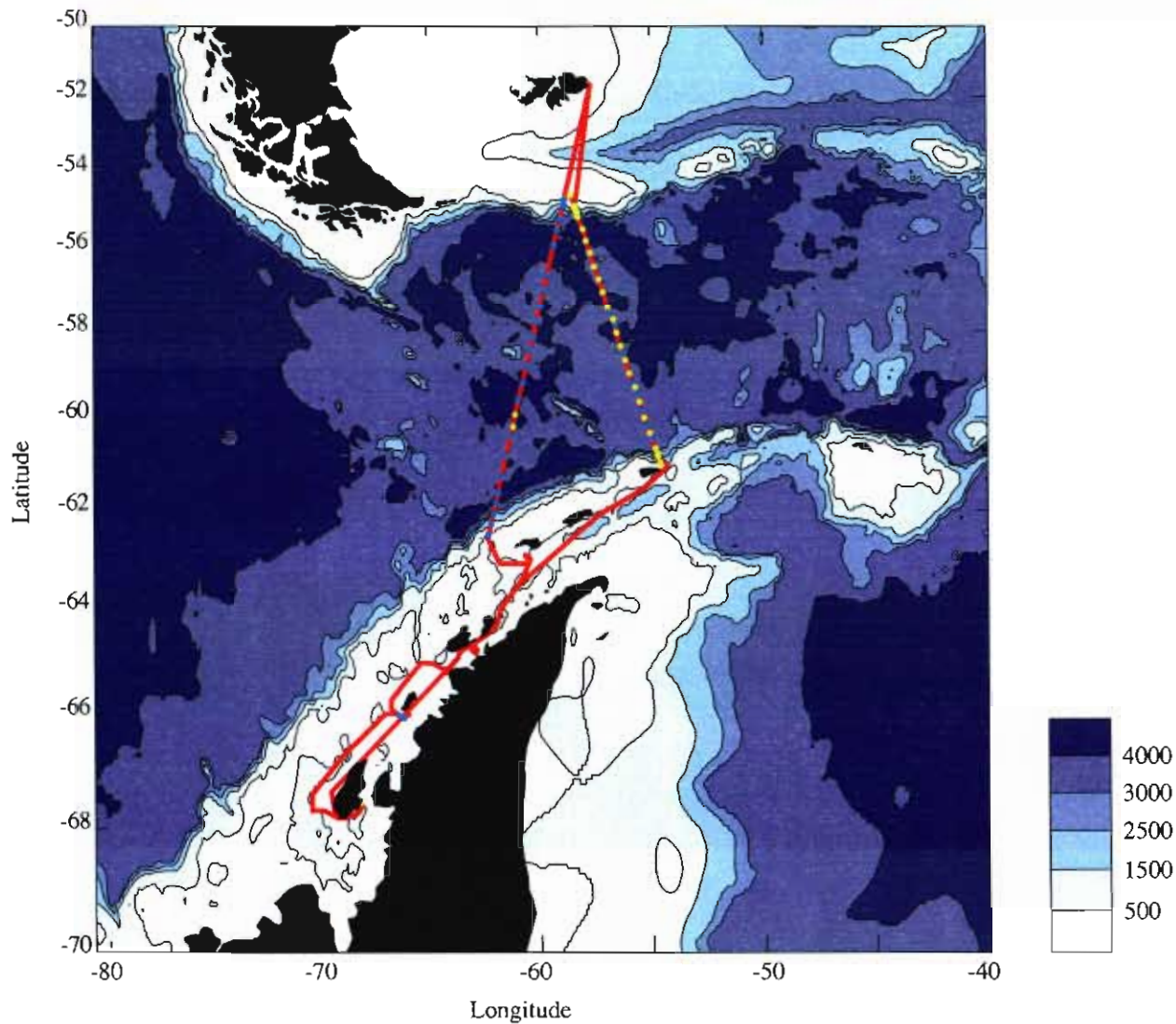
Figure 1. Cruise track for RRS James Clark Ross Cruise 55 (red line) showing CTD stations (yellow dots) and XBT stations (blue dots). Bathymetry is from the ddbb5 dataset.
