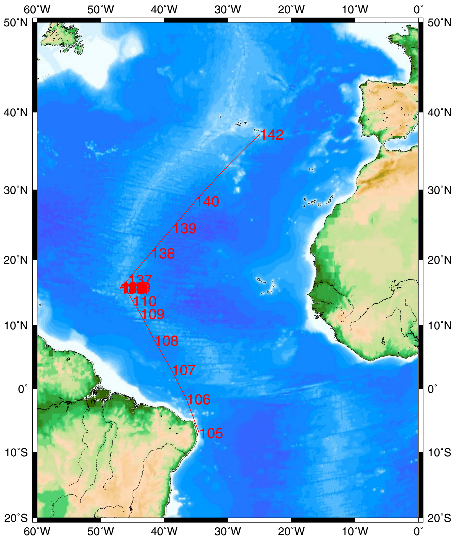
Figure 1: Shiptrack for JR63 over ETOPO5 bathymetry. Numbers correspond to Julian days.
