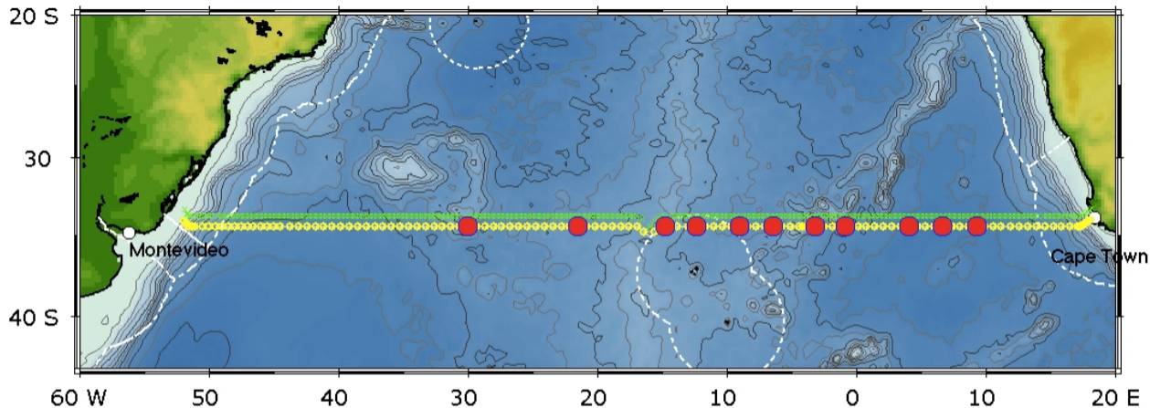
RV Maria S. Merian MSM60 cruise track from Cape Town to Montevideo. Yellow dots indicate CTD/IADCP/UVP casts, red circles indicate Argo float deployments, XBT data (green cross) are shown with an latitude offset.
