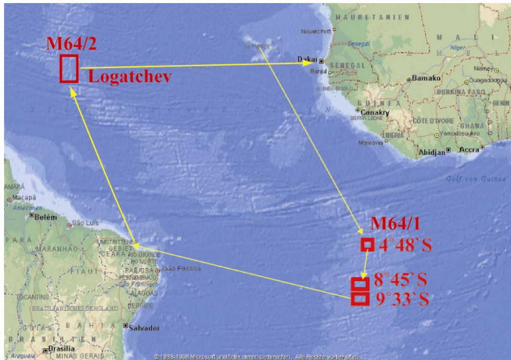
Fig. 1 Map of the central Atlantic Ocean showing the ports and working areas of the two M64 cruises.
