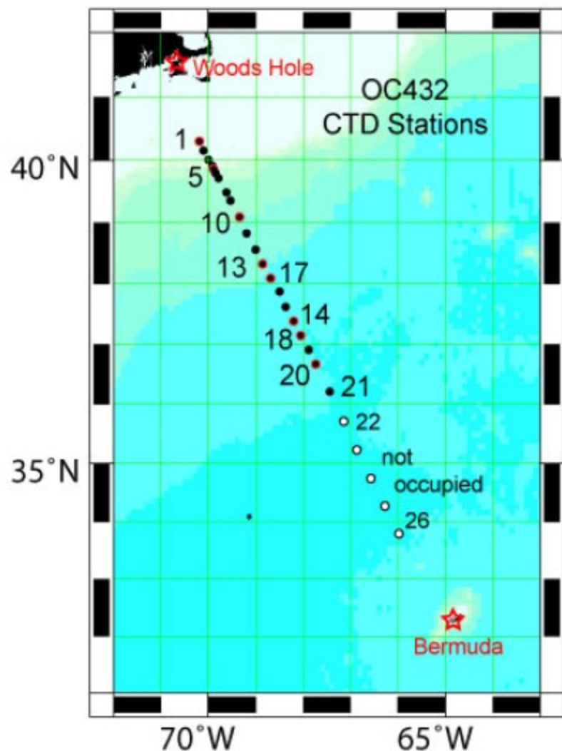
Figure 1. Left panel: locations of 21 CTD profiles acquired during OC432; background color depicts bathymetry. Right panel: cruise track overlain on sea surface temperature (source AVHRR, 6 days ending Oct 18).
