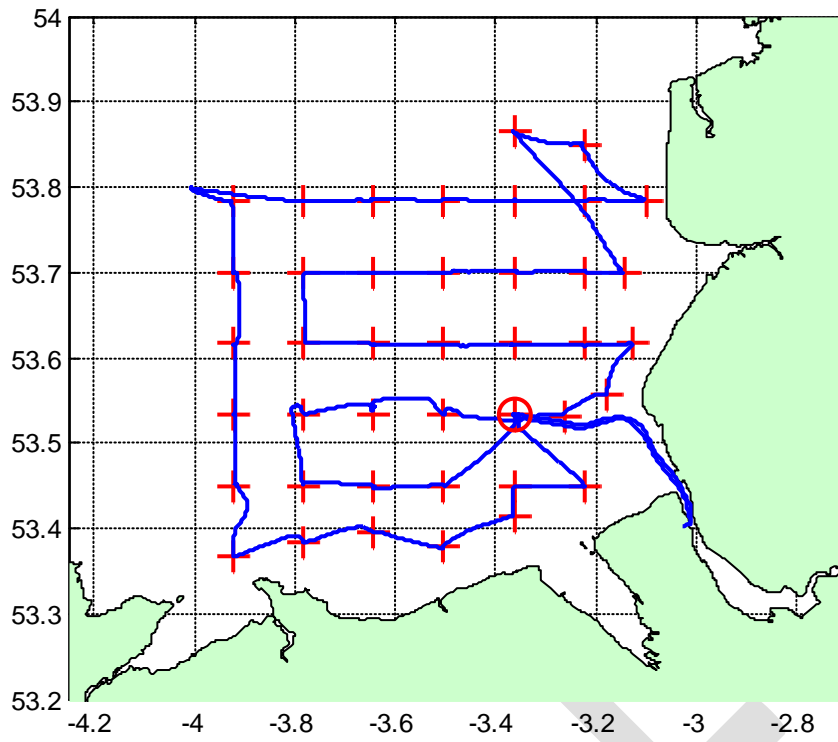
Figure 1. Irish Sea Observatory cruise 78 track. The nominal positions of the CTD stations are marked with red crosses and the main mooring site with an additional red circle.
