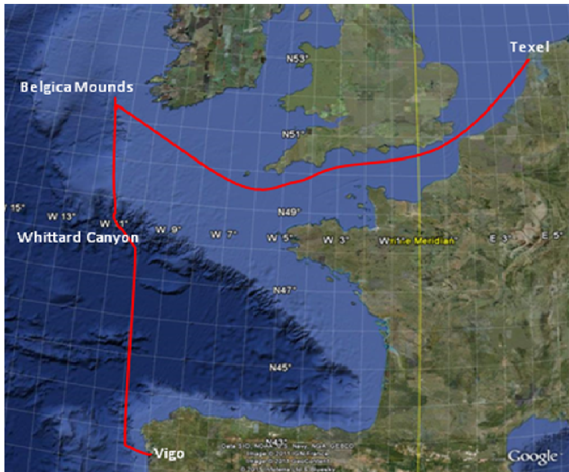
Fig. 1. Track of Cruise 64PE324 (11 Sept-2 Oct 2010).
