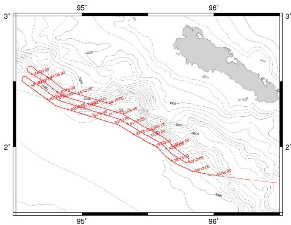
Figure 2. TOBI deep-towed sidescan sonar survey off Simeulue Island.
